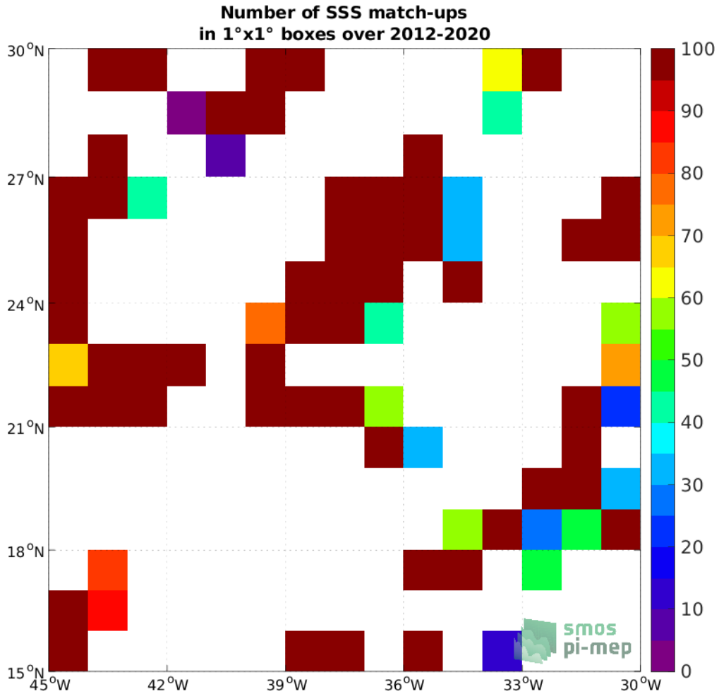
Figure 4: Number of SSS match-ups between TSG (GOSUD-Research-vessel) SSS and the SMOS SSS L2 v700 (ESA) SSS product for the SPURS 1 Pi-MEP region over 1^\circ \times 1^\circ boxes and for the full satellite product period.
