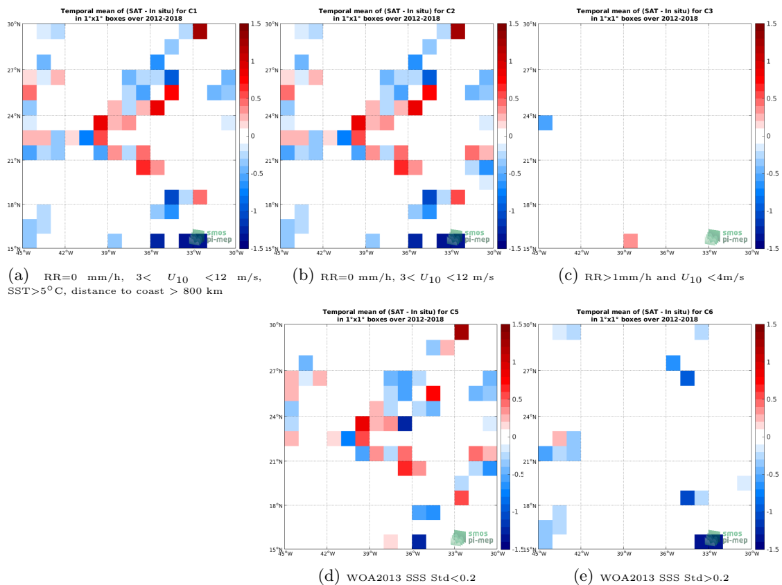
Figure 12: Temporal mean gridded over spatial boxes of size 1^\circ \times 1^\circ of \Delta\text{SSS} (SMOS SSS L2 v700 (ESA) - TSG (GOSUD-Research-vessel)) for 5 different subdatasets corresponding to:RR=0 mm/h, 3 < U_{10} < 12 m/s, SST>5°C, distance to coast > 800 km (a), RR=0 mm/h, 3 < U_{10} < 12 m/s (b), RR>1mm/h and U_{10} < 4 m/s (c), WOA2013 SSS Std<0.2 (d), WOA2013 SSS Std>0.2 (e).
