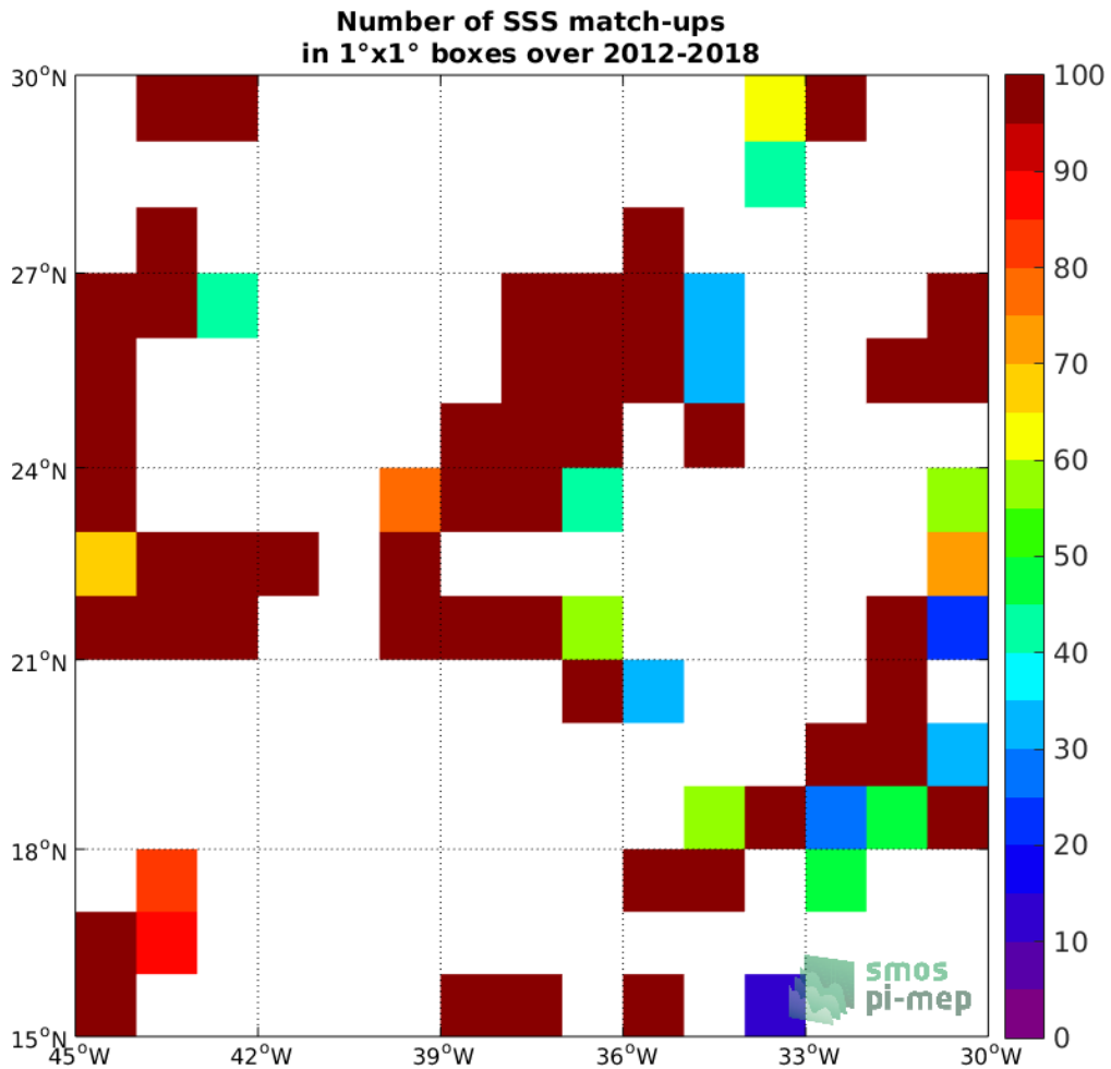
Figure 4: Number of SSS match-ups between TSG (GOSUD-Research-vessel) SSS and the SMOS SSS L2 v700 (ESA) SSS product for the SPURS 1 Pi-MEP region over 1°x1° boxes and for the full satellite product period.
