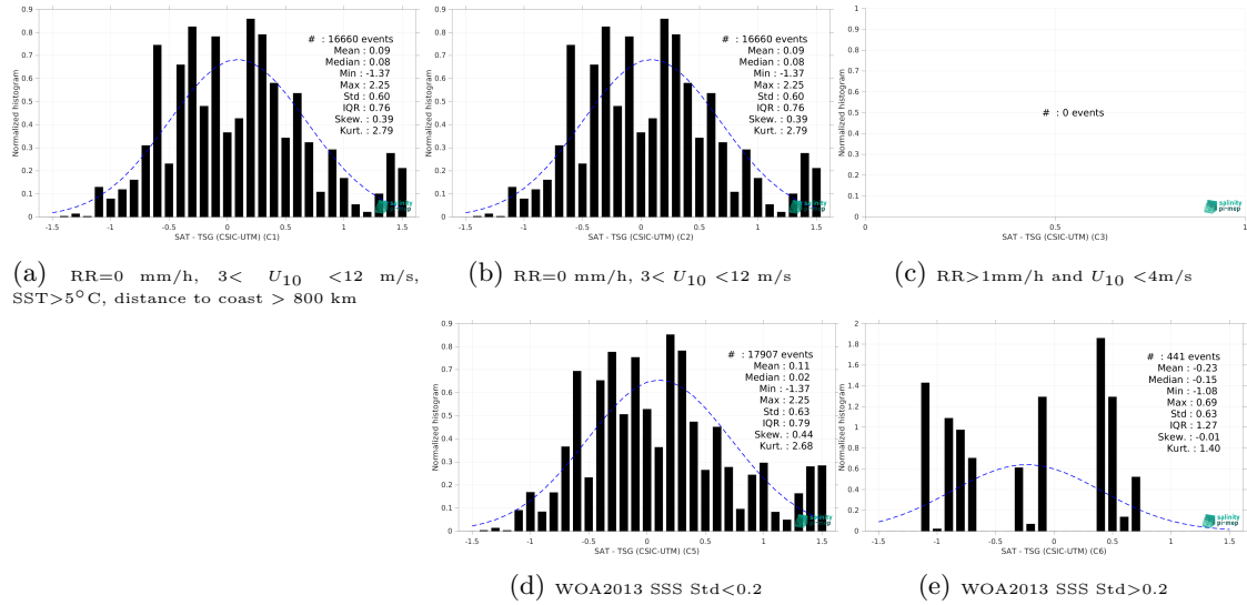
Figure 15: Normalized histogram of \Delta SSS (SMOS SSS L2 v700 (ESA) - TSG (CSIC-UTM)) for 5 different subdatasets corresponding to: RR=0 mm/h, 3 < U_{10} < 12 m/s, SST > 5°C, distance to coast > 800 km (a), RR=0 mm/h, 3 < U_{10} < 12 m/s (b), RR > 1mm/h and U_{10} < 4 m/s (c), WOA2013 SSS Std < 0.2 (d), WOA2013 SSS Std > 0.2 (e).
