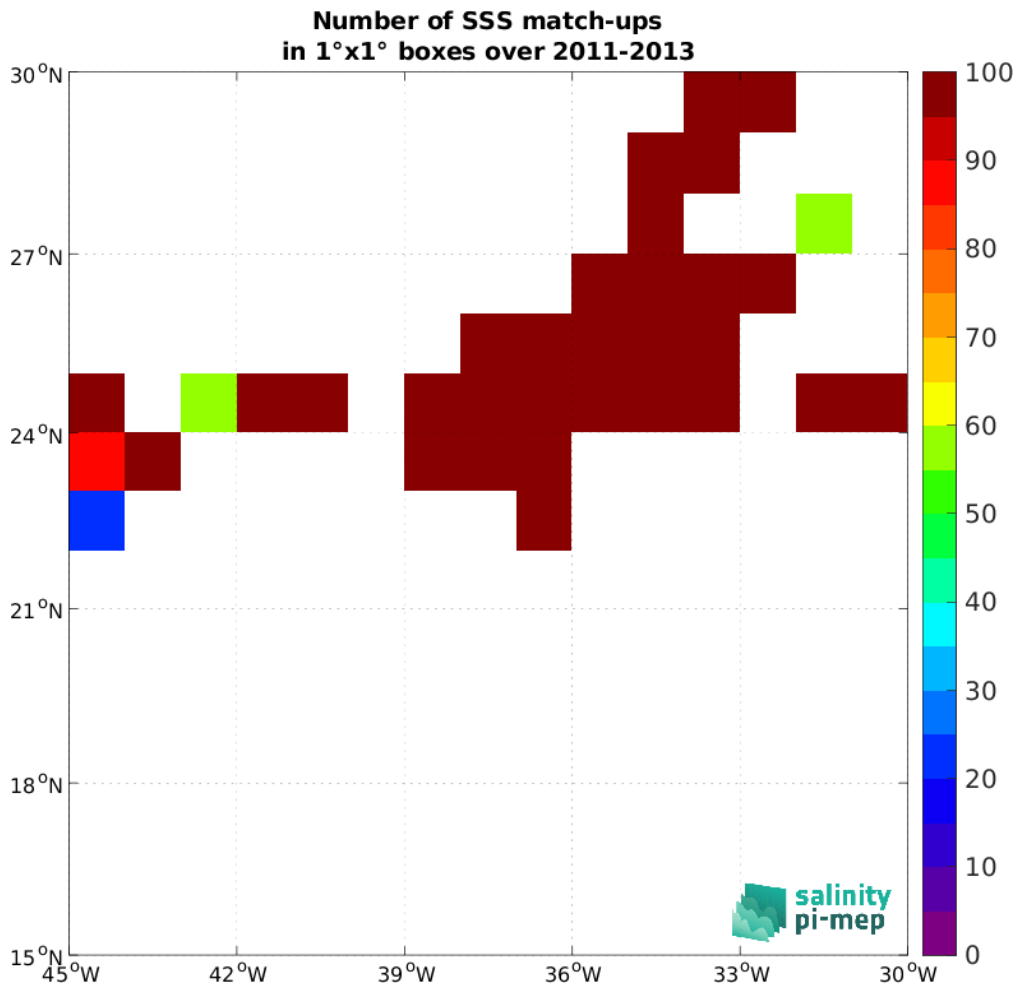
Figure 5: Number of SSS match-ups between TSG (CSIC-UTM) SSS and the SMOS SSS L2 v700 (ESA) SSS product for the SPURS 1 Pi-MEP region over 1°x1° boxes and for the full satellite product period.
