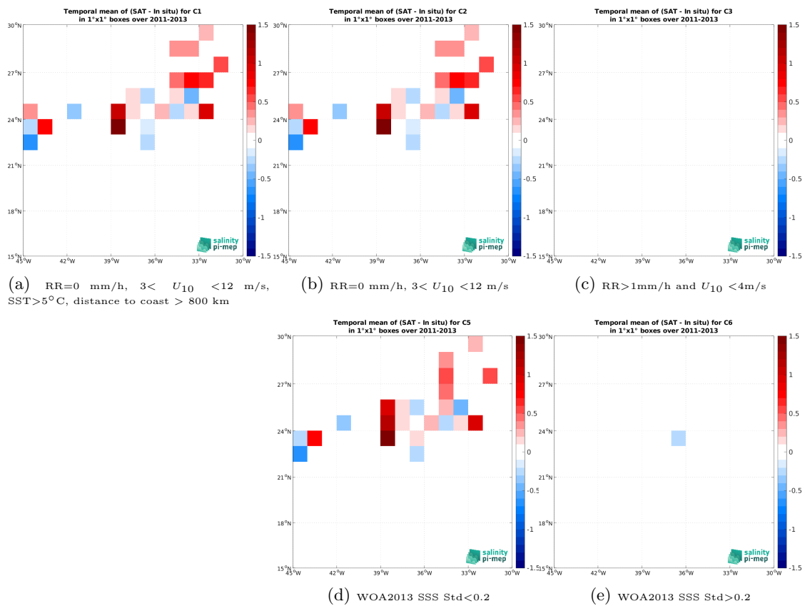
Figure 14: Temporal mean gridded over spatial boxes of size 1^\circ \times 1^\circ of \Delta SSS (SMOS SSS L2 v700 (ESA) - TSG (CSIC-UTM)) for 5 different subdatasets corresponding to:RR=0 mm/h, 3 < U_{10} < 12 m/s, SST>5°C, distance to coast > 800 km (a), RR=0 mm/h, 3 < U_{10} < 12 m/s (b), RR>1mm/h and U_{10} < 4 m/s (c), WOA2013 SSS Std<0.2 (d), WOA2013 SSS Std>0.2 (e).
