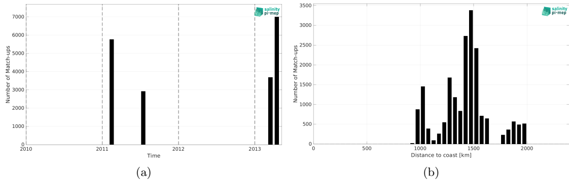
Figure 2: Number of match-ups between TSG (CSIC-UTM) and SMOS SSS L2 v700 (ESA) SSS as a function of time (a) and as function of the distance to coast (b) over the SPURS 1 Pi-MEP region and for the full satellite product period.
