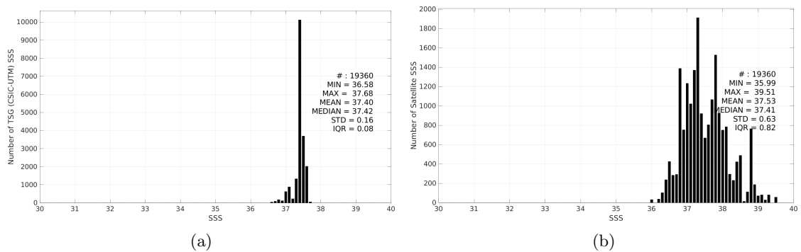
Figure 3: Histograms of SSS from TSG (CSIC-UTM) (a) and SMOS SSS L2 v700 (ESA) (b) considering all match-up pairs per bins of 0.1 over the SPURS 1 Pi-MEP region and for the full satellite product period.
