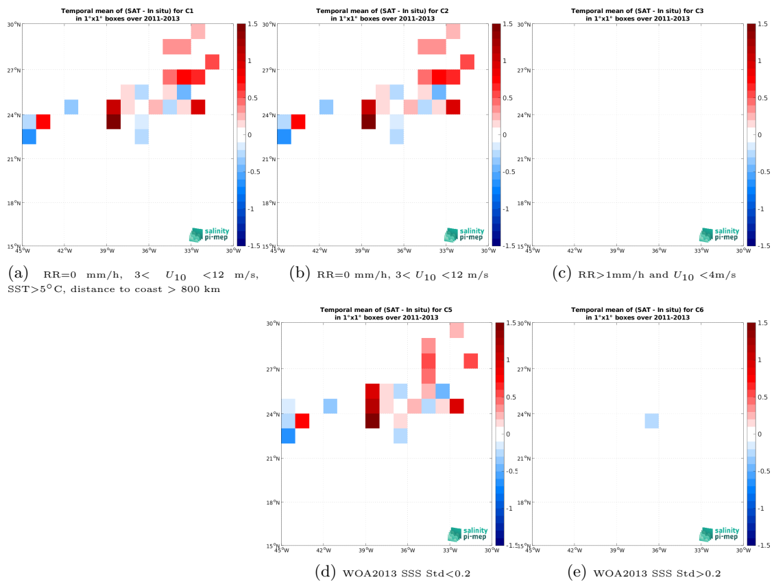
Figure 14: Temporal mean gridded over spatial boxes of size 1^\circ \times 1^\circ of \Delta SSS (SMOS SSS L2 v700 (ESA) - TSG (CSIC-UTM)) for 5 different subdatasets corresponding to: RR=0 mm/h, 3 < U_{10} < 12 m/s, SST > 5^\circ C , distance to coast > 800 km (a), RR=0 mm/h, 3 < U_{10} < 12 m/s (b), RR > 1 mm/h and U_{10} < 4 m/s (c), WOA2013 SSS Std < 0.2 (d), WOA2013 SSS Std > 0.2 (e).
