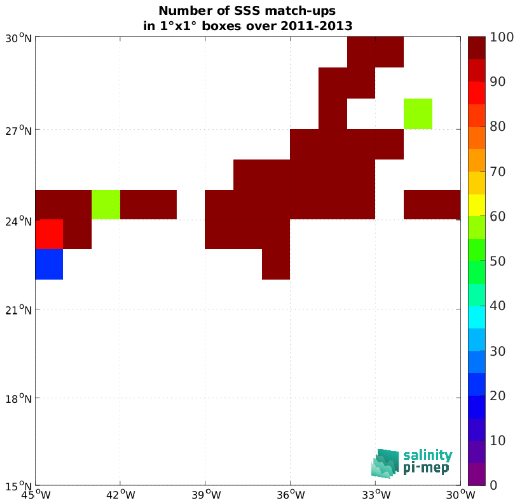
Figure 5: Number of SSS match-ups between TSG (CSIC-UTM) SSS and the SMOS SSS L2 v700 (ESA) SSS product for the SPURS 1 Pi-MEP region over 1^\circ \times 1^\circ boxes and for the full satellite product period.
