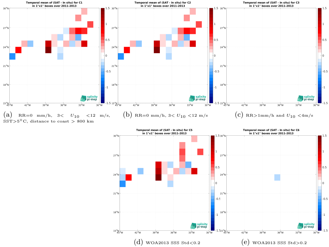
Figure 12: Temporal mean gridded over spatial boxes of size 1^{\circ}\times 1^{\circ} of \Delta\text{SSS} (SMOS SSS L2 v700 (ESA) - TSG (CSIC-UTM)) for 5 different subdatasets corresponding to:RR=0 mm/h, 3 < U_{10} < 12 m/s, SST >5^{\circ}\text{C} , distance to coast > 800 km (a), RR=0 mm/h, 3 < U_{10} < 12 m/s (b), RR >1 mm/h and U_{10} < 4 m/s (c), WOA2013 SSS Std <0.2 (d), WOA2013 SSS Std >0.2 (e).
