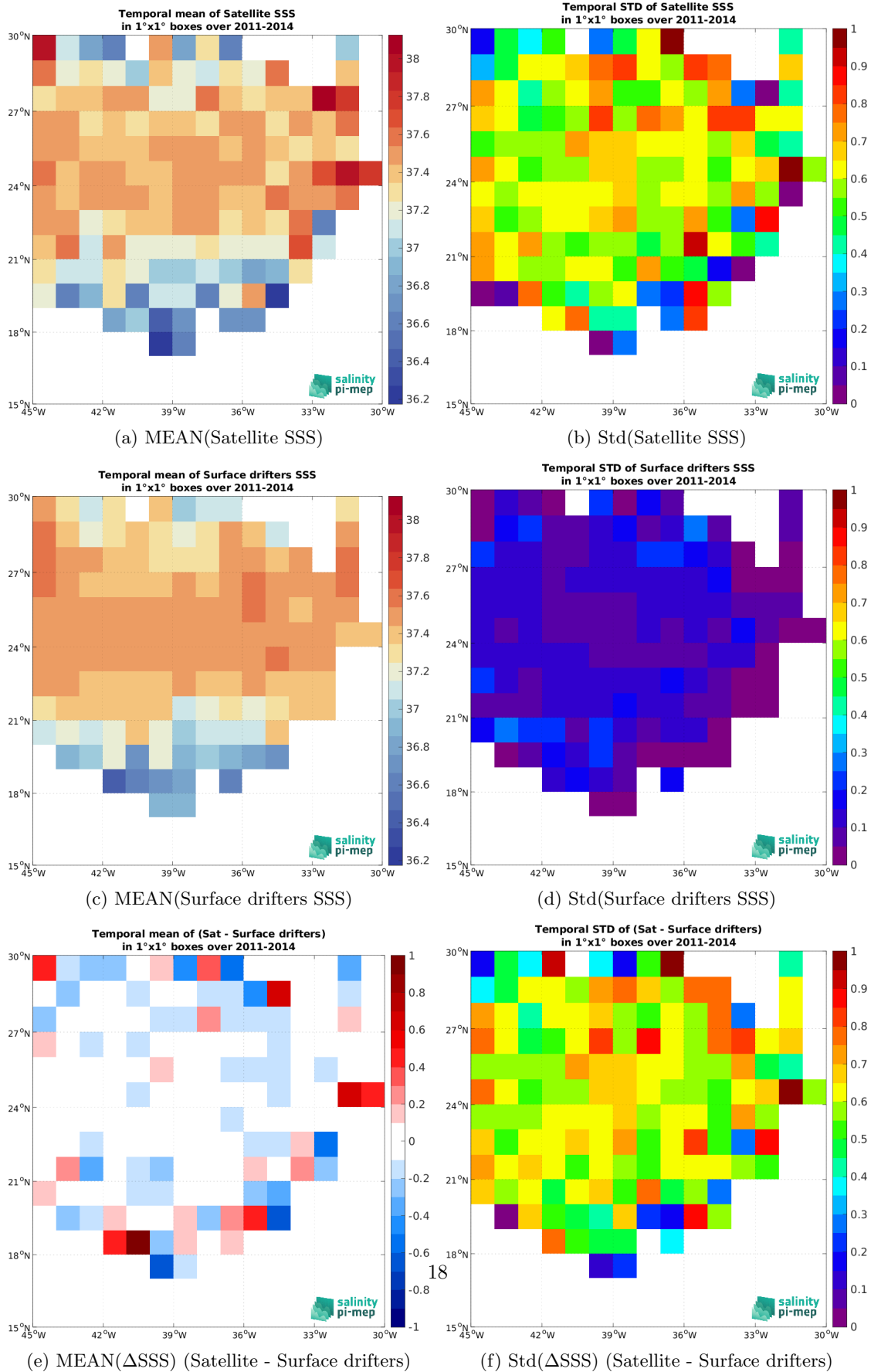
Figure 6: Temporal mean (left) and Std (right) of SSS from SMOS SSS L2 v700 (ESA) (top), Surface drifters (middle), and of \Delta SSS (Satellite - Surface drifters). Only match-up pairs are used to generate these maps.
