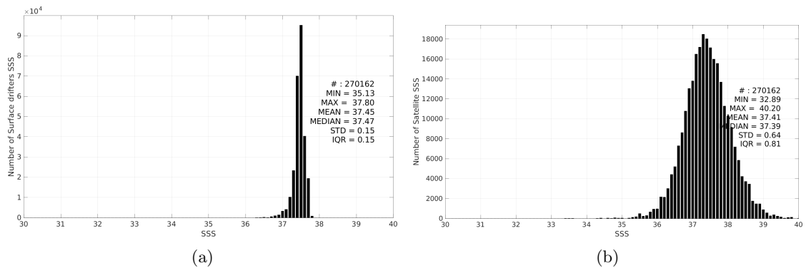
Figure 3: Histograms of SSS from Surface drifters (a) and SMOS SSS L2 v700 (ESA) (b) considering all match-up pairs per bins of 0.1 over the SPURS 1 Pi-MEP region and for the full satellite product period.
