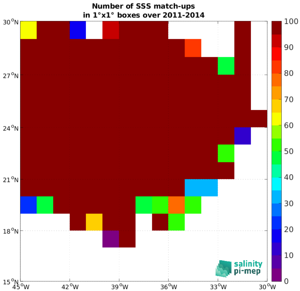
Figure 4: Number of SSS match-ups between Surface drifters SSS and the SMOS SSS L2 v700 (ESA) SSS product for the SPURS 1 Pi-MEP region over 1^\circ \times 1^\circ boxes and for the full satellite product period.
