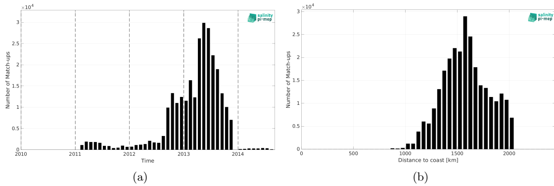
Figure 2: Number of match-ups between Surface drifters and SMOS SSS L2 v700 (ESA) SSS as a function of time (a) and as function of the distance to coast (b) over the SPURS 1 Pi-MEP region and for the full satellite product period.
