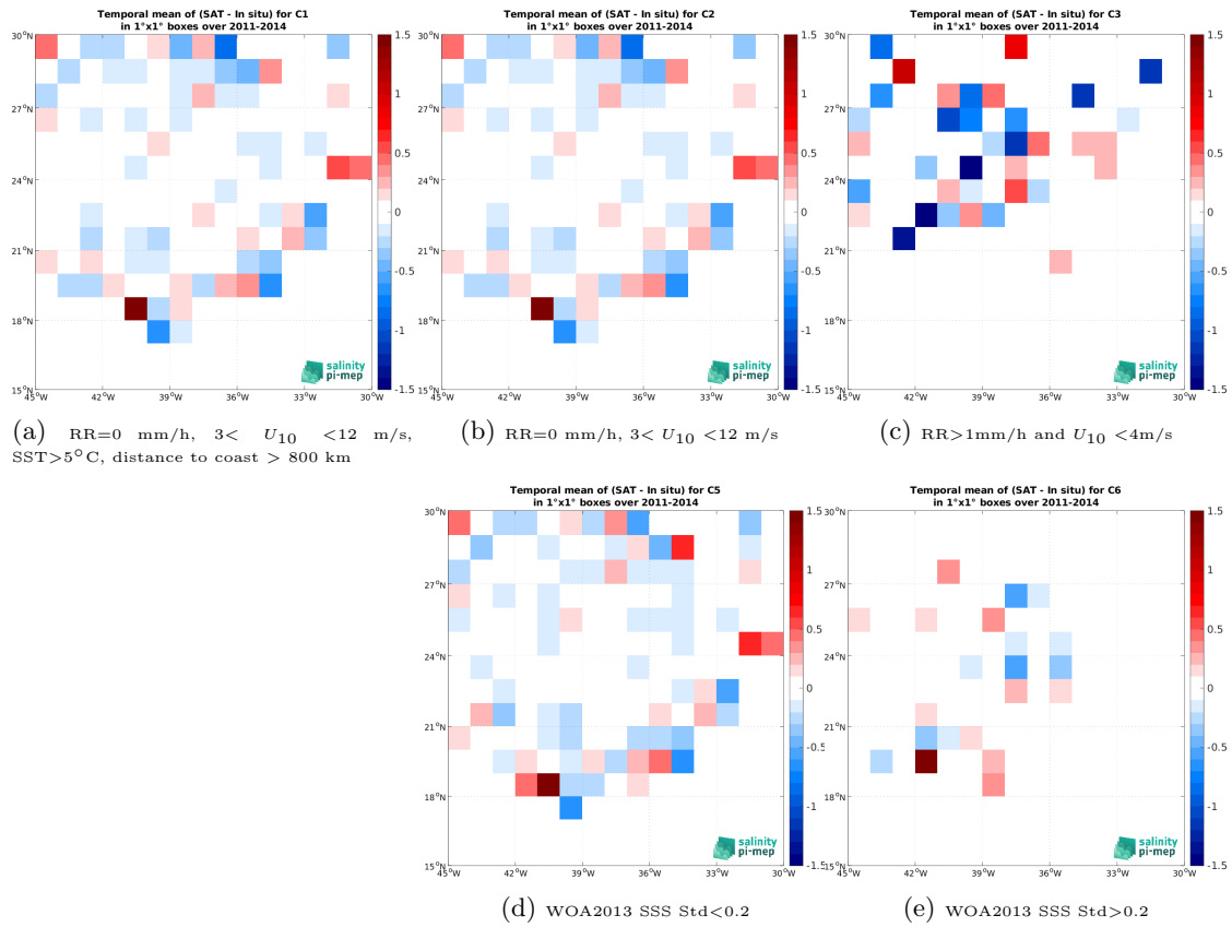
Figure 13: Temporal mean gridded over spatial boxes of size 1^\circ \times 1^\circ of \Delta SSS (SMOS SSS L2 v700 (ESA) - Surface drifters) for 5 different subdatasets corresponding to: RR=0 mm/h, 3 < U_{10} < 12 m/s, SST > 5^\circ C , distance to coast > 800 km (a), RR=0 mm/h, 3 < U_{10} < 12 m/s (b), RR > 1 mm/h and U_{10} < 4 m/s (c), WOA2013 SSS Std < 0.2 (d), WOA2013 SSS Std > 0.2 (e).
