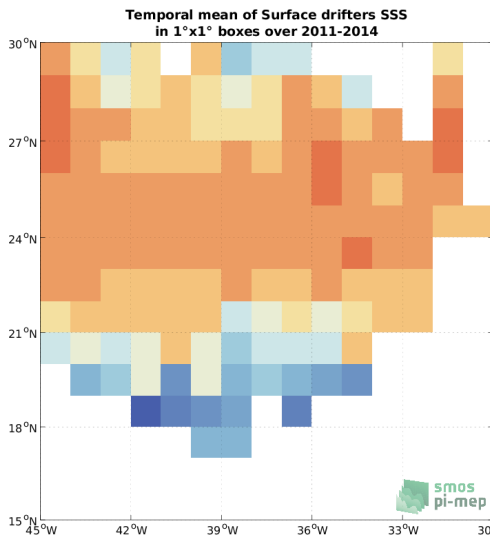
(c) MEAN(Surface drifters SSS)
