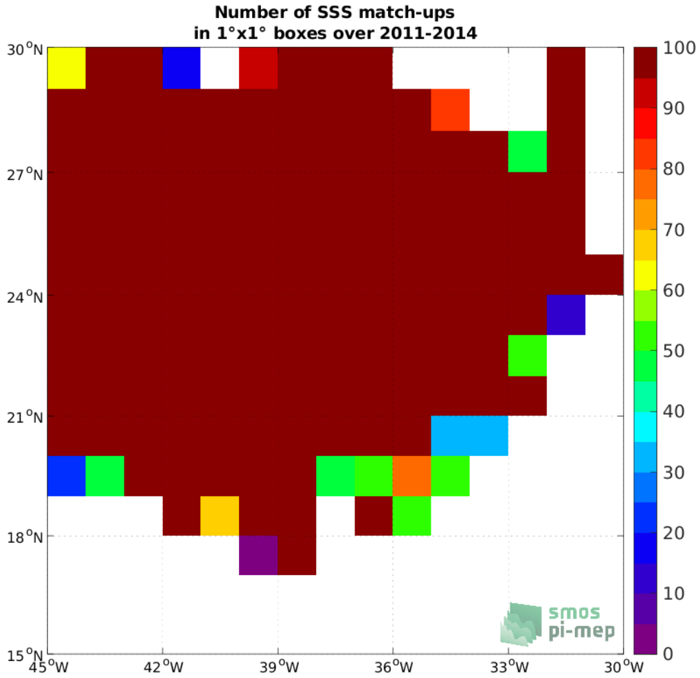
Figure 3: Number of SSS match-ups between Surface drifters SSS and the SMOS SSS L2 v700 (ESA) SSS product for the SPURS 1 Pi-MEP region over 1°x1° boxes and for the full satellite product period.
