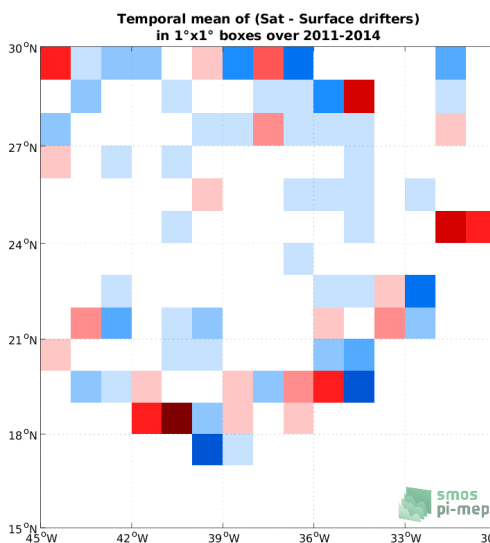
(e) MEAN( \Delta SSS) (Satellite - Surface drifters)
