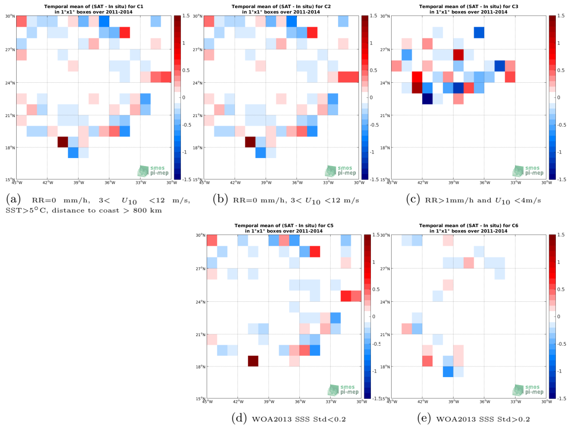
Figure 11: Temporal mean gridded over spatial boxes of size 1^\circ \times 1^\circ of \Delta\text{SSS} (SMOS SSS L2 v700 (ESA) - Surface drifters) for 5 different subdatasets corresponding to:RR=0 mm/h, 3 < U_{10} < 12 m/s, SST >5^\circ\text{C} , distance to coast > 800 km (a), RR=0 mm/h, 3 < U_{10} < 12 m/s (b), RR >1 mm/h and U_{10} < 4 m/s (c), WOA2013 SSS Std <0.2 (d), WOA2013 SSS Std >0.2 (e).
