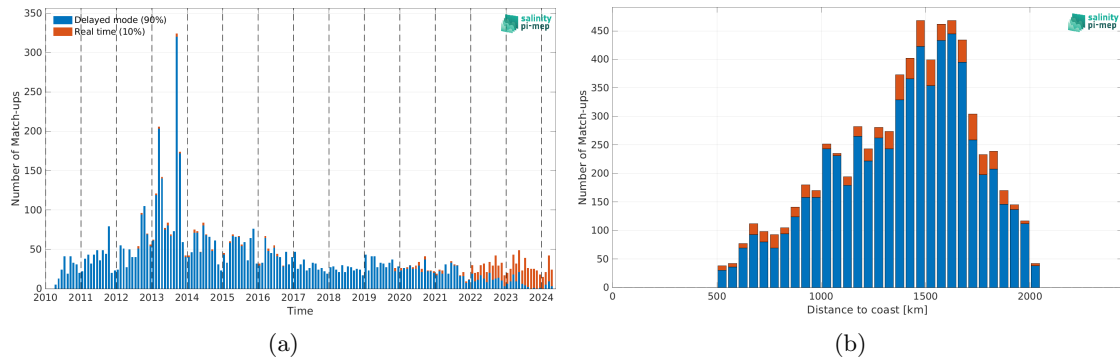
Figure 2: Number of match-ups between Argo and SMOS SSS L2 v700 (ESA) SSS as a function of time (a) and as function of the distance to coast (b) over the SPURS 1 Pi-MEP region and for the full satellite product period.
