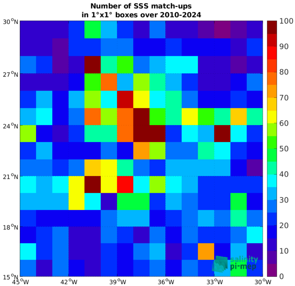
Figure 5: Number of SSS match-ups between Argo SSS and the SMOS SSS L2 v700 (ESA) SSS product for the SPURS 1 Pi-MEP region over 1°×1° boxes and for the full satellite product period.
