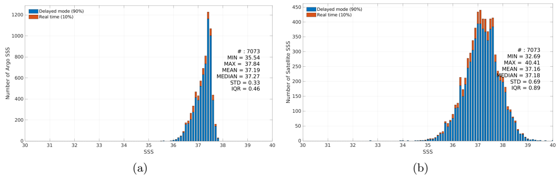
Figure 3: Histograms of SSS from Argo (a) and SMOS SSS L2 v700 (ESA) (b) considering all match-up pairs per bins of 0.1 over the SPURS 1 Pi-MEP region and for the full satellite product period.
