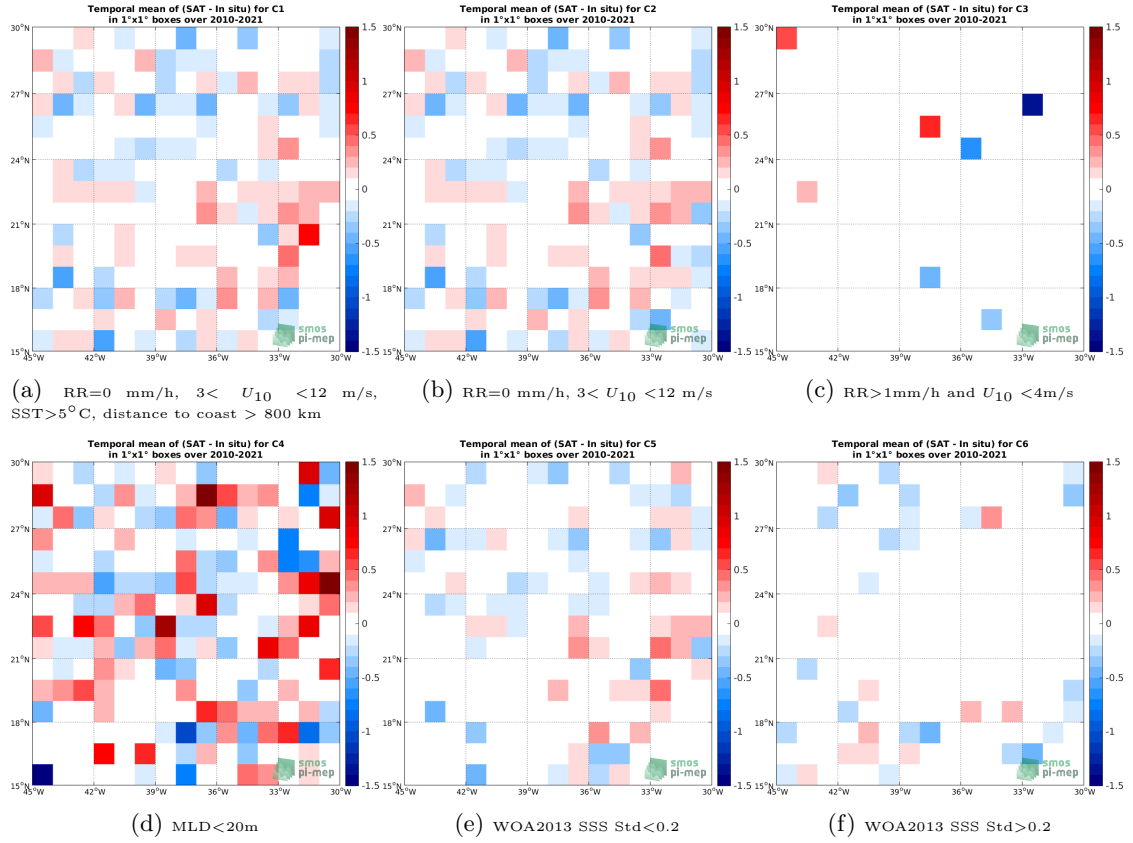
Figure 12: Temporal mean gridded over spatial boxes of size 1^\circ \times 1^\circ of \Delta SSS (SMOS SSS L2 v700 (ESA) - Argo) for 6 different subdatasets corresponding to: RR=0 mm/h, 3 < U_{10} < 12 m/s, SST >5^\circ C , distance to coast > 800 km (a), RR=0 mm/h, 3 < U_{10} < 12 m/s (b), RR >1 mm/h and U_{10} < 4 m/s (c), MLD <20 m (d), WOA2013 SSS Std <0.2 (e), WOA2013 SSS Std >0.2 (f).
