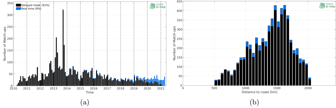
Figure 1: Number of match-ups between Argo and SMOS SSS L2 v700 (ESA) SSS as a function of time (a) and as function of the distance to coast (b) over the SPURS 1 Pi-MEP region and for the full satellite product period.
