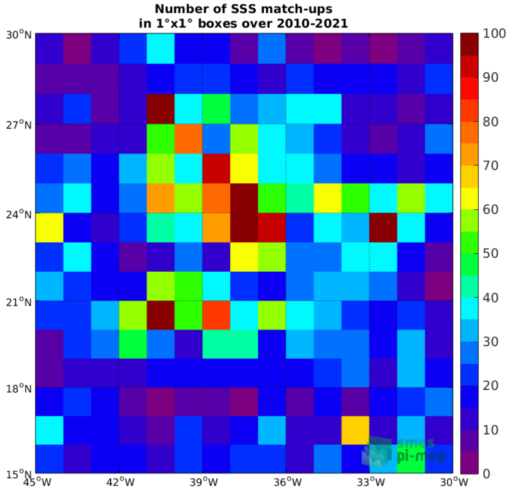
Figure 4: Number of SSS match-ups between Argo SSS and the SMOS SSS L2 v700 (ESA) SSS product for the SPURS 1 Pi-MEP region over 1°x1° boxes and for the full satellite product period.
