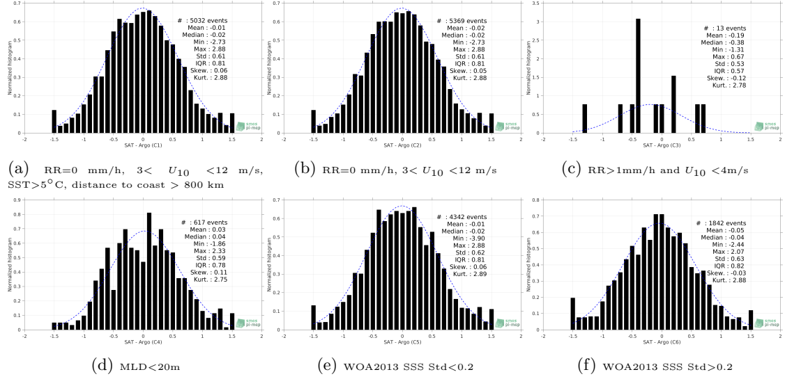
Figure 13: Normalized histogram of \Delta SSS (SMOS SSS L2 v700 (ESA) - Argo) for 6 different subdatasets corresponding to: RR=0 mm/h, 3 < U_{10} < 12 m/s, SST>5°C, distance to coast > 800 km (a), RR=0 mm/h, 3 < U_{10} < 12 m/s (b), RR>1mm/h and U_{10} < 4 m/s (c), MLD<20m (d), WOA2013 SSS Std<0.2 (e), WOA2013 SSS Std>0.2 (f).
