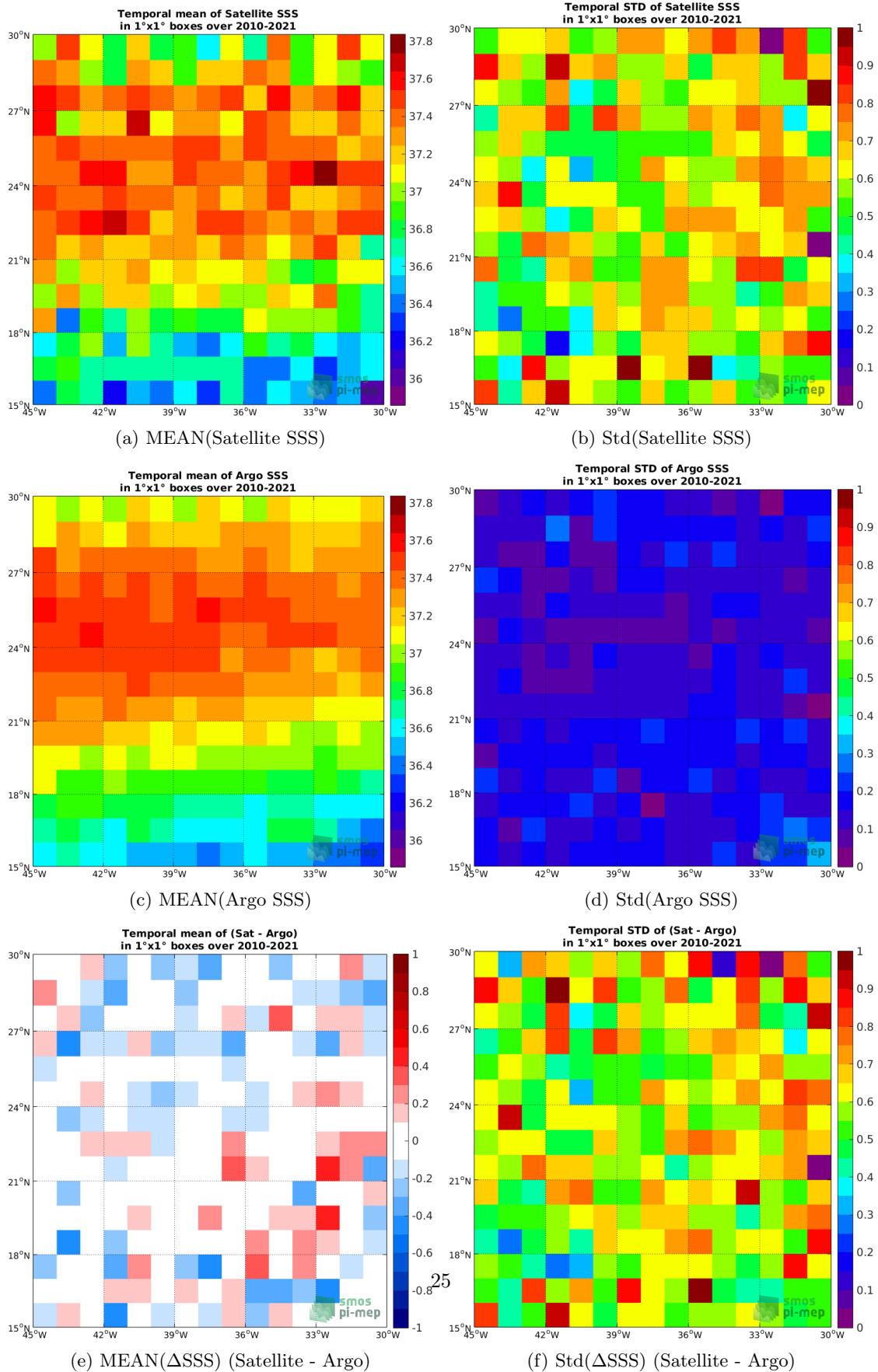
Figure 6: Temporal mean (left) and Std (right) of SSS from SMOS SSS L2 v700 (ESA) (top), Argo (middle), and of \Delta SSS (Satellite - Argo). Only match-up pairs are used to generate these maps.
