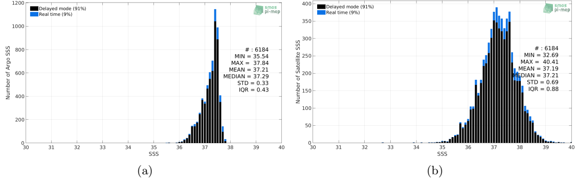
Figure 2: Histograms of SSS from Argo (a) and SMOS SSS L2 v700 (ESA) (b) considering all match-up pairs per bins of 0.1 over the SPURS 1 Pi-MEP region and for the full satellite product period.
