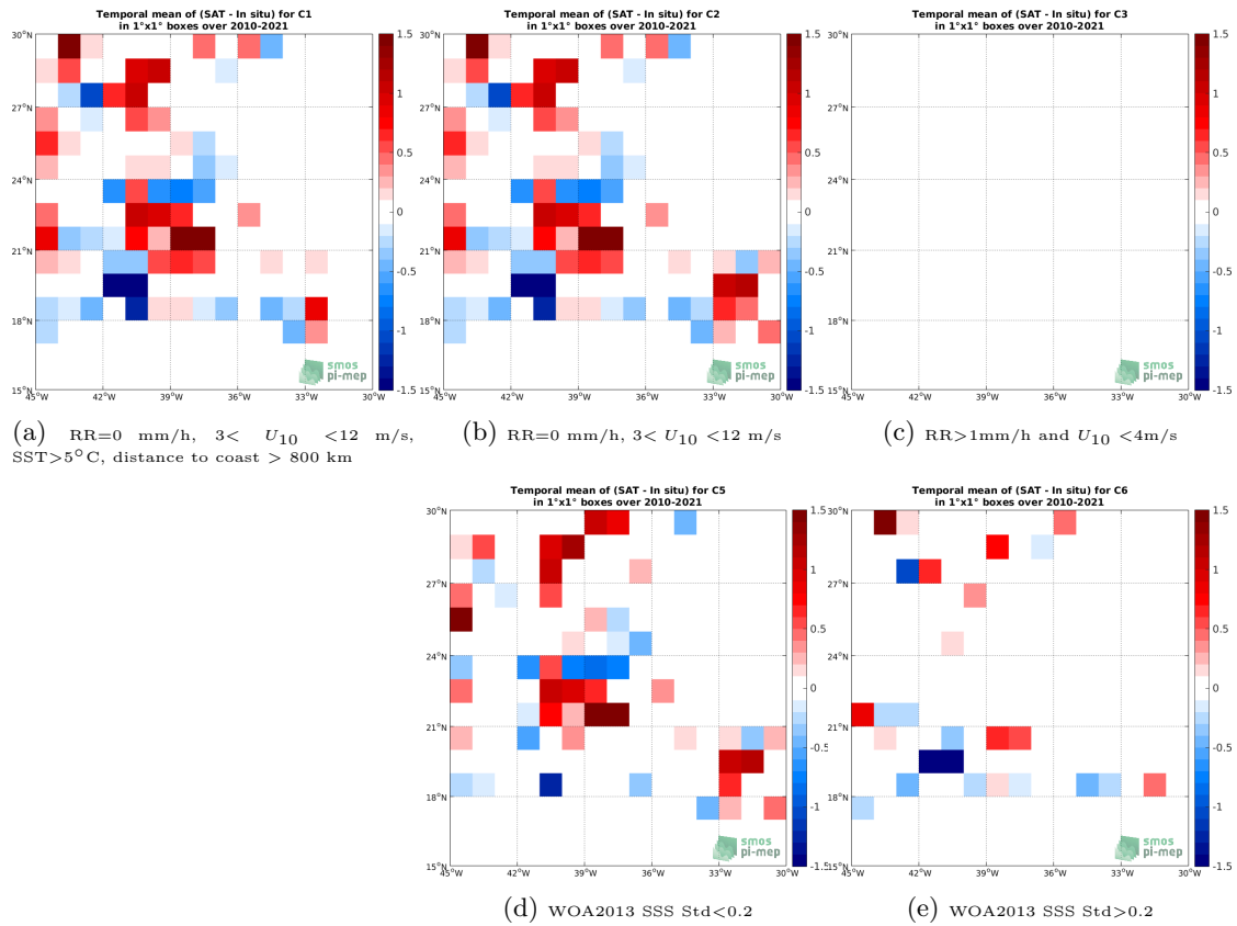
Figure 12: Temporal mean gridded over spatial boxes of size 1^\circ \times 1^\circ of \Delta SSS (SMOS SSS L2 v662 (ESA) - TSG (SAMOS)) for 5 different subdatasets corresponding to:RR=0 mm/h, 3 < U_{10} < 12 m/s, SST >5^\circ\text{C} , distance to coast > 800 km (a), RR=0 mm/h, 3 < U_{10} < 12 m/s (b), RR >1 mm/h and U_{10} < 4 m/s (c), WOA2013 SSS Std <0.2 (d), WOA2013 SSS Std >0.2 (e).
