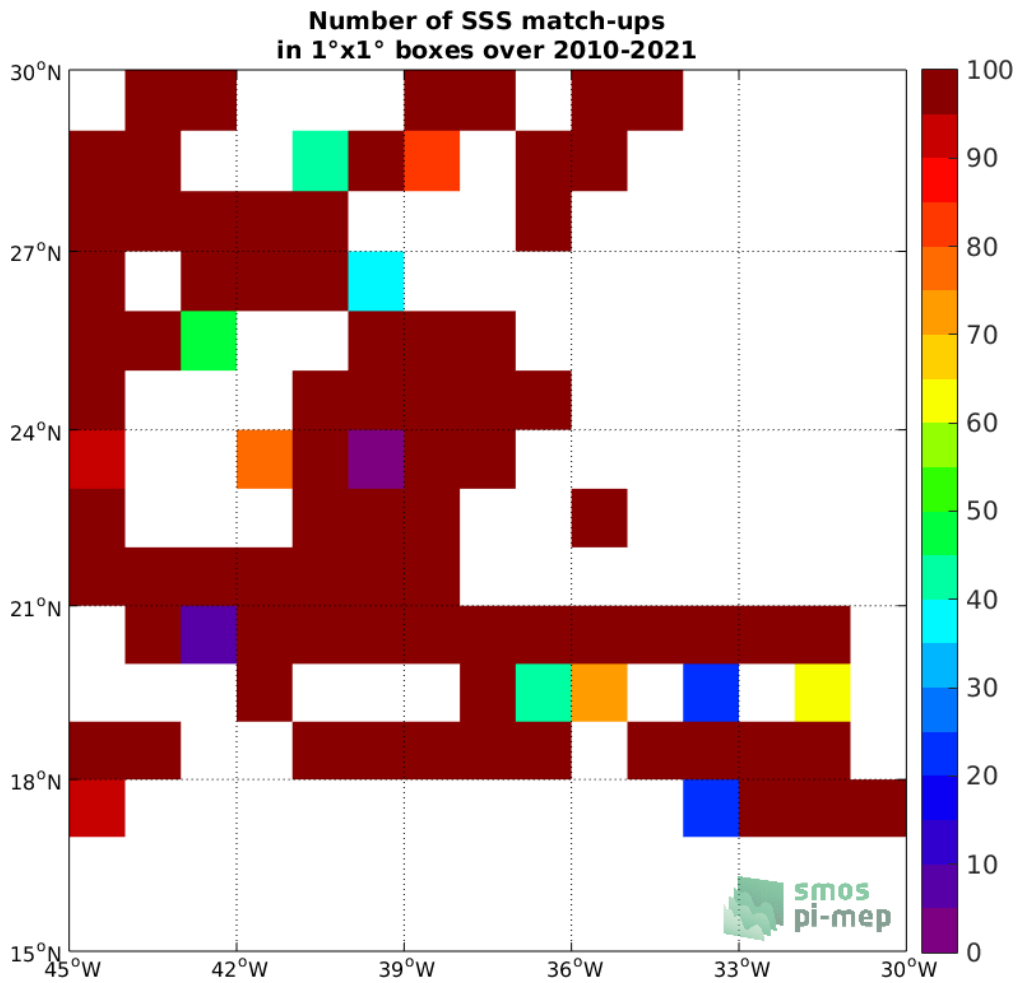
Figure 4: Number of SSS match-ups between TSG (SAMOS) SSS and the SMOS SSS L2 v662 (ESA) SSS product for the SPURS 1 Pi-MEP region over 1°x1° boxes and for the full satellite product period.
