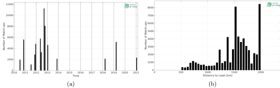
Figure 1: Number of match-ups between TSG (SAMOS) and SMOS SSS L2 v662 (ESA) SSS as a function of time (a) and as function of the distance to coast (b) over the SPURS 1 Pi-MEP region and for the full satellite product period.
