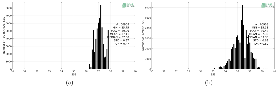
Figure 2: Histograms of SSS from TSG (SAMOS) (a) and SMOS SSS L2 v662 (ESA) (b) considering all match-up pairs per bins of 0.1 over the SPURS 1 Pi-MEP region and for the full satellite product period.
