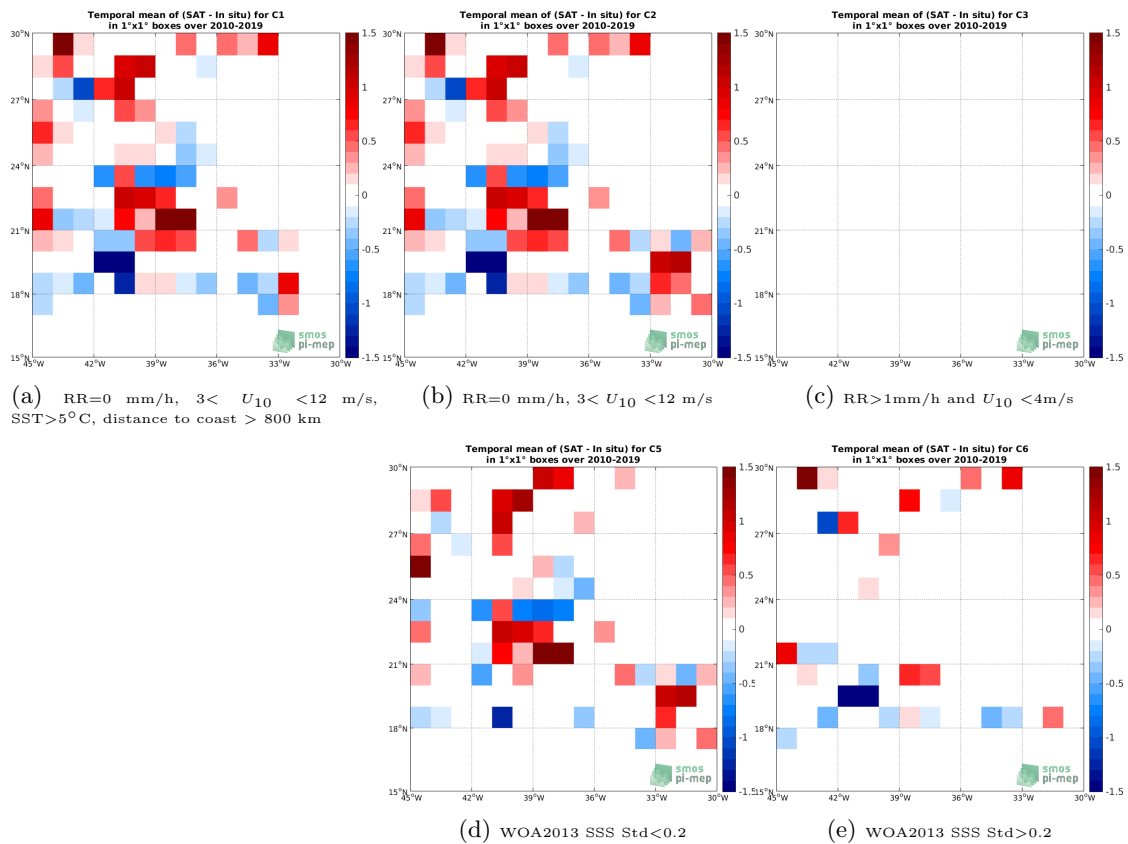
Figure 12: Temporal mean gridded over spatial boxes of size 1^\circ \times 1^\circ of \Delta\text{SSS} (SMOS SSS L2 v662 (ESA) - TSG (SAMOS)) for 5 different subdatasets corresponding to:RR=0 mm/h, 3 < U_{10} < 12 m/s, SST >5^\circ\text{C} , distance to coast > 800 km (a), RR=0 mm/h, 3 < U_{10} < 12 m/s (b), RR >1 mm/h and U_{10} < 4 m/s (c), WOA2013 SSS Std <0.2 (d), WOA2013 SSS Std >0.2 (e).
