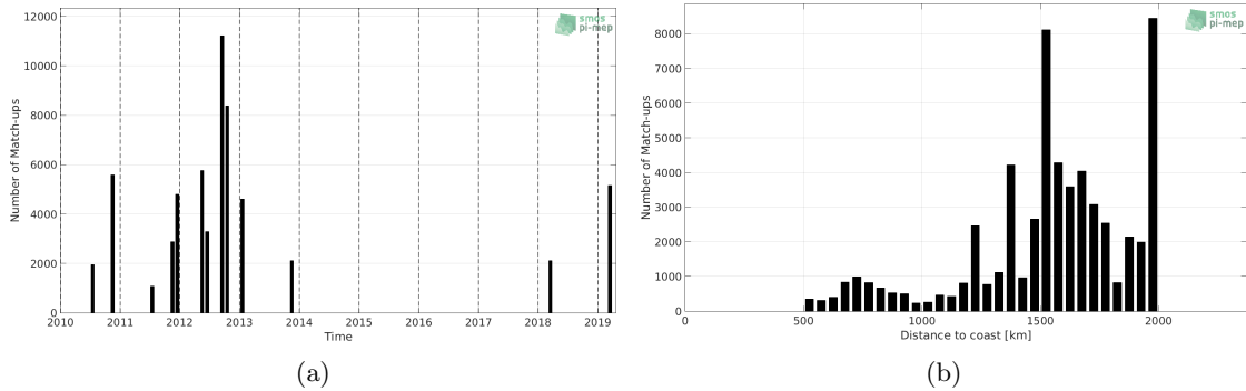
Figure 1: Number of match-ups between TSG-SAMOS and SMOS L2 v662 (ESA) SSS as a function of time (a) and as function of the distance to coast (b) over the SPURS 1 Pi-MEP region and for the full satellite product period.
