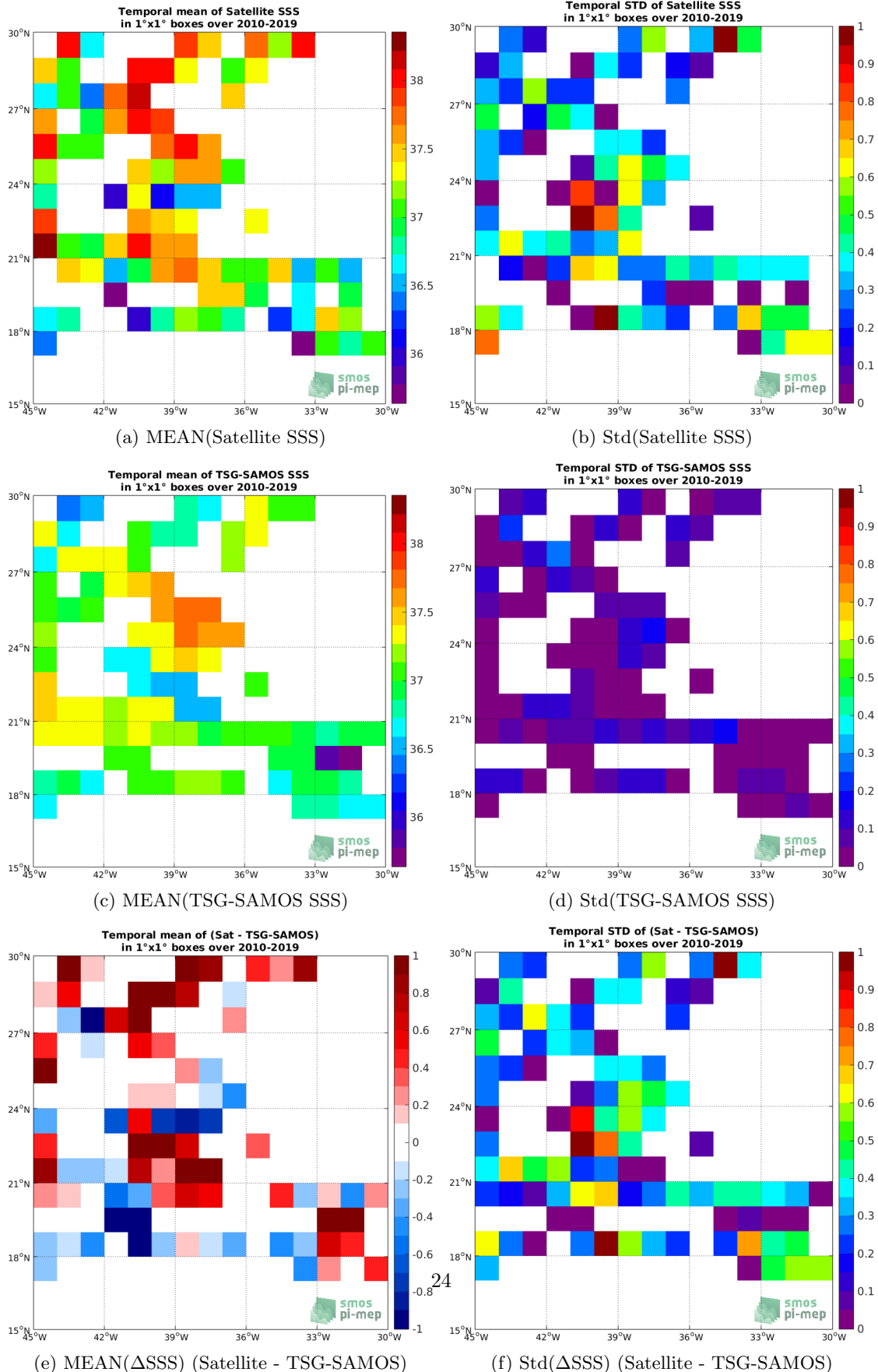
Figure 6: Temporal mean (left) and Std (right) of SSS from SMOS L2 v662 (ESA) (top), TSG-SAMOS (middle), and of \Delta SSS (Satellite - TSG-SAMOS). Only match-up pairs are used to generate these maps.
