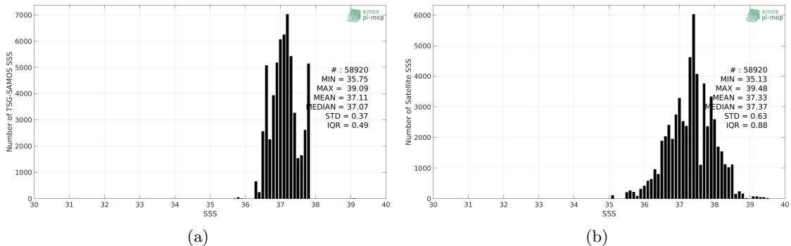
Figure 2: Histograms of SSS from TSG-SAMOS (a) and SMOS L2 v662 (ESA) (b) considering all match-up pairs per bins of 0.1 over the SPURS 1 Pi-MEP region and for the full satellite product period.
