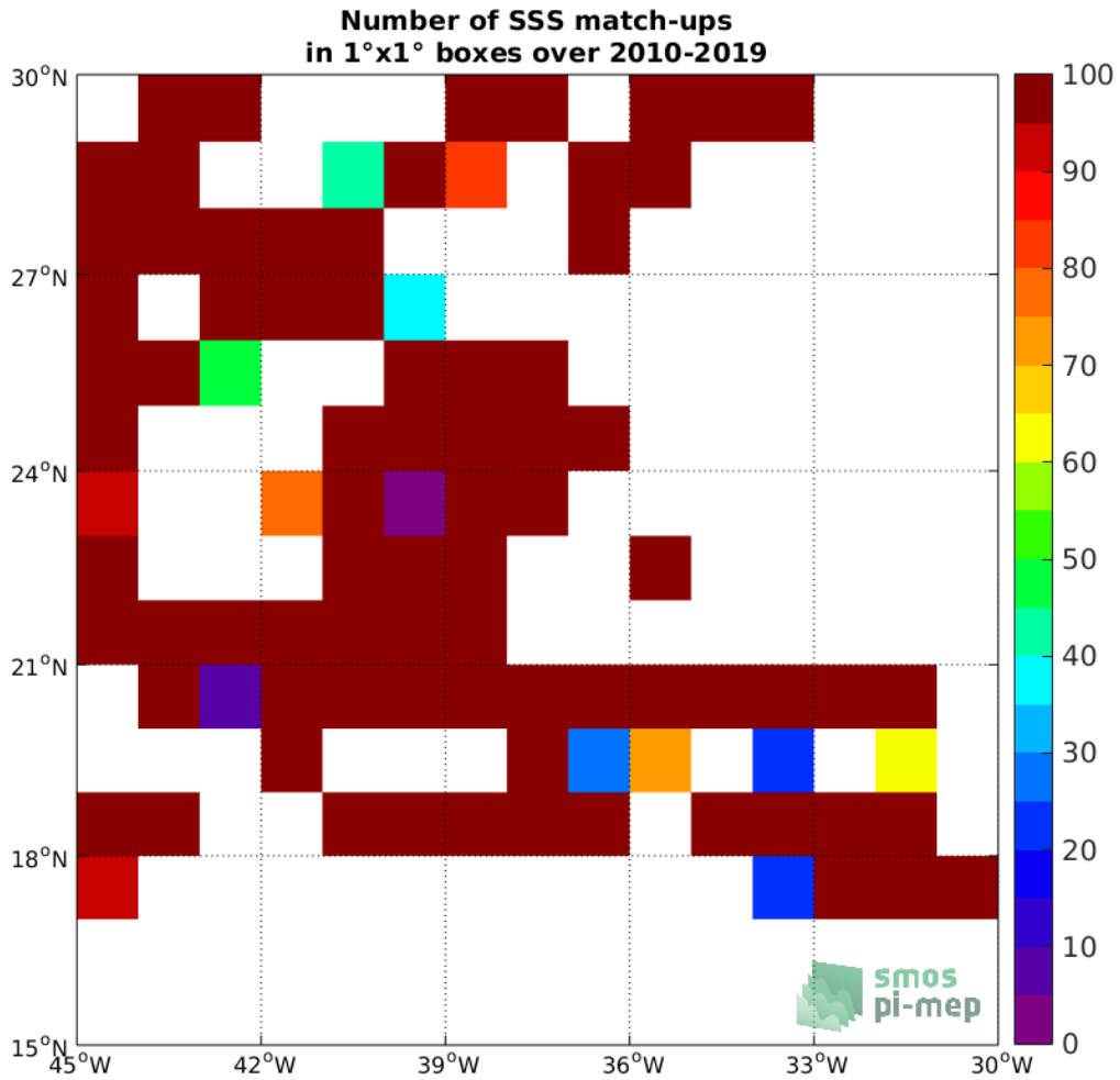
Figure 4: Number of SSS match-ups between TSG-SAMOS SSS and the SMOS L2 v662 (ESA) SSS product for the SPURS 1 Pi-MEP region over 1°x1° boxes and for the full satellite product period.
