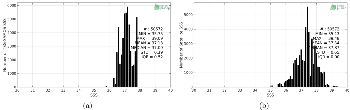
Figure 2: Histograms of SSS from TSG-SAMOS (a) and SMOS-L2-DPGS-v662 (b) considering all match-up pairs per bins of 0.1 over the SPURS 1 Pi-MEP region and for the full satellite product period.
