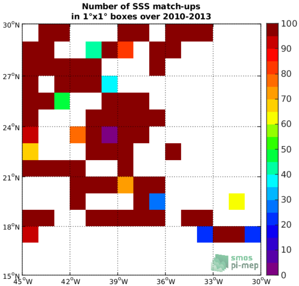
Figure 4: Number of SSS match-ups between TSG-SAMOS SSS and the SMOS-L2-DPGS-v662 SSS product for the SPURS 1 Pi-MEP region over 1°x1° boxes and for the full satellite product period.
