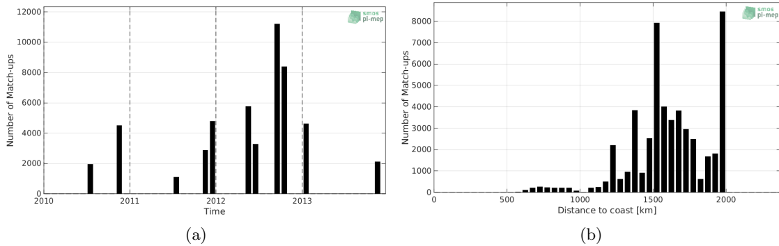
Figure 1: Number of match-ups between TSG-SAMOS and SMOS-L2-DPGS-v662 SSS as a function of time (a) and as function of the distance to coast (b) over the SPURS 1 Pi-MEP region and for the full satellite product period.
