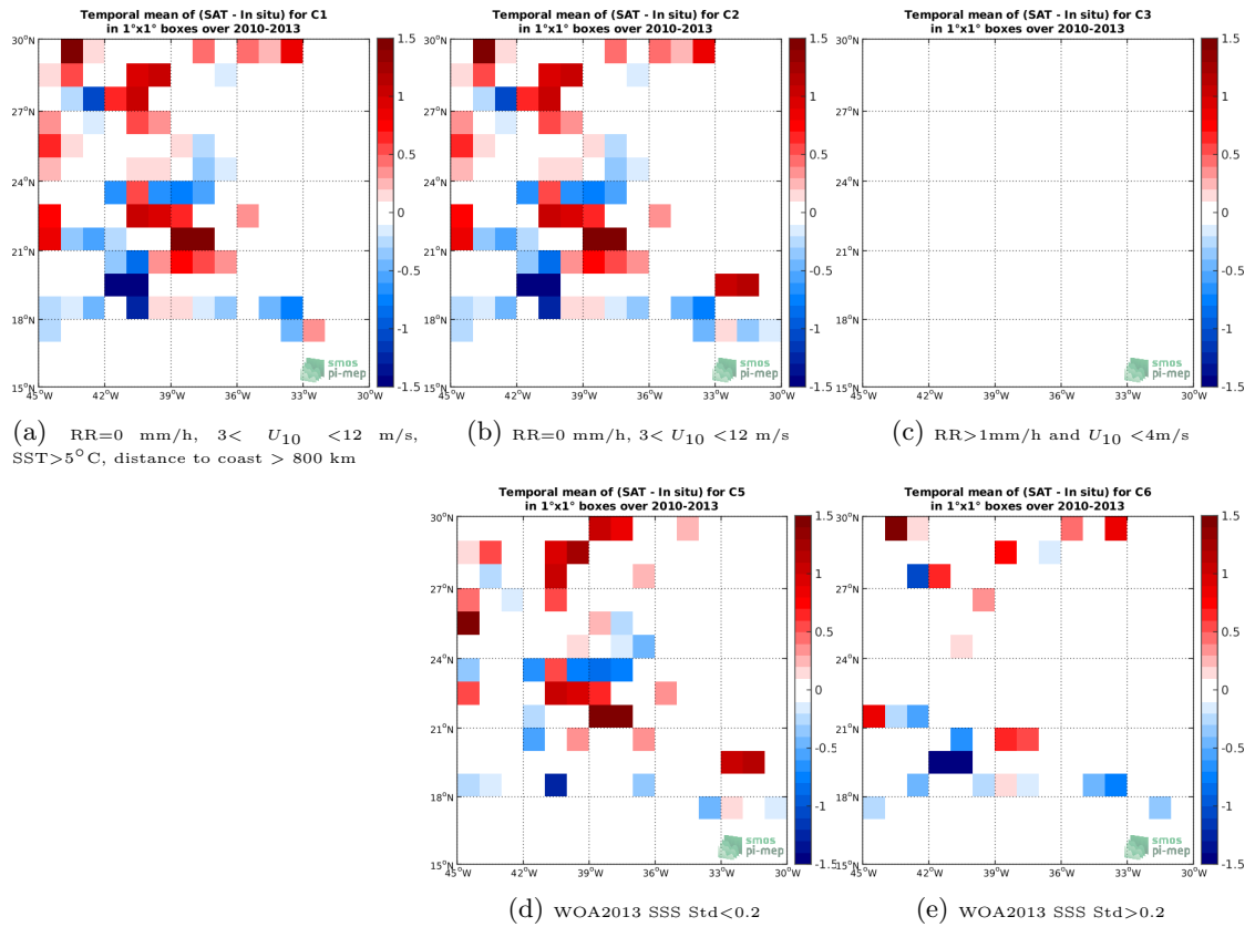
Figure 12: Temporal mean gridded over spatial boxes of size 1^\circ \times 1^\circ of \Delta SSS (SMOS-L2-DPGS-v662 - TSG-SAMOS) for 5 different subdatasets corresponding to:RR=0 mm/h, 3 < U_{10} < 12 m/s, SST >5^\circ\text{C} , distance to coast > 800 km (a), RR=0 mm/h, 3 < U_{10} < 12 m/s (b), RR >1 mm/h and U_{10} < 4 m/s (c), WOA2013 SSS Std <0.2 (d), WOA2013 SSS Std >0.2 (e).
