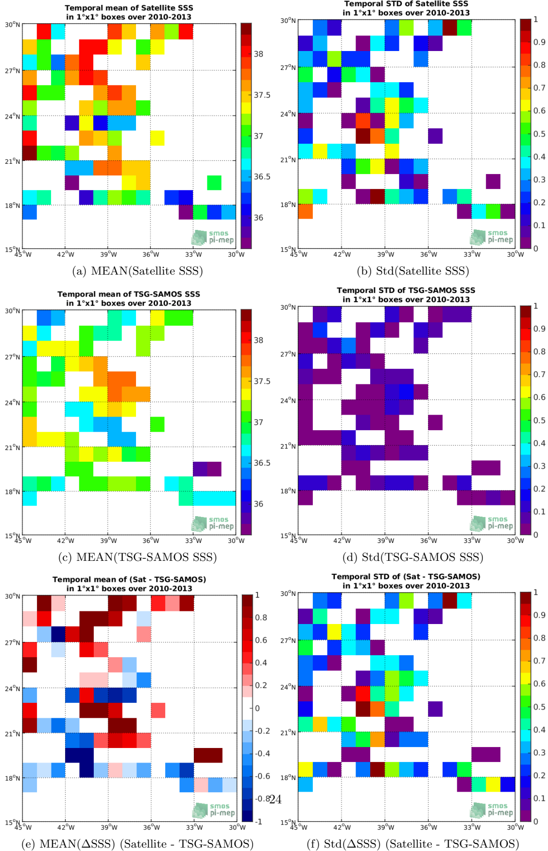
Figure 6: Temporal mean (left) and Std (right) of SSS from SMOS-L2-DPGS-v662 (top), TSG-SAMOS (middle), and of \Delta SSS (Satellite - TSG-SAMOS). Only match-up pairs are used to generate these maps.
