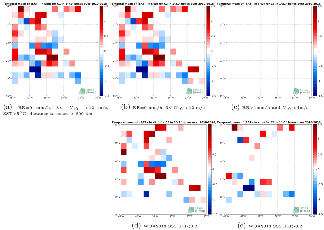
Figure 12: Temporal mean gridded over spatial boxes of size 1^\circ \times 1^\circ of \Delta SSS (SMOS-L2-DPGS-v662 - TSG-SAMOS) for 5 different subdatasets corresponding to:RR=0 mm/h, 3 < U_{10} < 12 m/s, SST >5^\circ C, distance to coast > 800 km (a), RR=0 mm/h, 3 < U_{10} < 12 m/s (b), RR >1 mm/h and U_{10} < 4 m/s (c), WOA2013 SSS Std <0.2 (d), WOA2013 SSS Std >0.2 (e).
