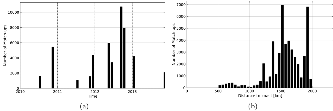
Figure 1: Number of match-ups between TSG-SAMOS and SMOS-L2-DPGS-v662 SSS as a function of time (a) and as function of the distance to coast (b) over the SPURS 1 Pi-MEP region and for the full satellite product period.
