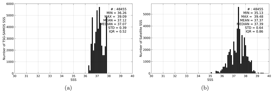
Figure 2: Histograms of SSS from TSG-SAMOS (a) and SMOS-L2-DPGS-v662 (b) considering all match-up pairs per bins of 0.1 over the SPURS 1 Pi-MEP region and for the full satellite product period.
