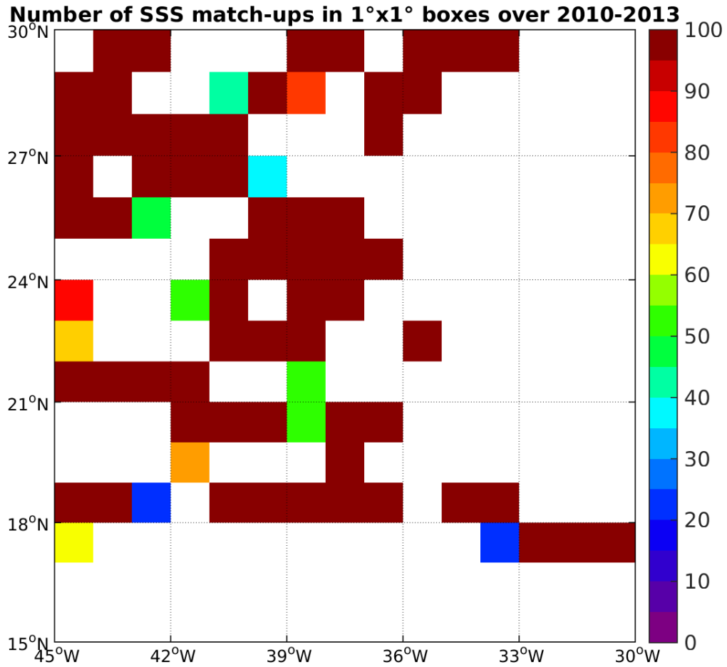
Figure 4: Number of SSS match-ups between TSG-SAMOS SSS and the SMOS-L2-DPGS-v662 SSS product for the SPURS 1 Pi-MEP region over 1°x1° boxes and for the full satellite product period.
