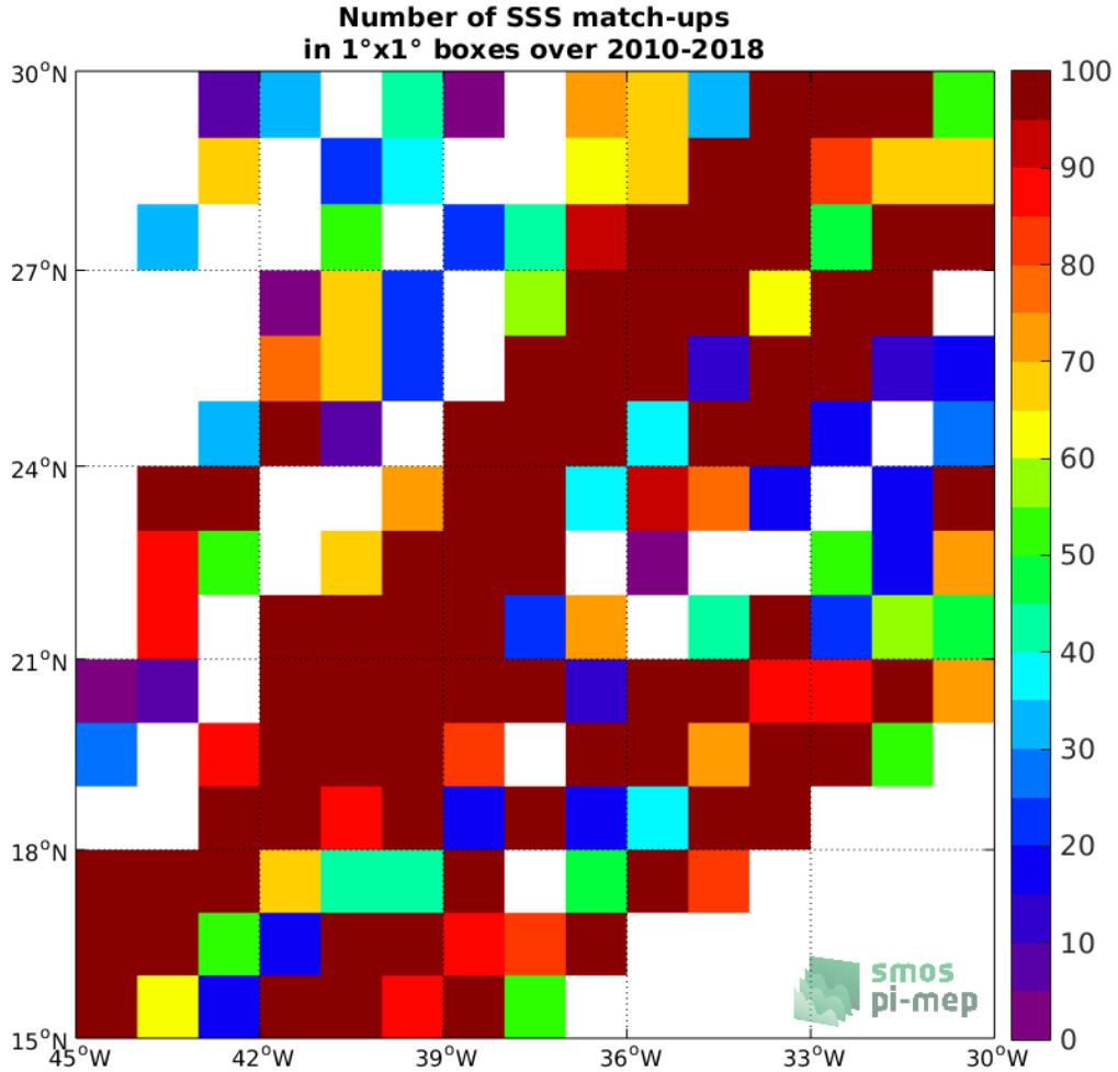
Figure 4: Number of SSS match-ups between TSG (LEGOS-DM) SSS and the SMOS SSS L2 v662 (ESA) SSS product for the SPURS 1 Pi-MEP region over 1°x1° boxes and for the full satellite product period.
