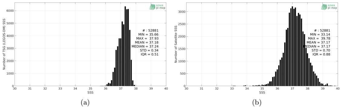
Figure 2: Histograms of SSS from TSG (LEGOS-DM) (a) and SMOS SSS L2 v662 (ESA) (b) considering all match-up pairs per bins of 0.1 over the SPURS 1 Pi-MEP region and for the full satellite product period.
