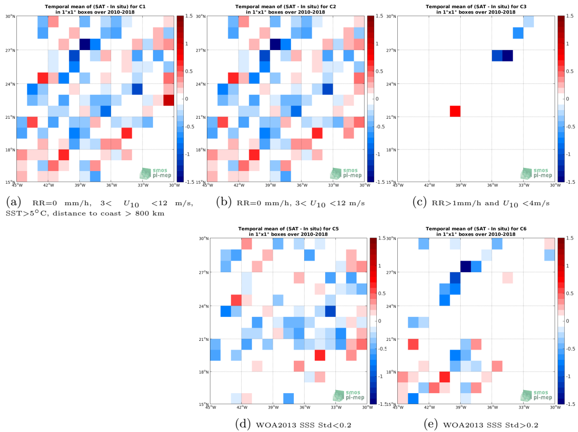
Figure 12: Temporal mean gridded over spatial boxes of size 1^\circ \times 1^\circ of \Delta SSS (SMOS SSS L2 v662 (ESA) - TSG (LEGOS-DM)) for 5 different subdatasets corresponding to: RR=0 mm/h, 3 < U_{10} < 12 m/s, SST > 5^\circ C , distance to coast > 800 km (a), RR=0 mm/h, 3 < U_{10} < 12 m/s (b), RR > 1 mm/h and U_{10} < 4 m/s (c), WOA2013 SSS Std < 0.2 (d), WOA2013 SSS Std > 0.2 (e).
