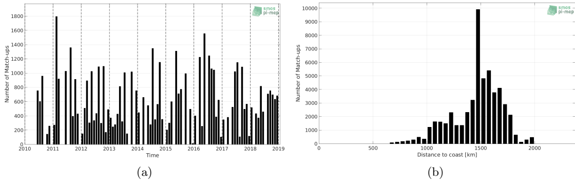
Figure 1: Number of match-ups between TSG (LEGOS-DM) and SMOS SSS L2 v662 (ESA) SSS as a function of time (a) and as function of the distance to coast (b) over the SPURS 1 Pi-MEP region and for the full satellite product period.
