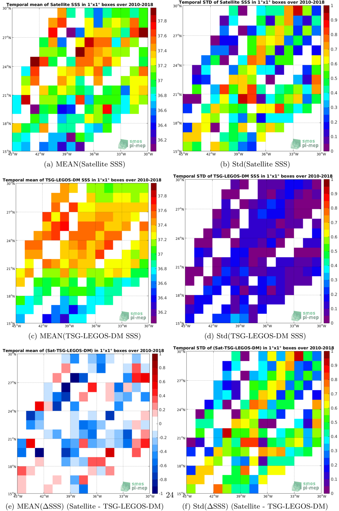
Figure 6: Temporal mean (left) and Std (right) of SSS from SMOS-L2-DPGS-v662 (top), TSG-LEGOS-DM (middle), and of \Delta SSS (Satellite - TSG-LEGOS-DM). Only match-up pairs are used to generate these maps.
