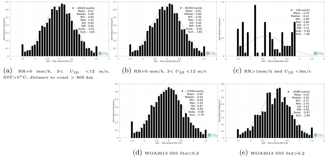
Figure 13: Normalized histogram of \Delta\text{SSS} (SMOS-L2-DPGS-v662 - TSG-LEGOS-DM) for 5 different subdatasets corresponding to: RR=0 mm/h, 3 < U_{10} < 12 m/s, SST > 5^\circ\text{C} , distance to coast > 800 km (a), RR=0 mm/h, 3 < U_{10} < 12 m/s (b), RR > 1 mm/h and U_{10} < 4 m/s (c), WOA2013 SSS Std < 0.2 (d), WOA2013 SSS Std > 0.2 (e).
