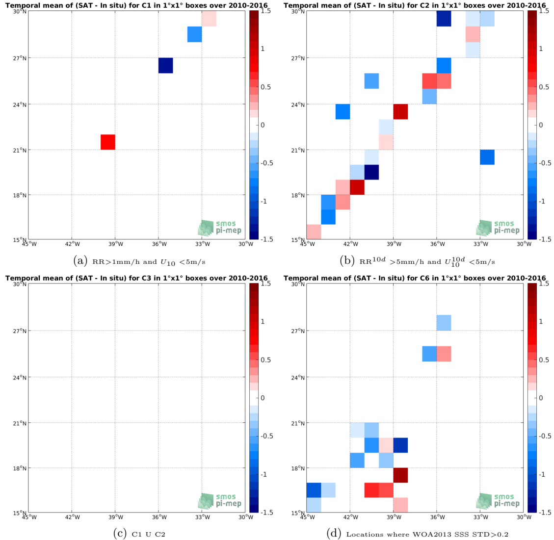
Figure 12: Temporal mean gridded over spatial boxes of size 1^\circ \times 1^\circ of \Delta SSS (SMOS-L2-DPGS-v662 - TSG-LEGOS-DM) for 4 different subdatasets corresponding to: RR > 1\text{mm/h} and U_{10} < 5\text{m/s} (a), RR^{10d} > 5\text{mm/h} and U_{10}^{10d} < 5\text{m/s} (b), C1 U C2 (c), Locations where WOA2013 SSS STD > 0.2 (d).
