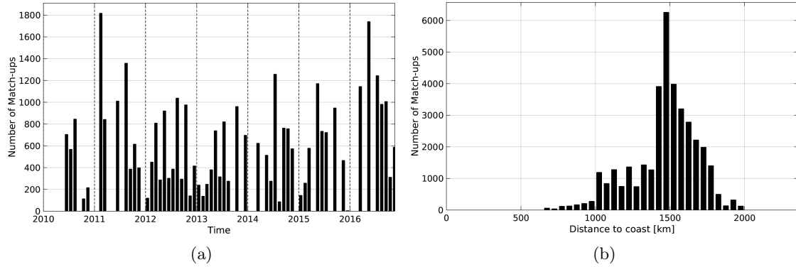
Figure 1: Number of match-ups between TSG-LEGOS-DM and SMOS-L2-DPGS-v662 SSS as a function of time (a) and as function of the distance to coast (b) over the SPURS 1 Pi-MEP region and for the full satellite product period.
