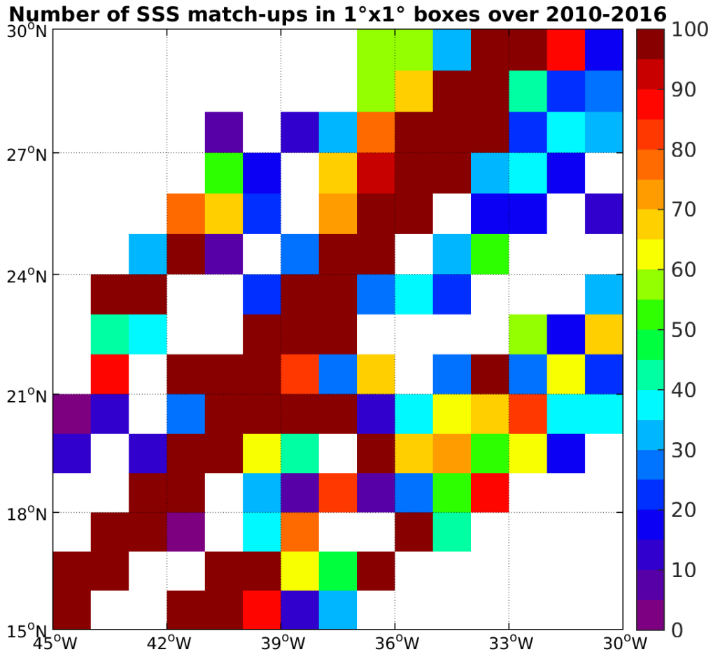
Figure 4: Number of SSS match-ups between TSG-LEGOS-DM SSS and the SMOS-L2-DPGS-v662 SSS product for the SPURS 1 Pi-MEP region over 1°x1° boxes and for the full satellite product period.
