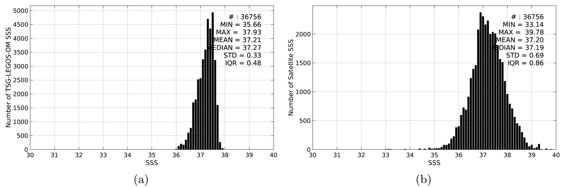
Figure 2: Histograms of SSS from TSG-LEGOS-DM (a) and SMOS-L2-DPGS-v662 (b) considering all match-up pairs per bins of 0.1 over the SPURS 1 Pi-MEP region and for the full satellite product period.
