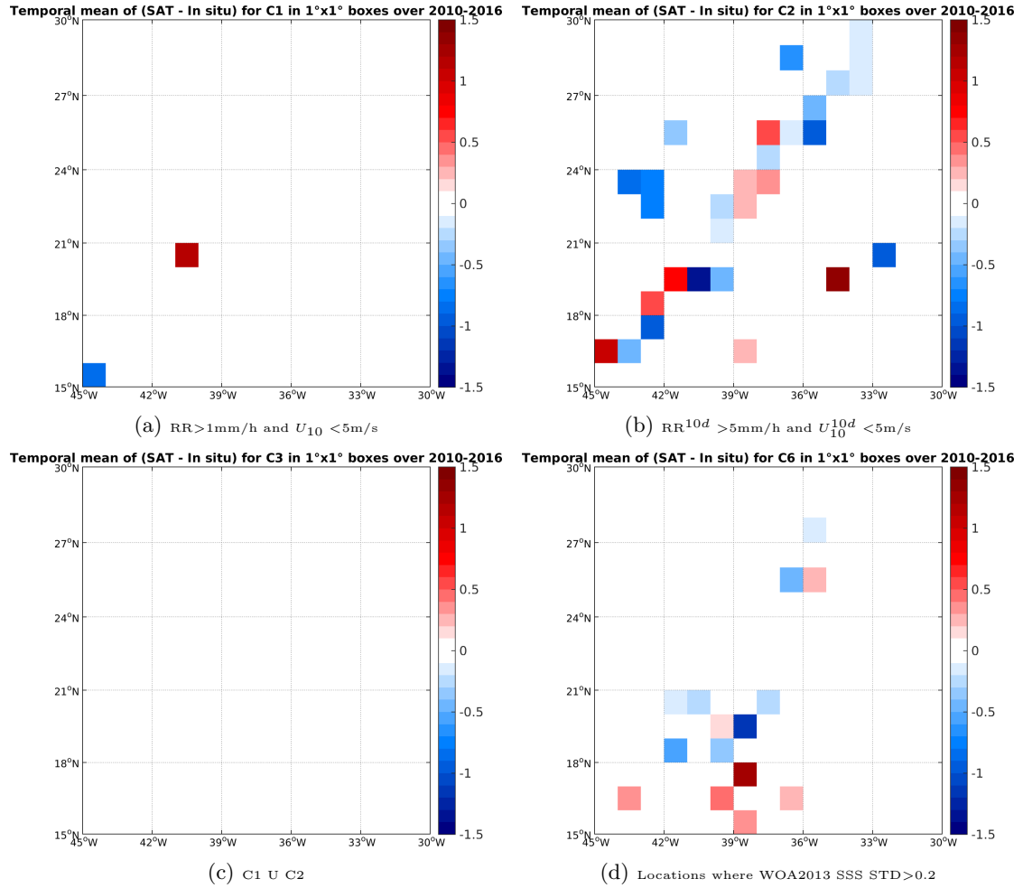
Figure 12: Temporal mean gridded over spatial boxes of size 1^\circ \times 1^\circ of \Delta SSS (SMOS-L2-DPGS-v662 - TSG-LEGOS-DM) for 4 different subdatasets corresponding to: RR > 1\text{mm/h} and U_{10} < 5\text{m/s} (a), RR^{10d} > 5\text{mm/h} and U_{10}^{10d} < 5\text{m/s} (b), C1 U C2 (c), Locations where WOA2013 SSS STD > 0.2 (d).
