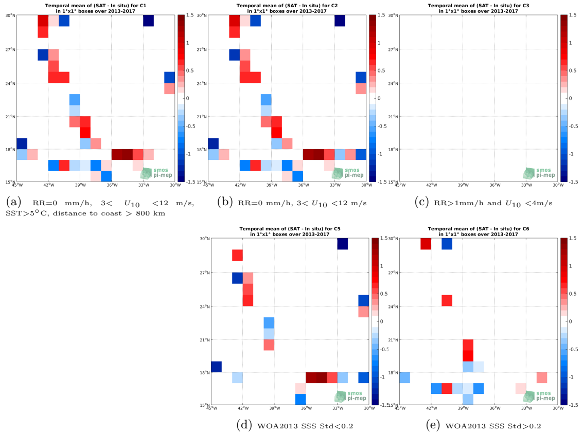
Figure 12: Temporal mean gridded over spatial boxes of size 1^\circ \times 1^\circ of \Delta SSS (SMOS SSS L2 v662 (ESA) - TSG (GOSUD-Sailing-ship)) for 5 different subdatasets corresponding to: RR=0 mm/h, 3 < U_{10} < 12 m/s, SST >5^\circ C, distance to coast > 800 km (a), RR=0 mm/h, 3 < U_{10} < 12 m/s (b), RR >1 mm/h and U_{10} < 4 m/s (c), WOA2013 SSS Std <0.2 (d), WOA2013 SSS Std >0.2 (e).
