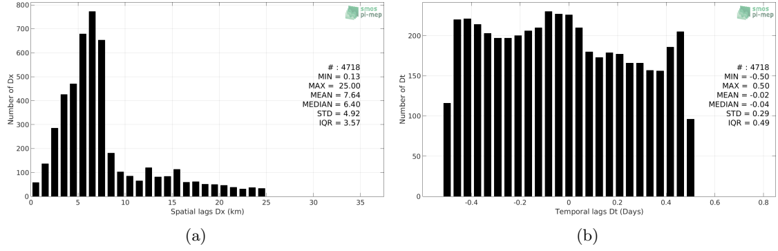
Figure 5: Histograms of the spatial (a) and temporal (b) lags between the location/time of the TSG (GOSUD-Sailing-ship) measurement and the date of the corresponding SMOS SSS L2 v662 (ESA) SSS pixel.
