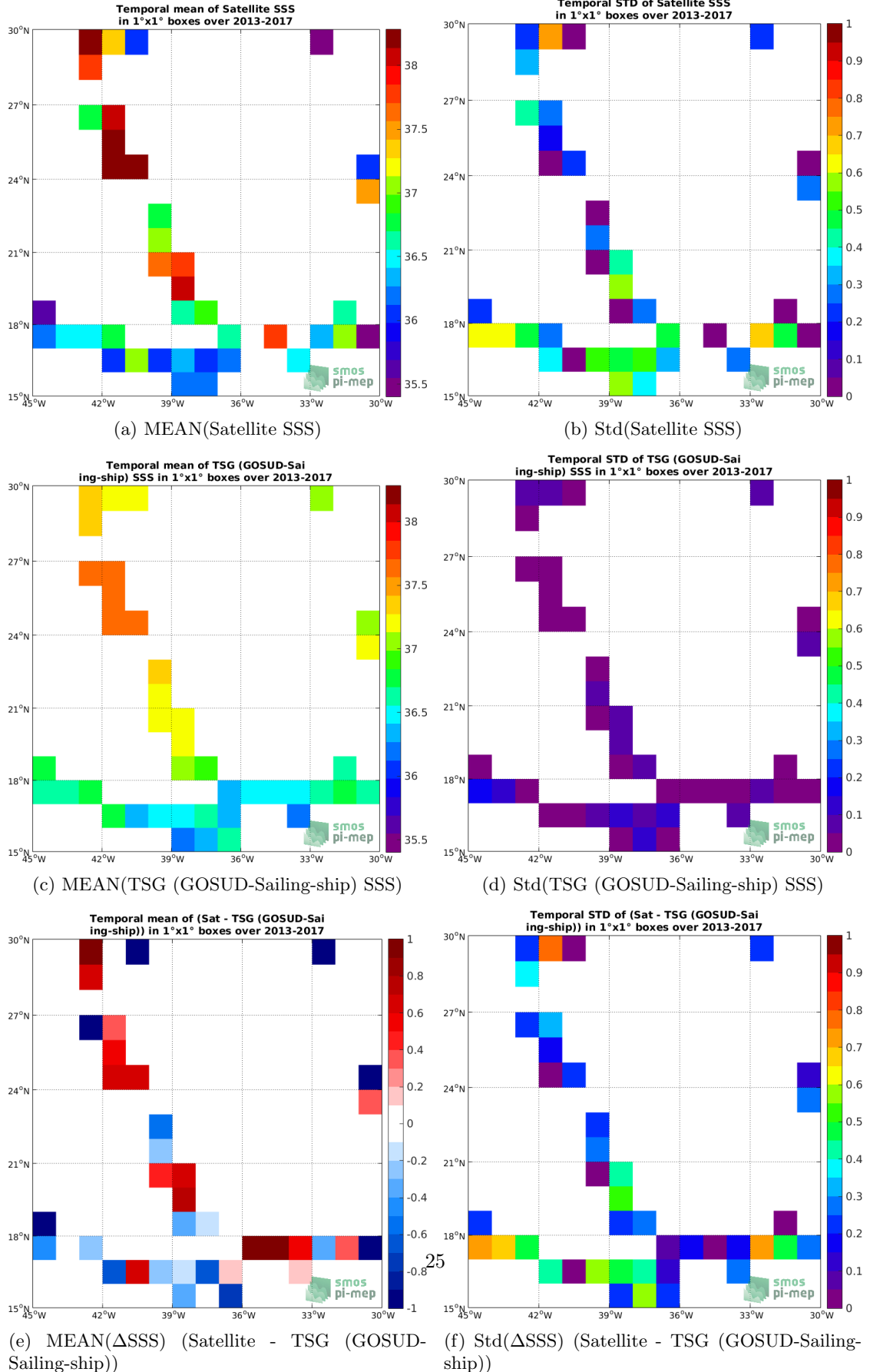
Figure 6: Temporal mean (left) and Std (right) of SSS from SMOS SSS L2 v662 (ESA) (top), TSG (GOSUD-Sailing-ship) (middle), and of \Delta SSS (Satellite - TSG (GOSUD-Sailing-ship)). Only match-up pairs are used to generate these maps.
