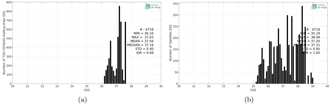
Figure 2: Histograms of SSS from TSG (GOSUD-Sailing-ship) (a) and SMOS SSS L2 v662 (ESA) (b) considering all match-up pairs per bins of 0.1 over the SPURS 1 Pi-MEP region and for the full satellite product period.
