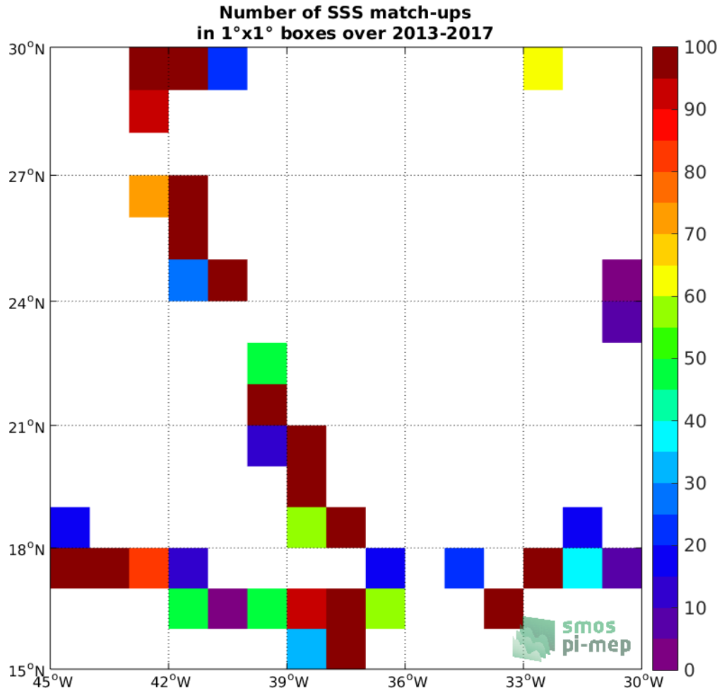
Figure 4: Number of SSS match-ups between TSG (GOSUD-Sailing-ship) SSS and the SMOS SSS L2 v662 (ESA) SSS product for the SPURS 1 Pi-MEP region over 1°x1° boxes and for the full satellite product period.
