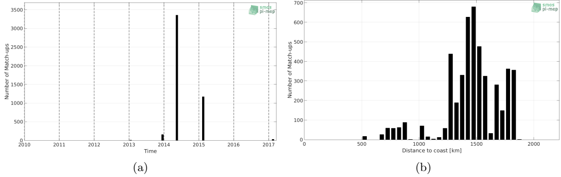
Figure 1: Number of match-ups between TSG (GOSUD-Sailing-ship) and SMOS SSS L2 v662 (ESA) SSS as a function of time (a) and as function of the distance to coast (b) over the SPURS 1 Pi-MEP region and for the full satellite product period.
