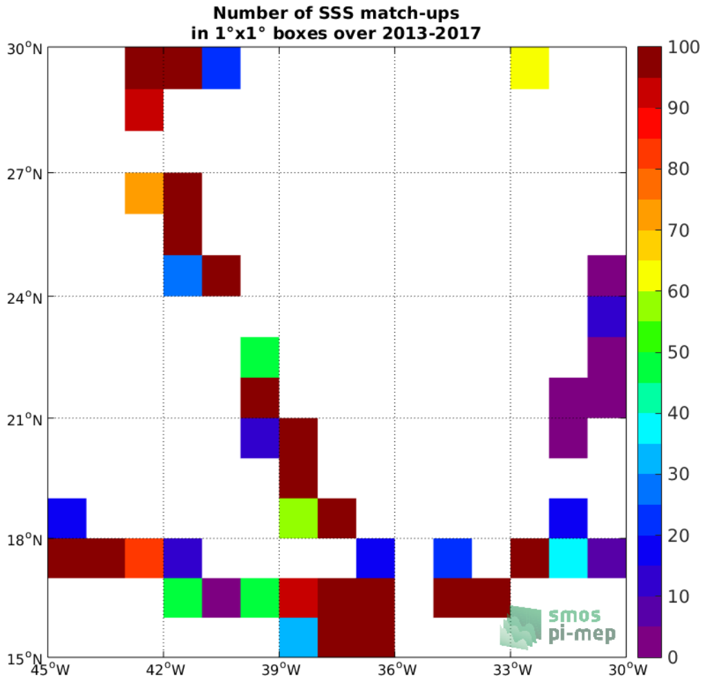
Figure 4: Number of SSS match-ups between TSG-GOSUD-Sailing-ship SSS and the SMOS L2 v662 (ESA) SSS product for the SPURS 1 Pi-MEP region over 1°x1° boxes and for the full satellite product period.
