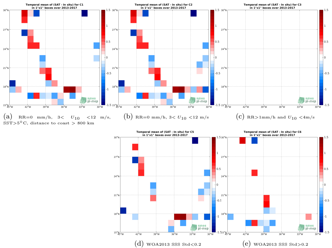
Figure 12: Temporal mean gridded over spatial boxes of size 1^\circ \times 1^\circ of \Delta SSS (SMOS L2 v662 (ESA) - TSG-GOSUD-Sailing-ship) for 5 different subdatasets corresponding to:RR=0 mm/h, 3 < U_{10} < 12 m/s, SST >5^\circ\text{C} , distance to coast > 800 km (a), RR=0 mm/h, 3 < U_{10} < 12 m/s (b), RR >1 mm/h and U_{10} < 4 m/s (c), WOA2013 SSS Std <0.2 (d), WOA2013 SSS Std >0.2 (e).
