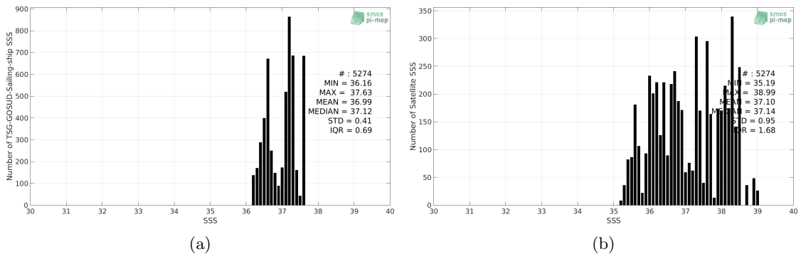
Figure 2: Histograms of SSS from TSG-GOSUD-Sailing-ship (a) and SMOS L2 v662 (ESA) (b) considering all match-up pairs per bins of 0.1 over the SPURS 1 Pi-MEP region and for the full satellite product period.
