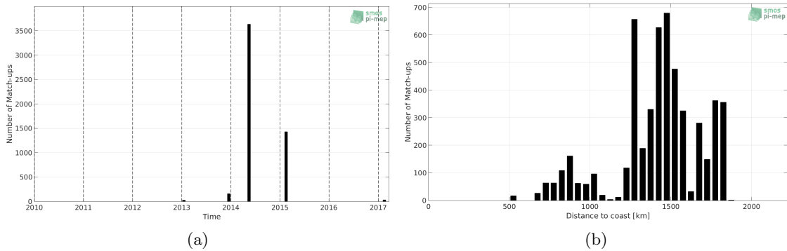
Figure 1: Number of match-ups between TSG-GOSUD-Sailing-ship and SMOS L2 v662 (ESA) SSS as a function of time (a) and as function of the distance to coast (b) over the SPURS 1 Pi-MEP region and for the full satellite product period.
