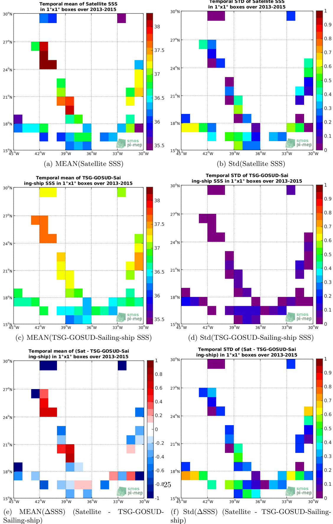
Figure 6: Temporal mean (left) and Std (right) of SSS from SMOS-L2-DPGS-v662 (top), TSG-GOSUD-Sailing-ship (middle), and of \Delta SSS (Satellite - TSG-GOSUD-Sailing-ship). Only match-up pairs are used to generate these maps.
