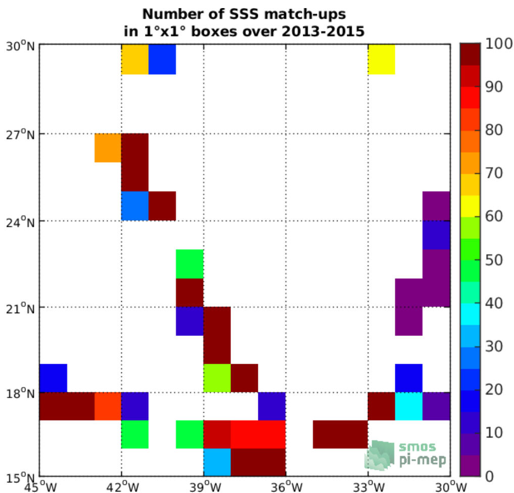
Figure 4: Number of SSS match-ups between TSG-GOSUD-Sailing-ship SSS and the SMOS-L2-DPGS-v662 SSS product for the SPURS 1 Pi-MEP region over 1°x1° boxes and for the full satellite product period.
