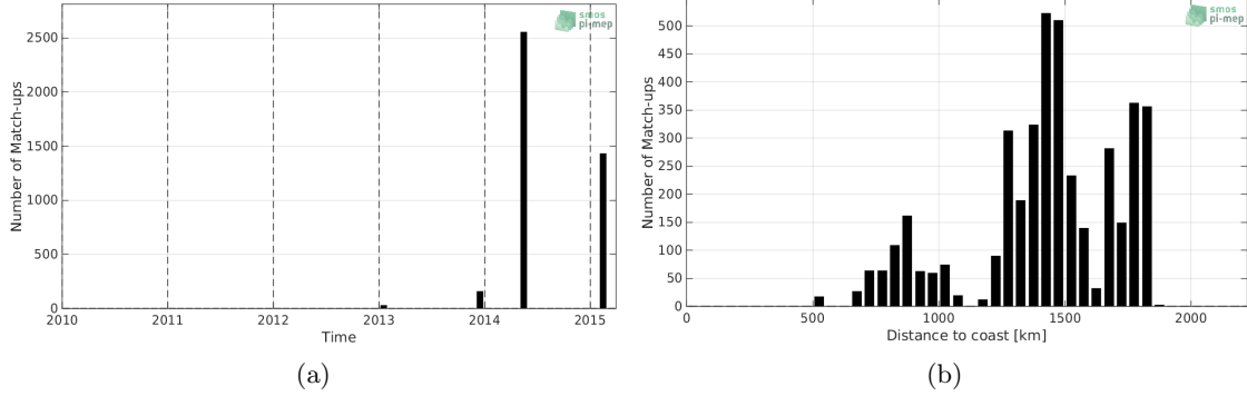
Figure 1: Number of match-ups between TSG-GOSUD-Sailing-ship and SMOS-L2-DPGS-v662 SSS as a function of time (a) and as function of the distance to coast (b) over the SPURS 1 Pi-MEP region and for the full satellite product period.
