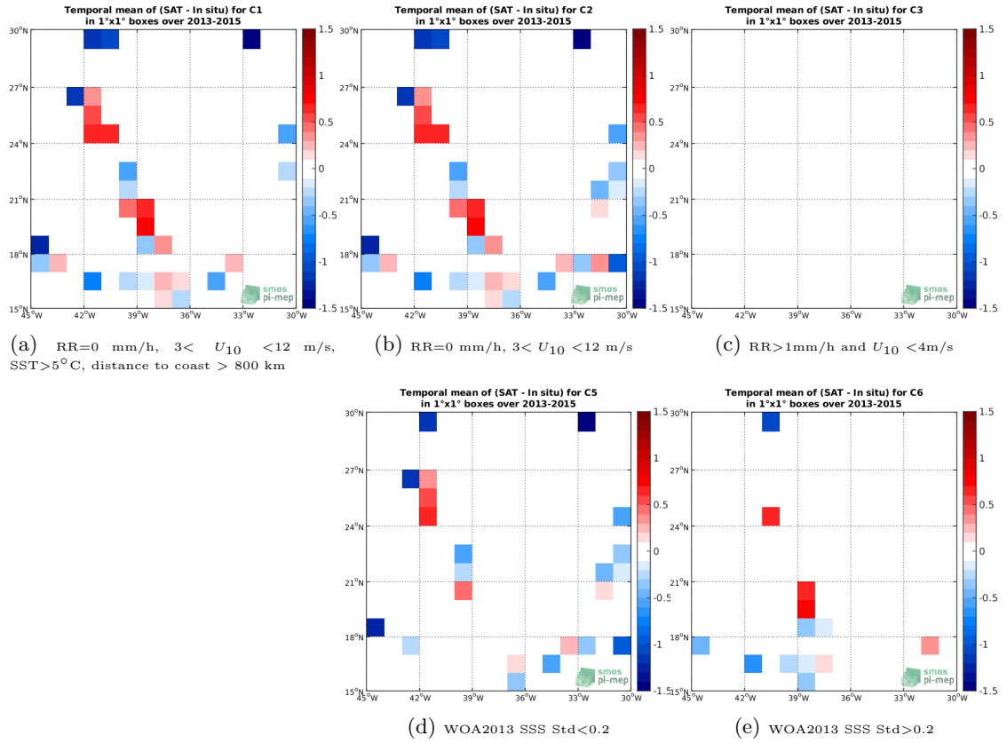
Figure 12: Temporal mean gridded over spatial boxes of size 1^\circ \times 1^\circ of \Delta SSS (SMOS-L2-DPGS-v662 - TSG-GOSUD-Sailing-ship) for 5 different subdatasets corresponding to: RR=0 mm/h, 3 < U_{10} < 12 m/s, SST >5^\circ C, distance to coast > 800 km (a), RR=0 mm/h, 3 < U_{10} < 12 m/s (b), RR >1 mm/h and U_{10} < 4 m/s (c), WOA2013 SSS Std <0.2 (d), WOA2013 SSS Std >0.2 (e).
