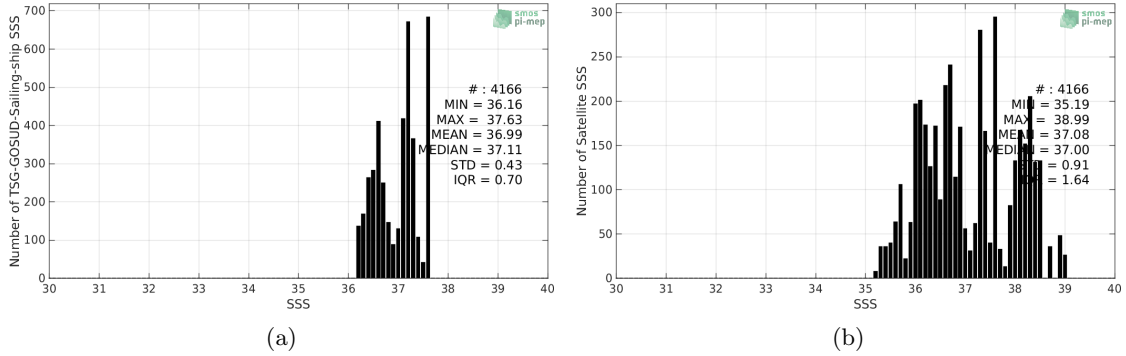
Figure 2: Histograms of SSS from TSG-GOSUD-Sailing-ship (a) and SMOS-L2-DPGS-v662 (b) considering all match-up pairs per bins of 0.1 over the SPURS 1 Pi-MEP region and for the full satellite product period.
