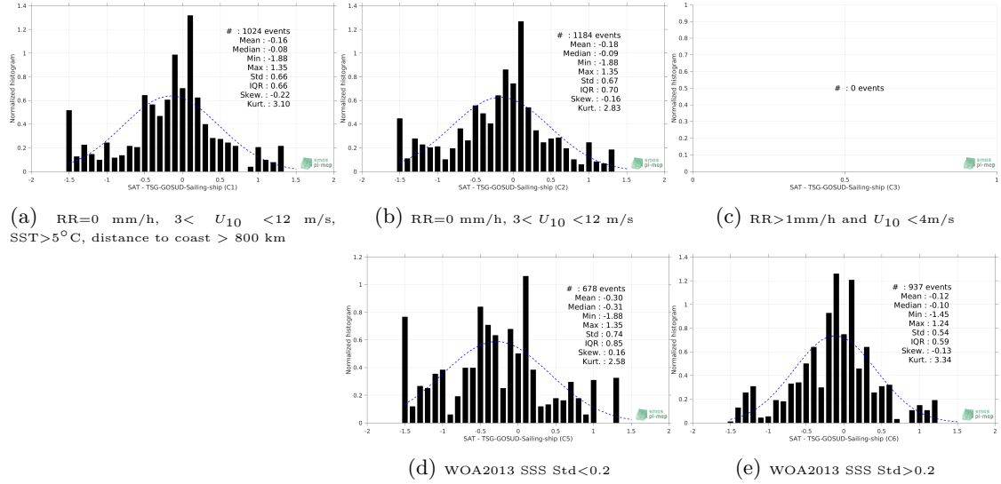
Figure 13: Normalized histogram of \Delta SSS (SMOS-L2-DPGS-v662 - TSG-GOSUD-Sailing-ship) for 5 different subdatasets corresponding to: RR=0 mm/h, 3 < U_{10} < 12 m/s, SST > 5°C, distance to coast > 800 km (a), RR=0 mm/h, 3 < U_{10} < 12 m/s (b), RR > 1mm/h and U_{10} < 4 m/s (c), WOA2013 SSS Std < 0.2 (d), WOA2013 SSS Std > 0.2 (e).
