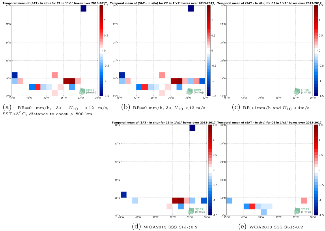
Figure 12: Temporal mean gridded over spatial boxes of size 1^\circ \times 1^\circ of \Delta SSS (SMOS-L2-DPGS-v662 - TSG-GOSUD-Sailing-ship) for 5 different subdatasets corresponding to: RR=0 mm/h, 3 < U_{10} < 12 m/s, SST > 5^\circ C , distance to coast > 800 km (a), RR=0 mm/h, 3 < U_{10} < 12 m/s (b), RR > 1 mm/h and U_{10} < 4 m/s (c), WOA2013 SSS Std <0.2 (d), WOA2013 SSS Std >0.2 (e).
