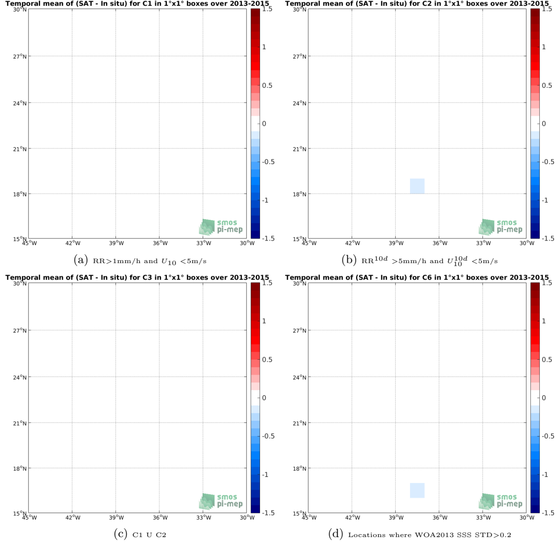
Figure 12: Temporal mean gridded over spatial boxes of size 1^\circ \times 1^\circ of \Delta SSS (SMOS-L2-DPGS-v662 - TSG-GOSUD-Sailing-ship) for 4 different subdatasets corresponding to: RR > 1 mm/h and U_{10} < 5 m/s (a), RR 10d > 5 mm/h and U_{10}^{10d} < 5 m/s (b), C1 U C2 (c), Locations where WOA2013 SSS STD > 0.2 (d).
