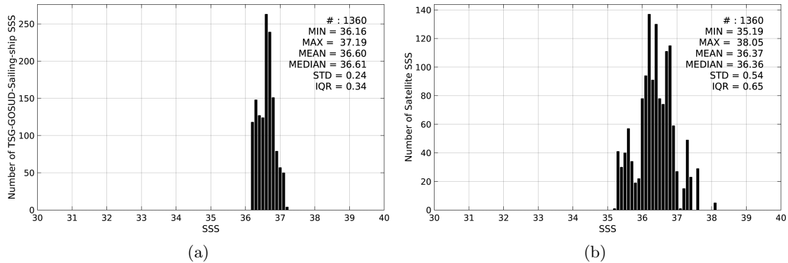
Figure 2: Histograms of SSS from TSG-GOSUD-Sailing-ship (a) and SMOS-L2-DPGS-v662 (b) considering all match-up pairs per bins of 0.1 over the SPURS 1 Pi-MEP region and for the full satellite product period.
