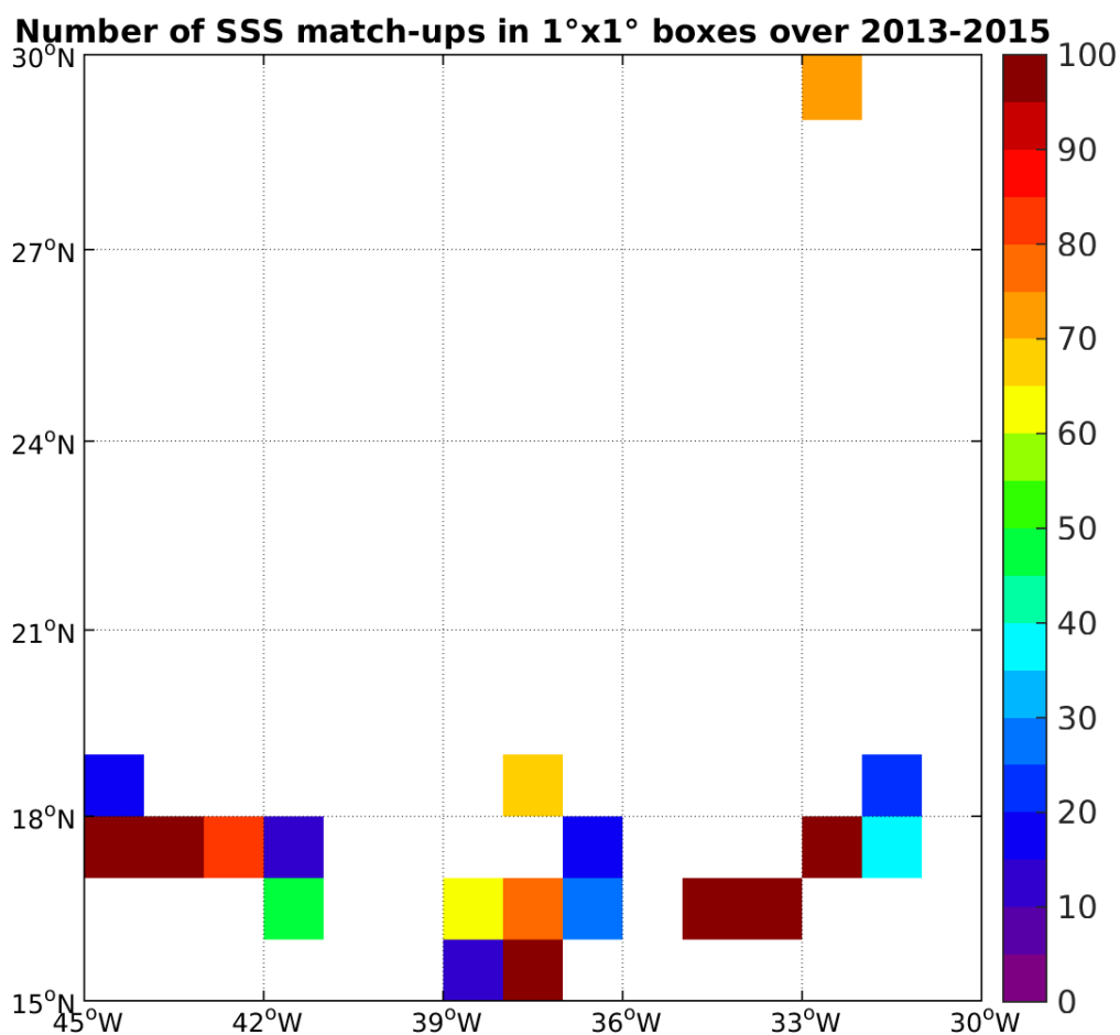
Figure 4: Number of SSS match-ups between TSG-GOSUD-Sailing-ship SSS and the SMOS-L2-DPGS-v662 SSS product for the SPURS 1 Pi-MEP region over 1°x1° boxes and for the full satellite product period.
