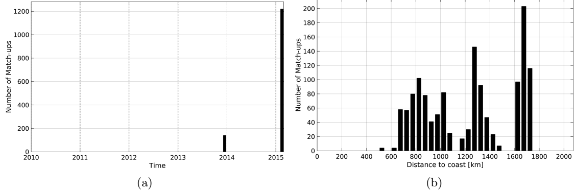
Figure 1: Number of match-ups between TSG-GOSUD-Sailing-ship and SMOS-L2-DPGS-v662 SSS as a function of time (a) and as function of the distance to coast (b) over the SPURS 1 Pi-MEP region and for the full satellite product period.
