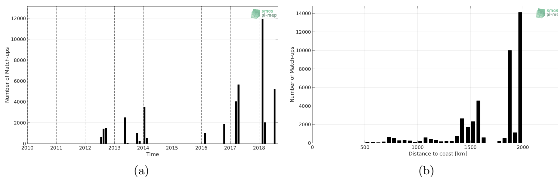
Figure 1: Number of match-ups between TSG-GOSUD-Research-vessel and SMOS L2 v662 (ESA) SSS as a function of time (a) and as function of the distance to coast (b) over the SPURS 1 Pi-MEP region and for the full satellite product period.
