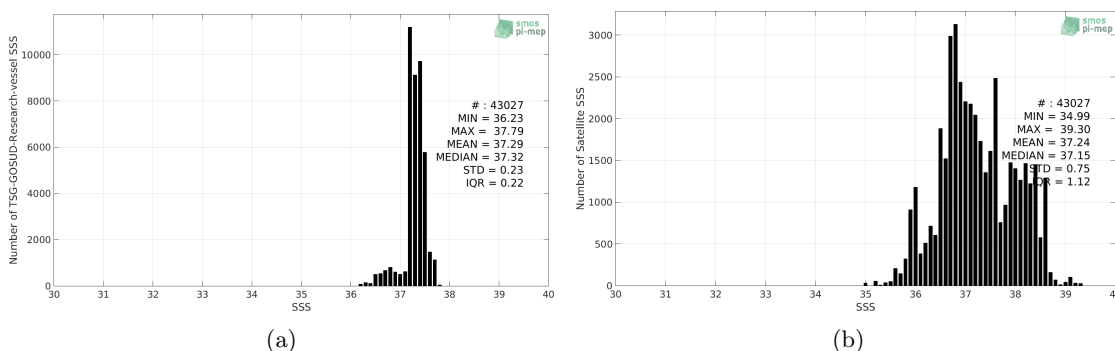
Figure 2: Histograms of SSS from TSG-GOSUD-Research-vessel (a) and SMOS L2 v662 (ESA) (b) considering all match-up pairs per bins of 0.1 over the SPURS 1 Pi-MEP region and for the full satellite product period.
