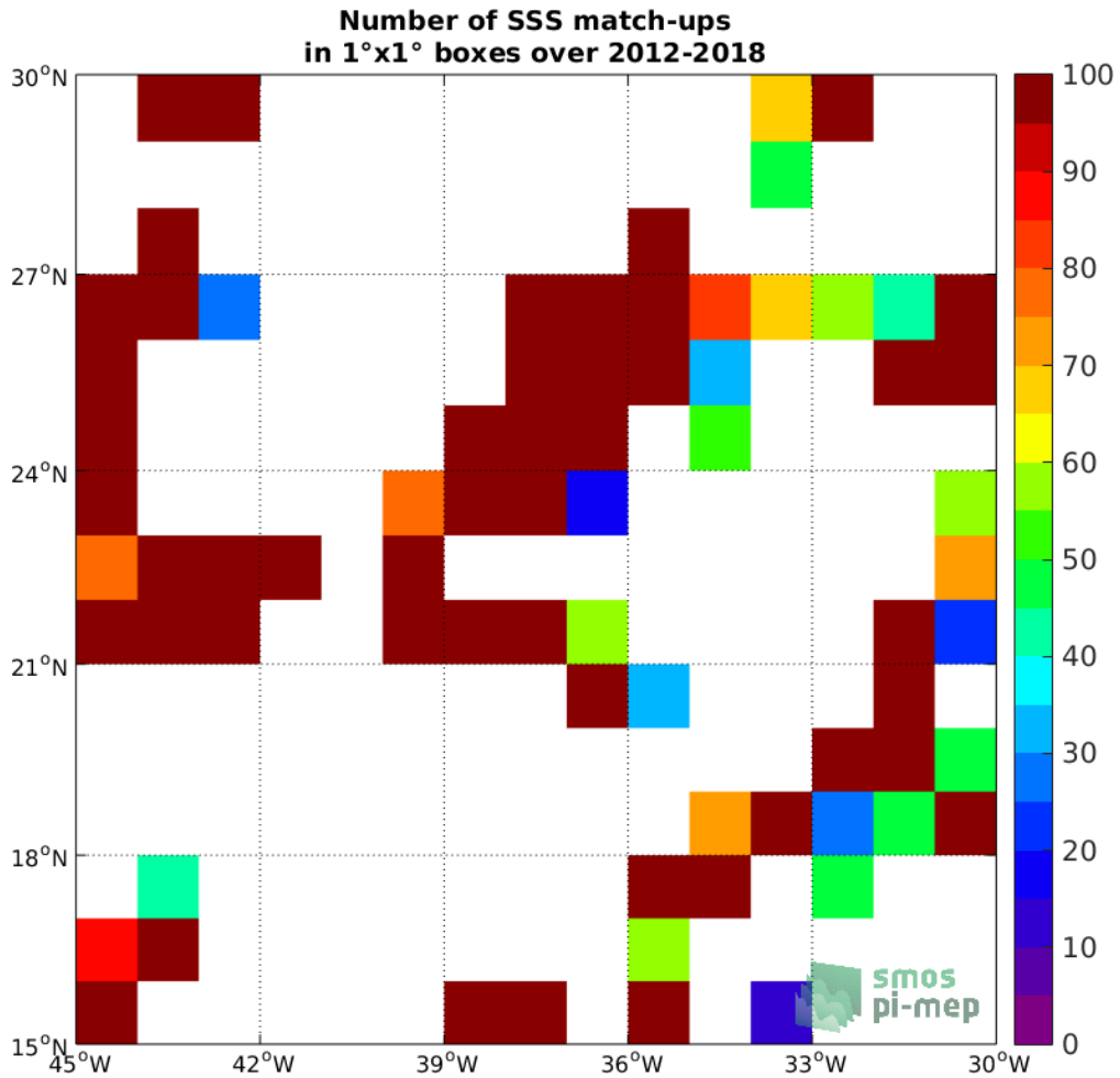
Figure 4: Number of SSS match-ups between TSG-GOSUD-Research-vessel SSS and the SMOS L2 v662 (ESA) SSS product for the SPURS 1 Pi-MEP region over 1°x1° boxes and for the full satellite product period.
