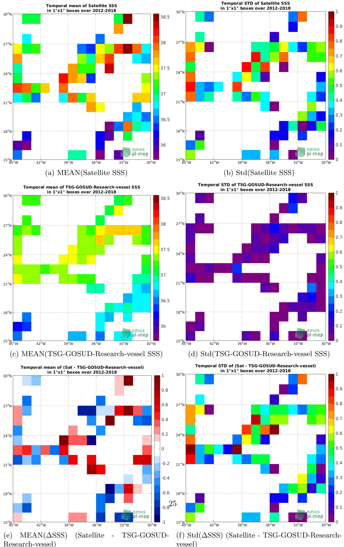
Figure 6: Temporal mean (left) and Std (right) of SSS from SMOS L2 v662 (ESA) (top), TSG-GOSUD-Research-vessel (middle), and of \Delta SSS (Satellite - TSG-GOSUD-Research-vessel). Only match-up pairs are used to generate these maps.
