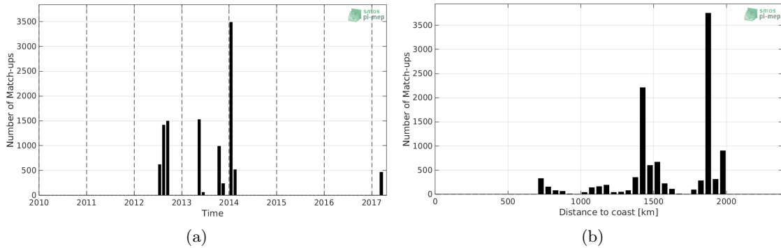
Figure 1: Number of match-ups between TSG-GOSUD-Research-vessel and SMOS-L2-DPGS-v662 SSS as a function of time (a) and as function of the distance to coast (b) over the SPURS 1 Pi-MEP region and for the full satellite product period.
