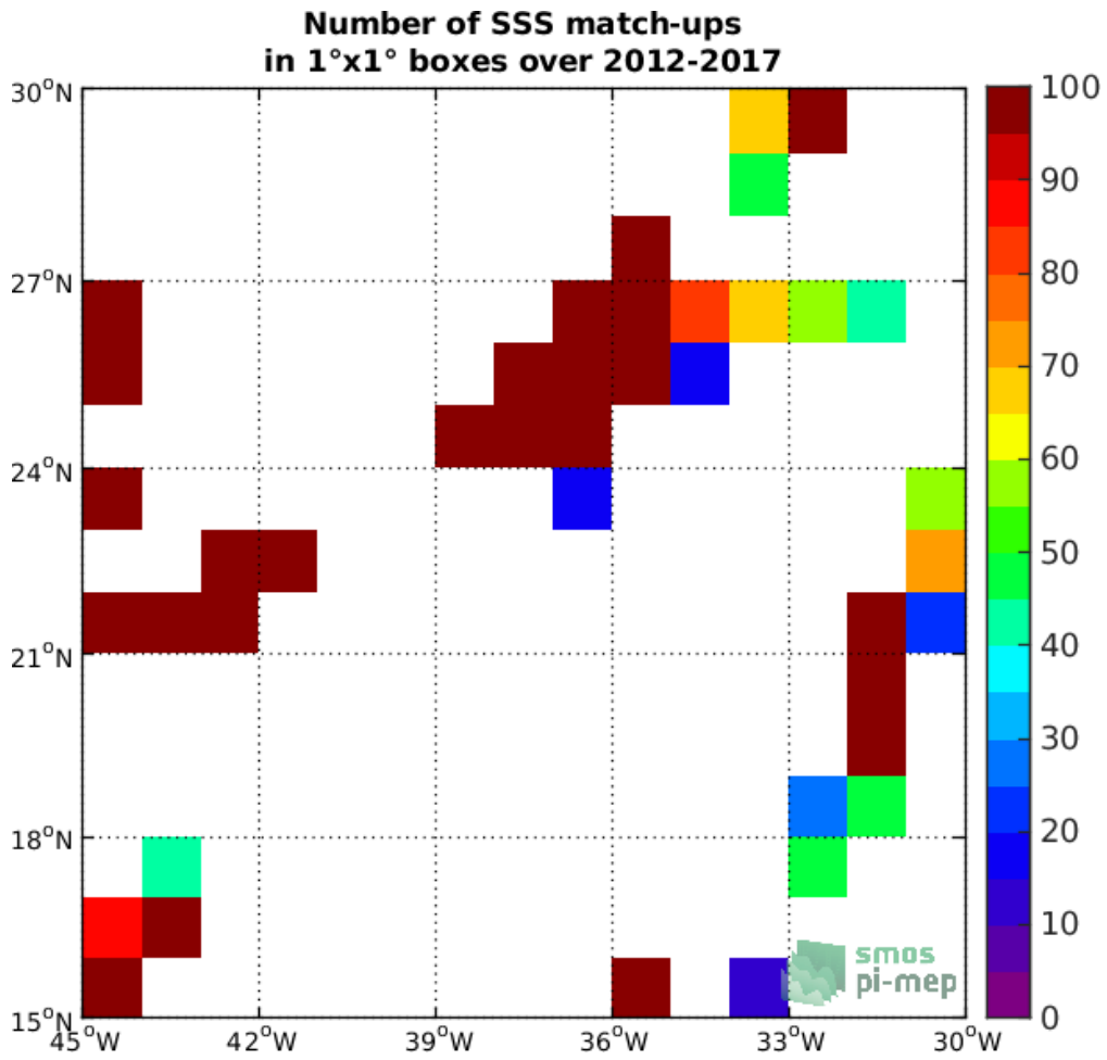
Figure 4: Number of SSS match-ups between TSG-GOSUD-Research-vessel SSS and the SMOS-L2-DPGS-v662 SSS product for the SPURS 1 Pi-MEP region over 1°x1° boxes and for the full satellite product period.
