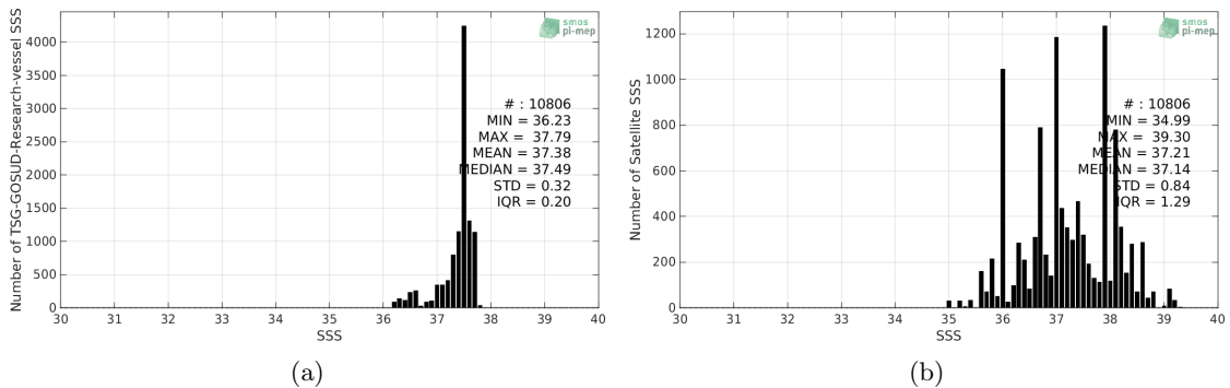
Figure 2: Histograms of SSS from TSG-GOSUD-Research-vessel (a) and SMOS-L2-DPGS-v662 (b) considering all match-up pairs per bins of 0.1 over the SPURS 1 Pi-MEP region and for the full satellite product period.
