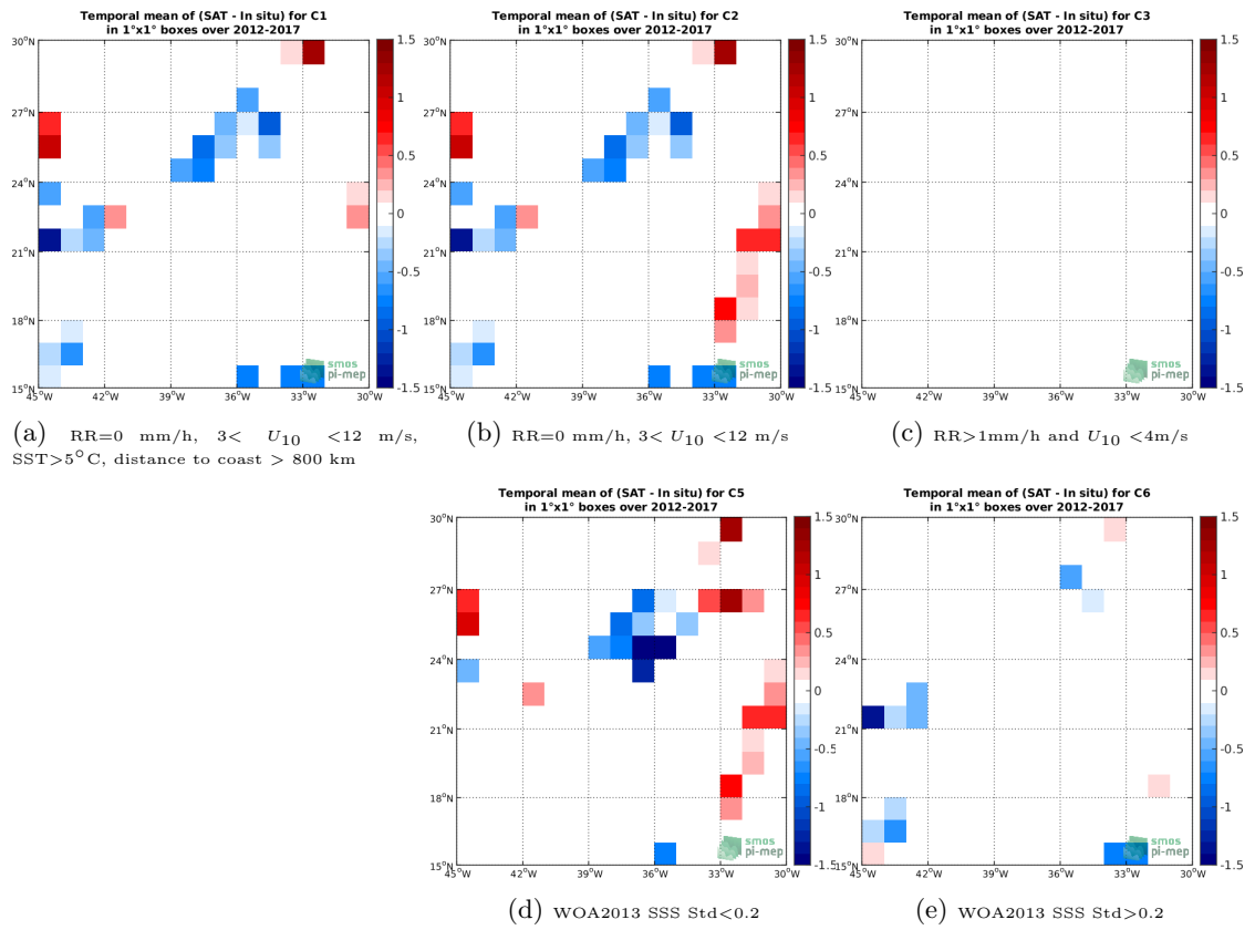
Figure 12: Temporal mean gridded over spatial boxes of size 1^\circ \times 1^\circ of \Delta SSS (SMOS-L2-DPGS-v662 - TSG-GOSUD-Research-vessel) for 5 different subdatasets corresponding to:RR=0 mm/h, 3 < U_{10} < 12 m/s, SST > 5^\circ\text{C} , distance to coast > 800 km (a), RR=0 mm/h, 3 < U_{10} < 12 m/s (b), RR > 1 mm/h and U_{10} < 4 m/s (c), WOA2013 SSS Std < 0.2 (d), WOA2013 SSS Std > 0.2 (e).
