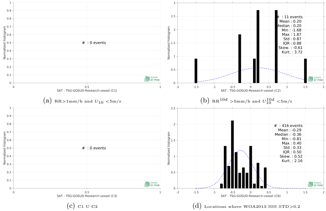
Figure 13: Normalized histogram of \Delta SSS (SMOS-L2-DPGS-v662 - TSG-GOSUD-Research-vessel) for 6 different subdatasets corresponding to: RR > 1\text{mm/h} and U_{10} < 5\text{m/s} (a), RR^{10d} > 5\text{mm/h} and U_{10}^{10d} < 5\text{m/s} (b), C1 \cup C2 (c), Locations where WOA2013 SSS STD > 0.2 (d).
