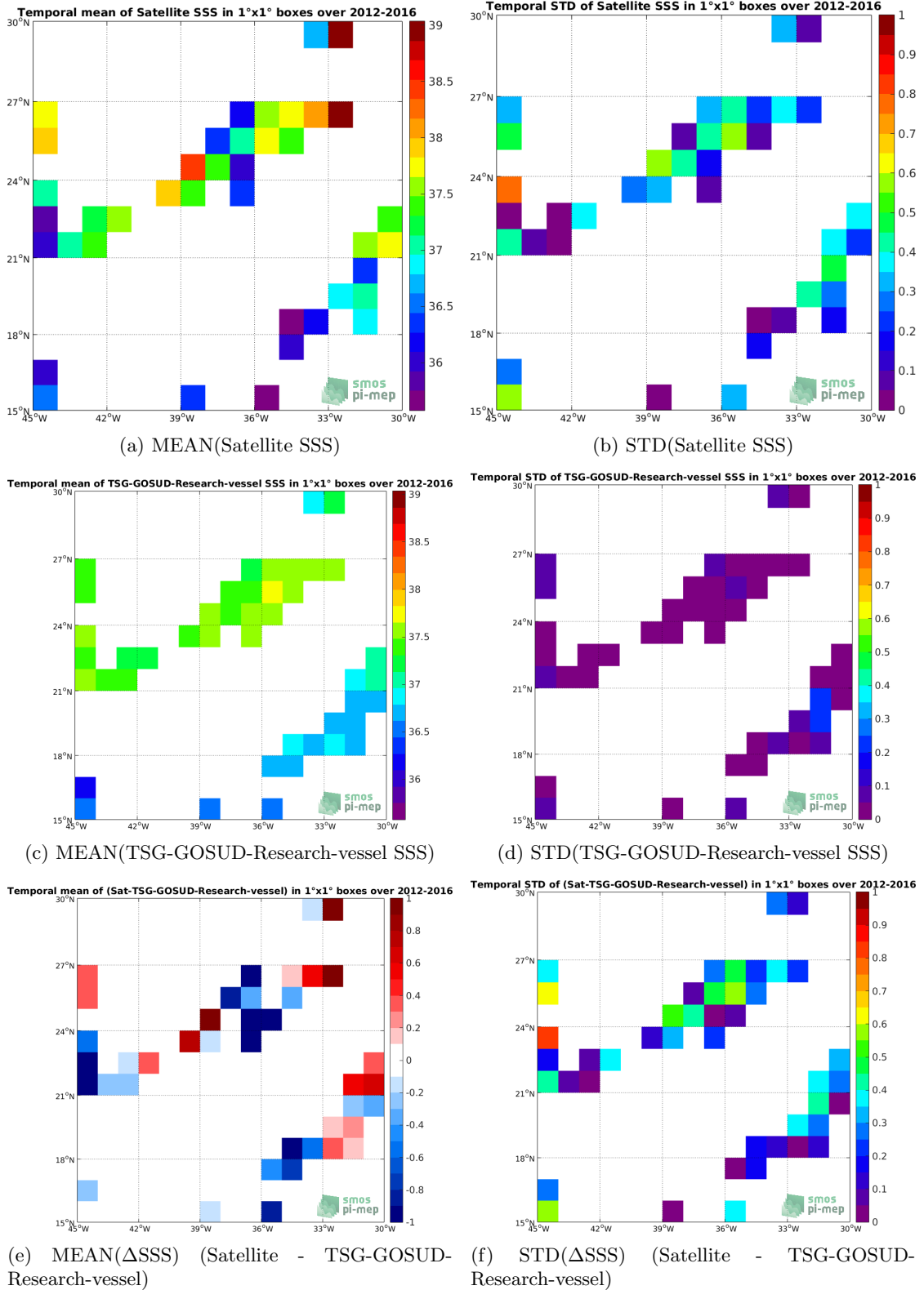
Figure 6: Temporal mean (left) and STD (right) of SSS from SMOS-L2-DPGS-v662 (top), TSG-GOSUD-Research-vessel (middle), and of \Delta SSS (Satellite - TSG-GOSUD-Research-vessel). Only match-up pairs are used to generate these maps.
