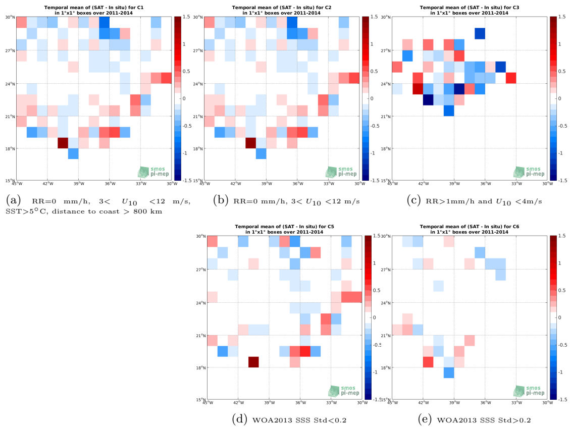
Figure 11: Temporal mean gridded over spatial boxes of size 1^\circ \times 1^\circ of \Delta\text{SSS} (SMOS SSS L2 v662 (ESA) - Surface drifters) for 5 different subdatasets corresponding to:RR=0 mm/h, 3 < U_{10} < 12 m/s, SST >5^\circ\text{C} , distance to coast > 800 km (a), RR=0 mm/h, 3 < U_{10} < 12 m/s (b), RR >1 mm/h and U_{10} < 4 m/s (c), WOA2013 SSS Std <0.2 (d), WOA2013 SSS Std >0.2 (e).
