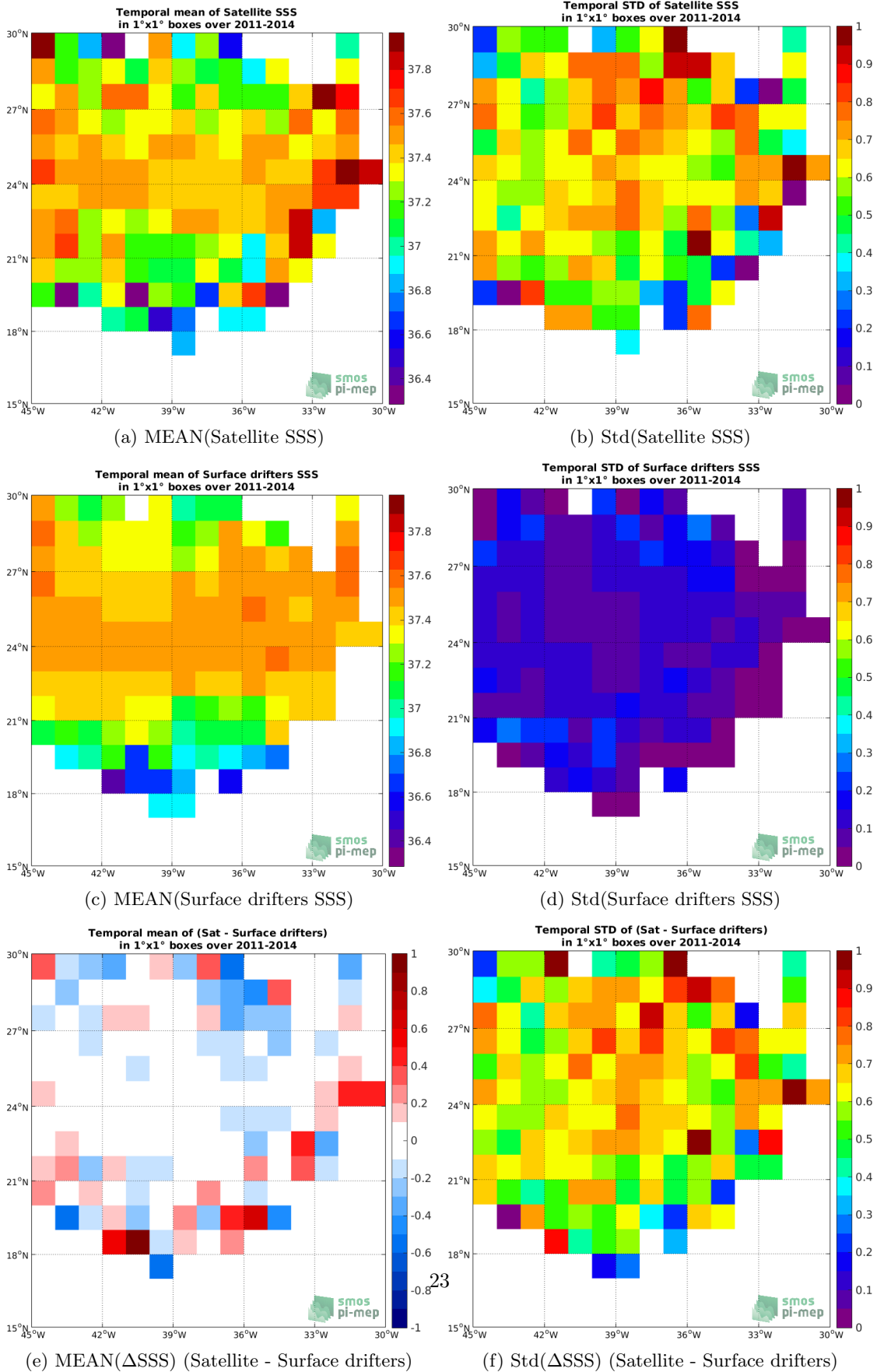
Figure 5: Temporal mean (left) and Std (right) of SSS from SMOS SSS L2 v662 (ESA) (top), Surface drifters (middle), and of \Delta SSS (Satellite - Surface drifters). Only match-up pairs are used to generate these maps.
