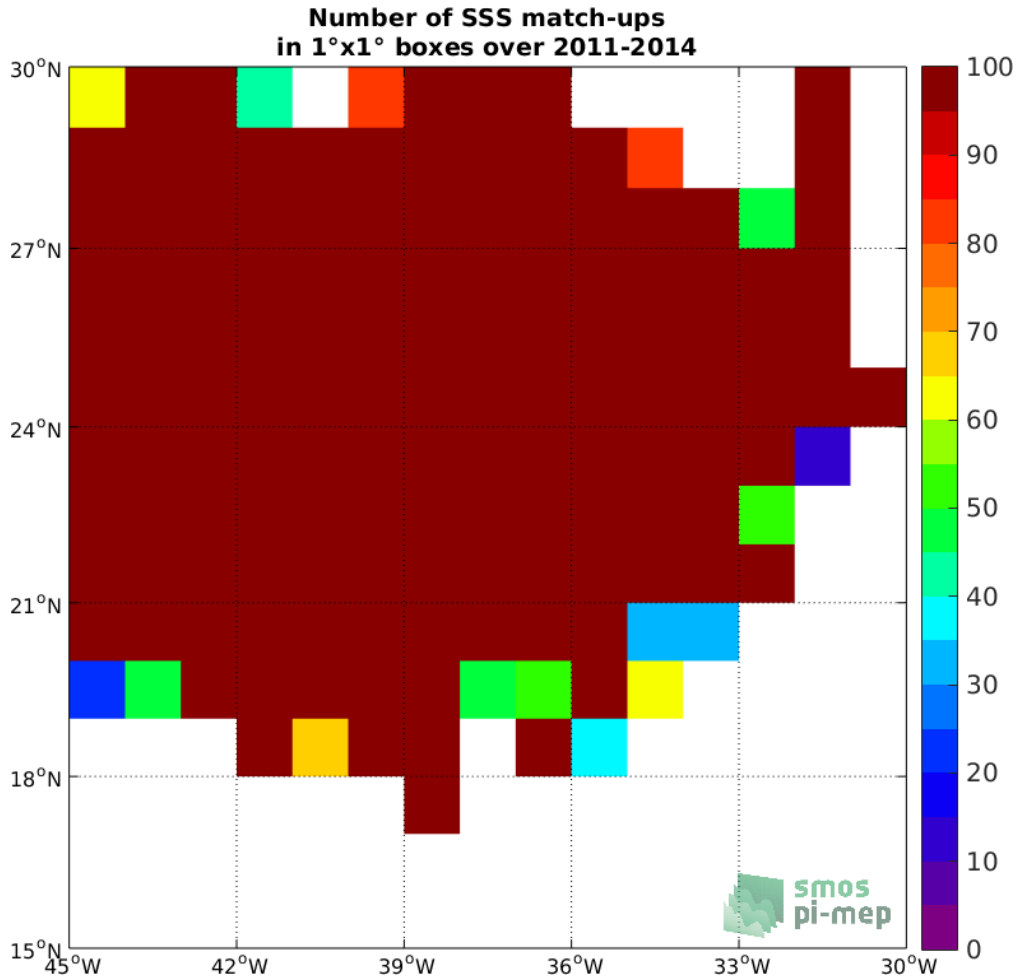
Figure 3: Number of SSS match-ups between Surface drifters SSS and the SMOS SSS L2 v662 (ESA) SSS product for the SPURS 1 Pi-MEP region over 1°x1° boxes and for the full satellite product period.
