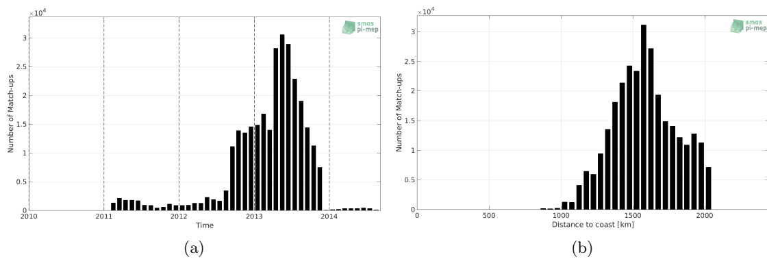
Figure 1: Number of match-ups between Surface drifters and SMOS SSS L2 v662 (ESA) SSS as a function of time (a) and as function of the distance to coast (b) over the SPURS 1 Pi-MEP region and for the full satellite product period.
