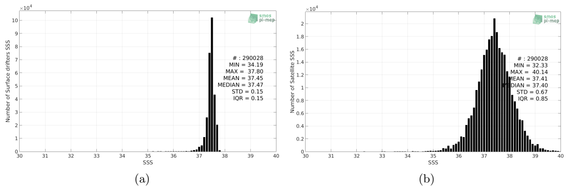
Figure 2: Histograms of SSS from Surface drifters (a) and SMOS SSS L2 v662 (ESA) (b) considering all match-up pairs per bins of 0.1 over the SPURS 1 Pi-MEP region and for the full satellite product period.
