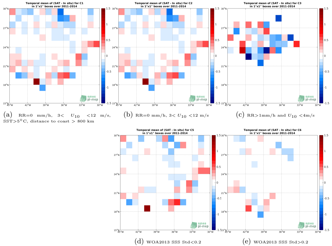
Figure 11: Temporal mean gridded over spatial boxes of size 1^\circ \times 1^\circ of \Delta SSS (SMOS L2 v662 (ESA) - Surface drifters) for 5 different subdatasets corresponding to:RR=0 mm/h, 3 < U_{10} < 12 m/s, SST > 5^\circ\text{C} , distance to coast > 800 km (a), RR=0 mm/h, 3 < U_{10} < 12 m/s (b), RR > 1 mm/h and U_{10} < 4 m/s (c), WOA2013 SSS Std < 0.2 (d), WOA2013 SSS Std > 0.2 (e).
