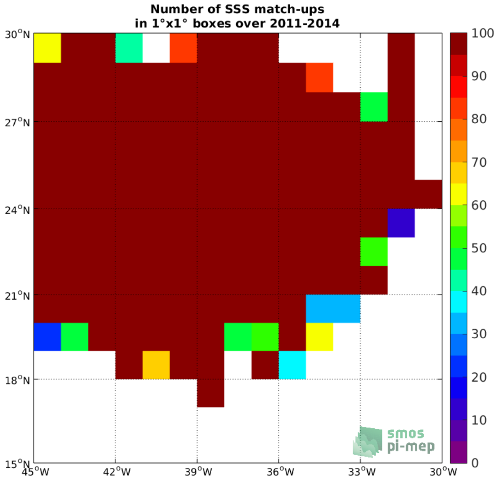
Figure 3: Number of SSS match-ups between Surface drifters SSS and the SMOS L2 v662 (ESA) SSS product for the SPURS 1 Pi-MEP region over 1°x1° boxes and for the full satellite product period.
