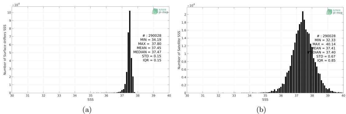
Figure 2: Histograms of SSS from Surface drifters (a) and SMOS L2 v662 (ESA) (b) considering all match-up pairs per bins of 0.1 over the SPURS 1 Pi-MEP region and for the full satellite product period.
