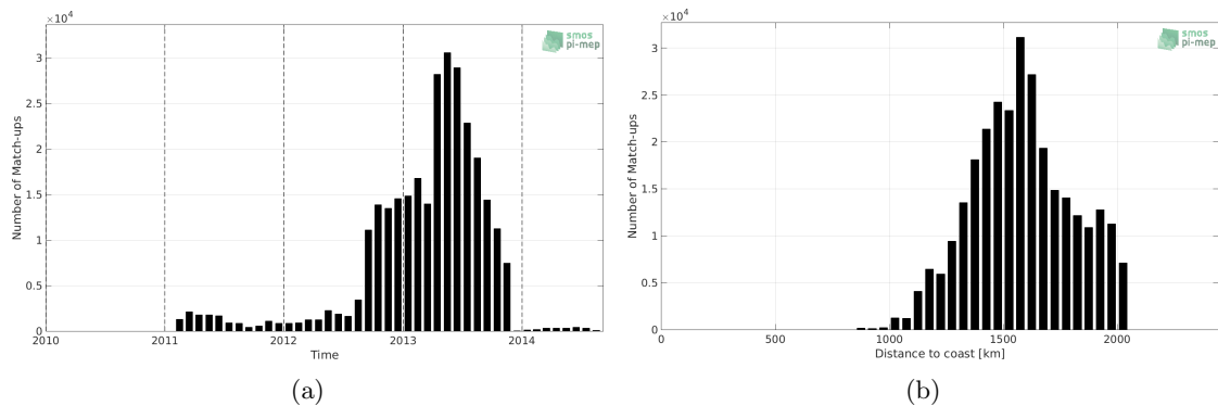
Figure 1: Number of match-ups between Surface drifters and SMOS L2 v662 (ESA) SSS as a function of time (a) and as function of the distance to coast (b) over the SPURS 1 Pi-MEP region and for the full satellite product period.
