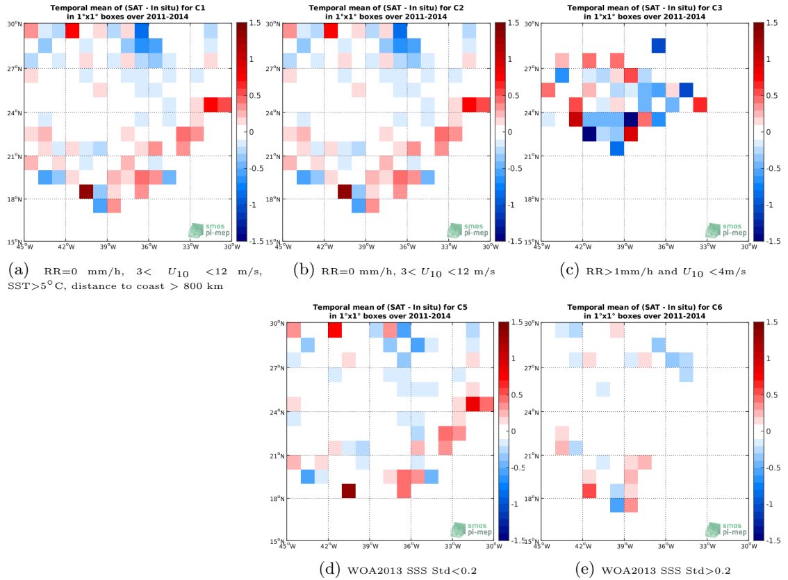
Figure 11: Temporal mean gridded over spatial boxes of size 1^\circ \times 1^\circ of \Delta\text{SSS} (SMOS-L2-DPGS-v662 - Surface drifters) for 5 different subdatasets corresponding to:RR=0 mm/h, 3 < U_{10} < 12 m/s, SST >5^\circ\text{C} , distance to coast > 800 km (a), RR=0 mm/h, 3 < U_{10} < 12 m/s (b), RR >1 mm/h and U_{10} < 4 m/s (c), WOA2013 SSS Std <0.2 (d), WOA2013 SSS Std >0.2 (e).
