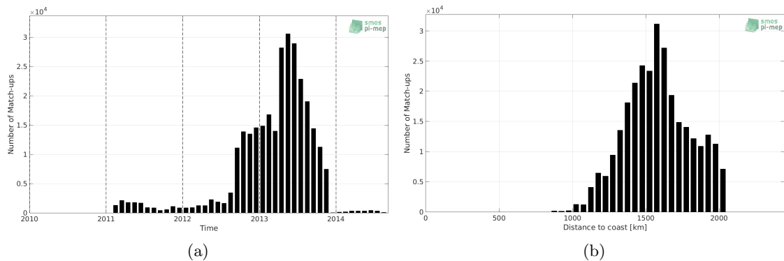
Figure 1: Number of match-ups between Surface drifters and SMOS-L2-DPGS-v662 SSS as a function of time (a) and as function of the distance to coast (b) over the SPURS 1 Pi-MEP region and for the full satellite product period.
