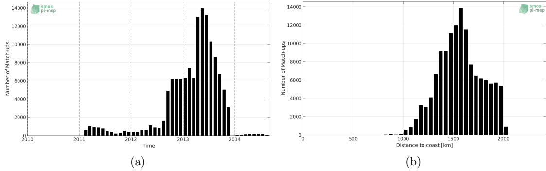
Figure 1: Number of match-ups between Surface drifters and SMOS-L2-DPGS-v662 SSS as a function of time (a) and as function of the distance to coast (b) over the SPURS 1 Pi-MEP region and for the full satellite product period.
