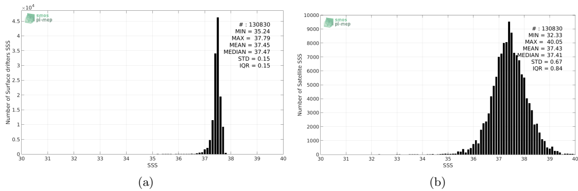
Figure 2: Histograms of SSS from Surface drifters (a) and SMOS-L2-DPGS-v662 (b) considering all match-up pairs per bins of 0.1 over the SPURS 1 Pi-MEP region and for the full satellite product period.
