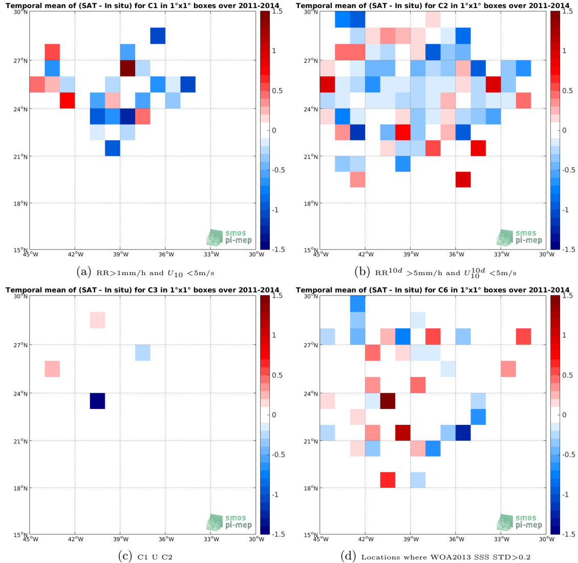
Figure 11: Temporal mean gridded over spatial boxes of size 1^\circ \times 1^\circ of \Delta SSS (SMOS-L2-DPGS-v662 - Surface drifters) for 4 different subdatasets corresponding to: RR > 1\text{mm/h} and U_{10} < 5\text{m/s} (a), RR^{10d} > 5\text{mm/h} and U_{10}^{10d} < 5\text{m/s} (b), C1 U C2 (c), Locations where WOA2013 SSS STD > 0.2 (d).
