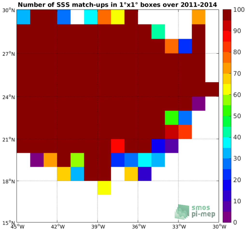
Figure 3: Number of SSS match-ups between Surface drifters SSS and the SMOS-L2-DPGS-v662 SSS product for the SPURS 1 Pi-MEP region over 1°x1° boxes and for the full satellite product period.
