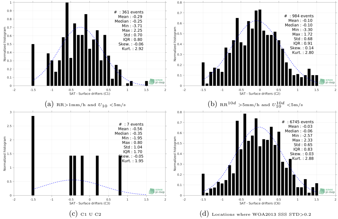
Figure 12: Normalized histogram of \Delta SSS (SMOS-L2-DPGS-v662 - Surface drifters) for 6 different subdatasets corresponding to: RR > 1\text{mm/h} and U_{10} < 5\text{m/s} (a), RR^{10d} > 5\text{mm/h} and U_{10}^{10d} < 5\text{m/s} (b), C1 U C2 (c), Locations where WOA2013 SSS STD > 0.2 (d).
