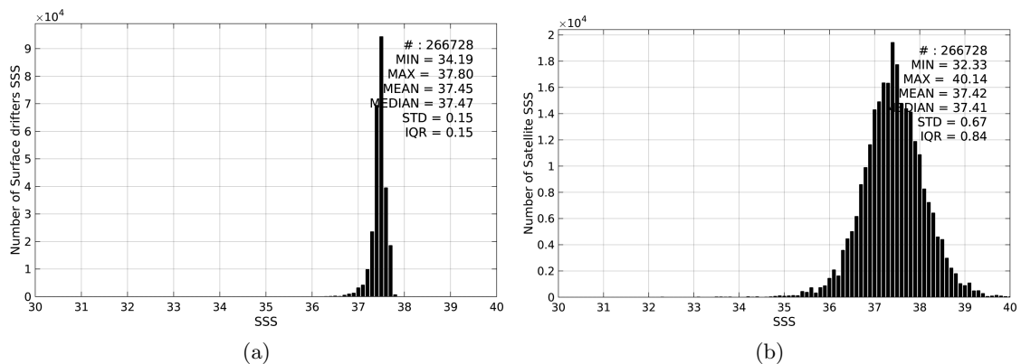
Figure 2: Histograms of SSS from Surface drifters (a) and SMOS-L2-DPGS-v662 (b) considering all match-up pairs per bins of 0.1 over the SPURS 1 Pi-MEP region and for the full satellite product period.
