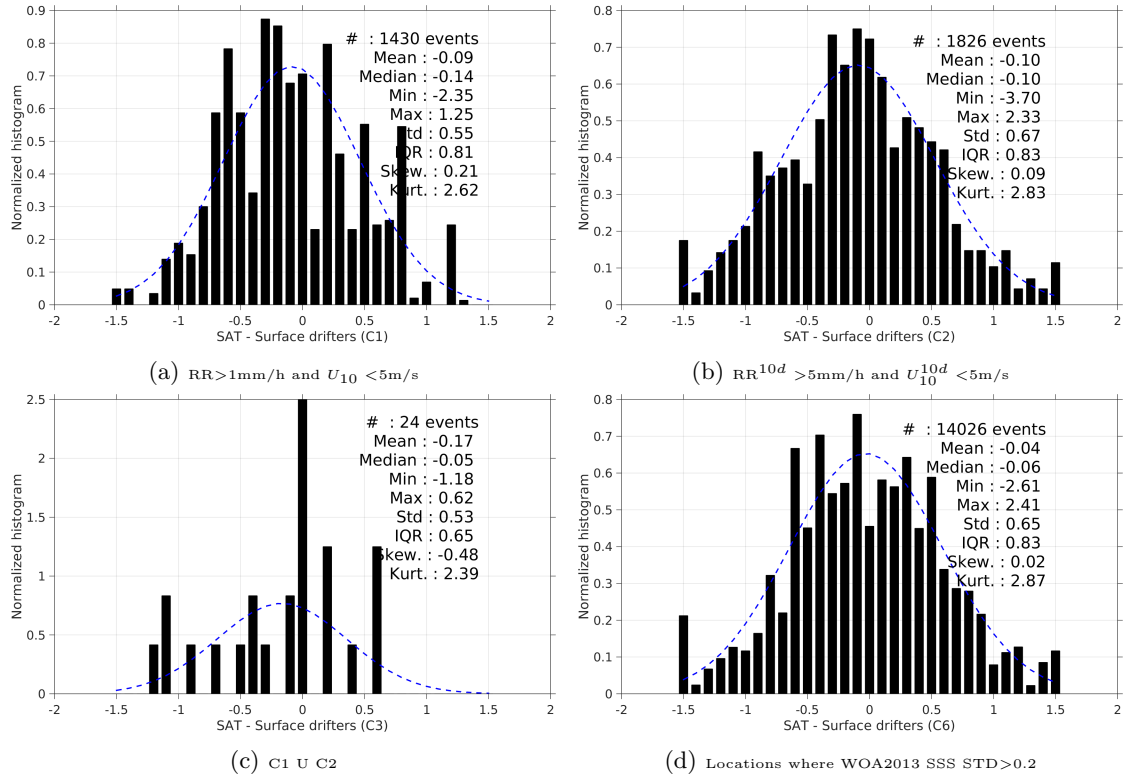
Figure 12: Normalized histogram of \Delta SSS (SMOS-L2-DPGS-v662 - Surface drifters) for 6 different subdatasets corresponding to: RR > 1mm/h and U_{10} < 5 m/s (a), RR^{10d} > 5 mm/h and U_{10}^{10d} < 5 m/s (b), C1 U C2 (c), Locations where WOA2013 SSS STD > 0.2 (d).
