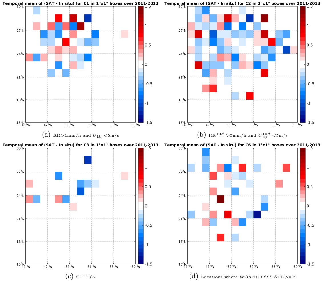
Figure 11: Temporal mean gridded over spatial boxes of size 1°x1° of \Delta SSS (SMOS-L2-DPGS-v662 - Surface drifters) for 4 different subdatasets corresponding to: RR > 1\text{mm/h} and U_{10} < 5\text{m/s} (a), RR^{10d} > 5\text{mm/h} and U_{10}^{10d} < 5\text{m/s} (b), C1 U C2 (c), Locations where WOA2013 SSS STD > 0.2 (d).
