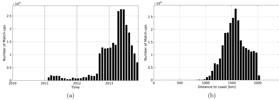
Figure 1: Number of match-ups between Surface drifters and SMOS-L2-DPGS-v662 SSS as a function of time (a) and as function of the distance to coast (b) over the SPURS 1 Pi-MEP region and for the full satellite product period.
