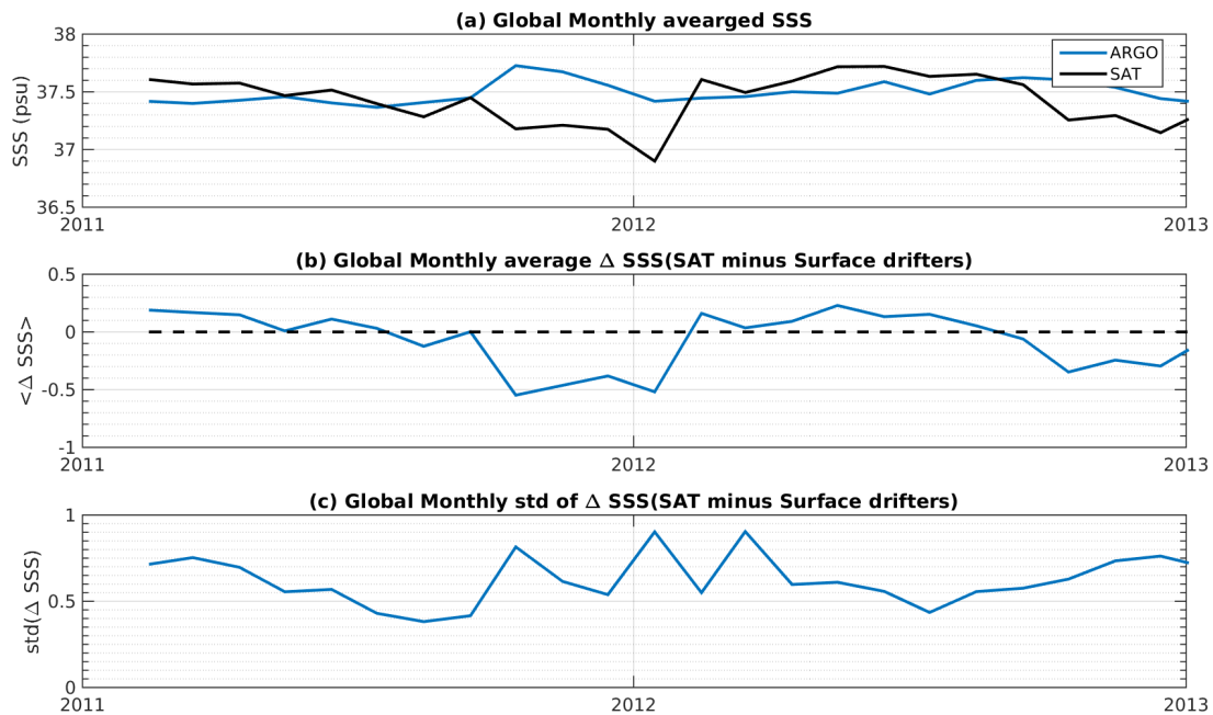
Figure 6: Time series of the monthly averaged mean SSS (top), mean \Delta SSS (Satellite - Surface drifters) and STD of \Delta SSS (Satellite - Surface drifters) over the SPURS 1 Pi-MEP region considering all match-ups collected by the Pi-MEP platform.
