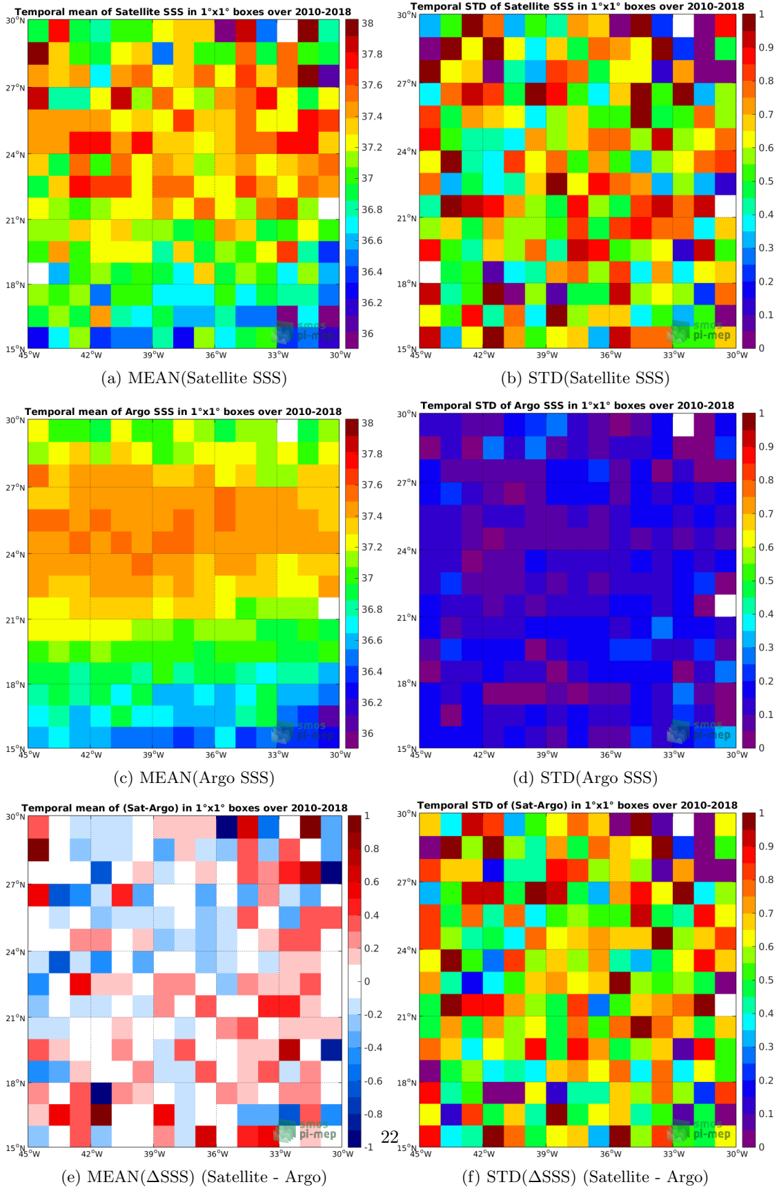
Figure 6: Temporal mean (left) and STD (right) of SSS from SMOS-L2-DPGS-v662 (top), Argo (middle), and of \Delta SSS (Satellite - Argo). Only match-up pairs are used to generate these maps.
