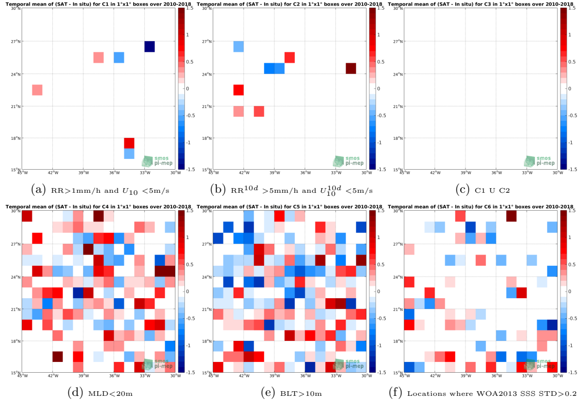
Figure 12: Temporal mean gridded over spatial boxes of size 1^\circ \times 1^\circ of \Delta\text{SSS} (SMOS-L2-DPGS-v662 - Argo) for 6 different subdatasets corresponding to: \text{RR} > 1\text{mm/h} and U_{10} < 5\text{m/s} (a), \text{RR}^{10d} > 5\text{mm/h} and U_{10}^{10d} < 5\text{m/s} (b), C1 U C2 (c), \text{MLD} < 20\text{m} (d), \text{BLT} > 10\text{m} (e), Locations where WOA2013 SSS STD > 0.2 (f).
