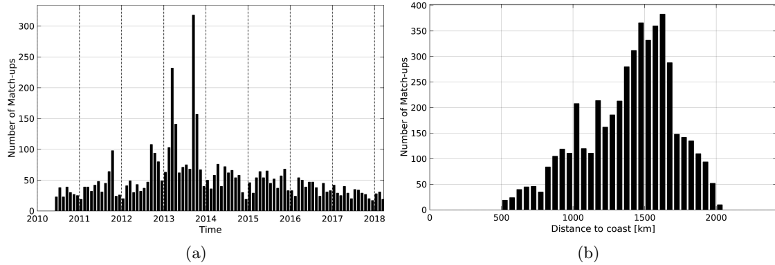
Figure 1: Number of match-ups between Argo and SMOS-L2-DPGS-v662 SSS as a function of time (a) and as function of the distance to coast (b) over the SPURS 1 Pi-MEP region and for the full satellite product period.
