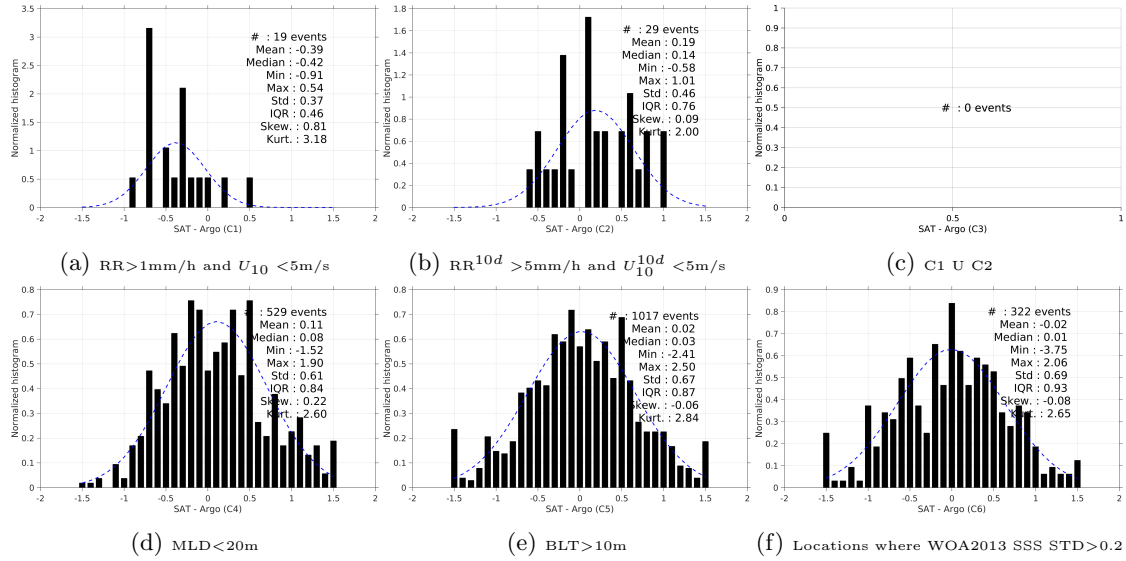
Figure 13: Normalized histogram of \Delta SSS (SMOS-L2-DPGS-v662 - Argo) for 6 different sub-datasets corresponding to: RR > 1mm/h and U_{10} < 5 m/s (a), RR 10d > 5mm/h and U_{10}^{10d} < 5 m/s (b), C1 U C2 (c), MLD < 20m (d), BLT > 10m (e), Locations where WOA2013 SSS STD > 0.2 (f).
