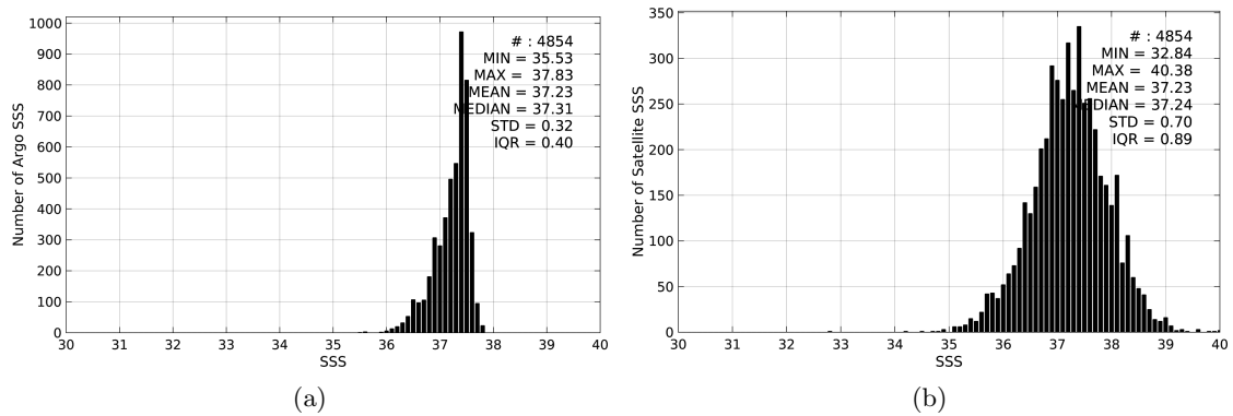
Figure 2: Histograms of SSS from Argo (a) and SMOS-L2-DPGS-v662 (b) considering all match-up pairs per bins of 0.1 over the SPURS 1 Pi-MEP region and for the full satellite product period.
