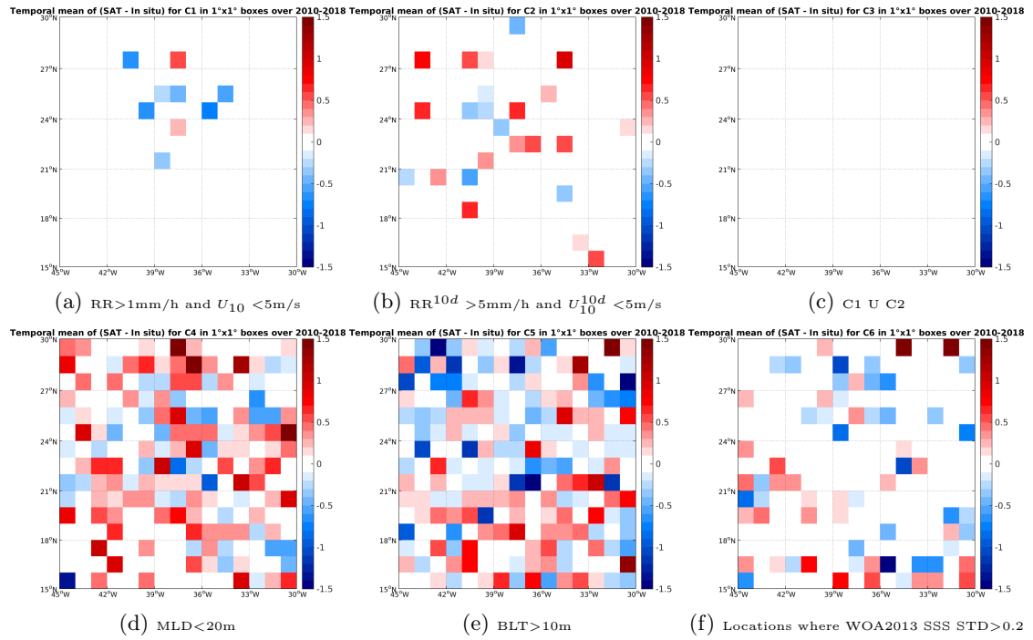
Figure 12: Temporal mean gridded over spatial boxes of size 1^\circ \times 1^\circ of \Delta\text{SSS} (SMOS-L2-DPGS-v662 - Argo) for 6 different subdatasets corresponding to: \text{RR} > 1\text{mm/h} and U_{10} < 5\text{m/s} (a), \text{RR}^{10d} > 5\text{mm/h} and U_{10}^{10d} < 5\text{m/s} (b), C1 U C2 (c), \text{MLD} < 20\text{m} (d), \text{BLT} > 10\text{m} (e), Locations where WOA2013 SSS STD > 0.2 (f).
