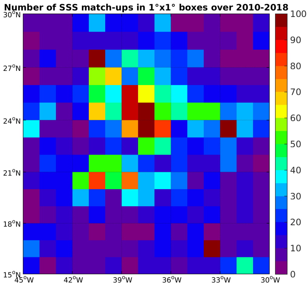
Figure 4: Number of SSS match-ups between Argo SSS and the SMOS-L2-DPGS-v662 SSS product for the SPURS 1 Pi-MEP region over 1°x1° boxes and for the full satellite product period.
