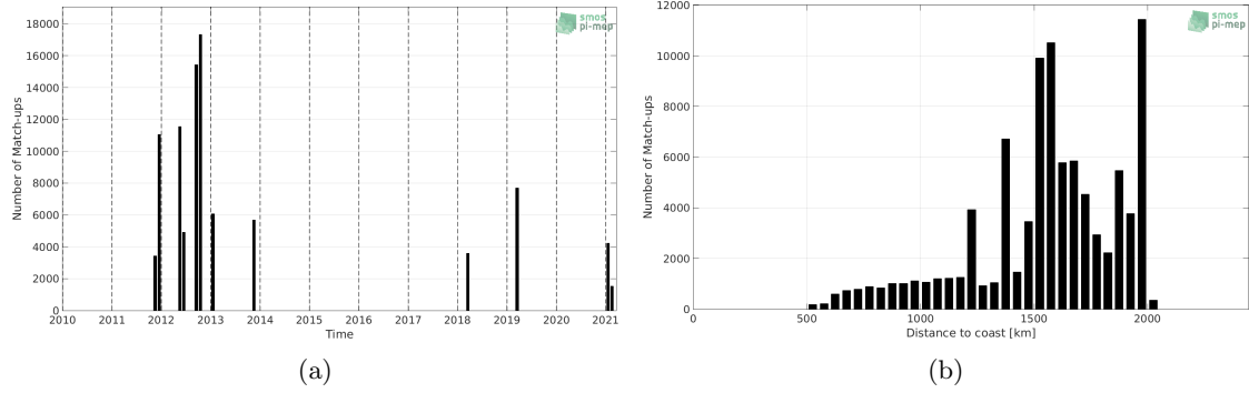
Figure 1: Number of match-ups between TSG (SAMOS) and SMAP SSS L4 OI v1 - 7day (IPRC) SSS as a function of time (a) and as function of the distance to coast (b) over the SPURS 1 Pi-MEP region and for the full satellite product period.
