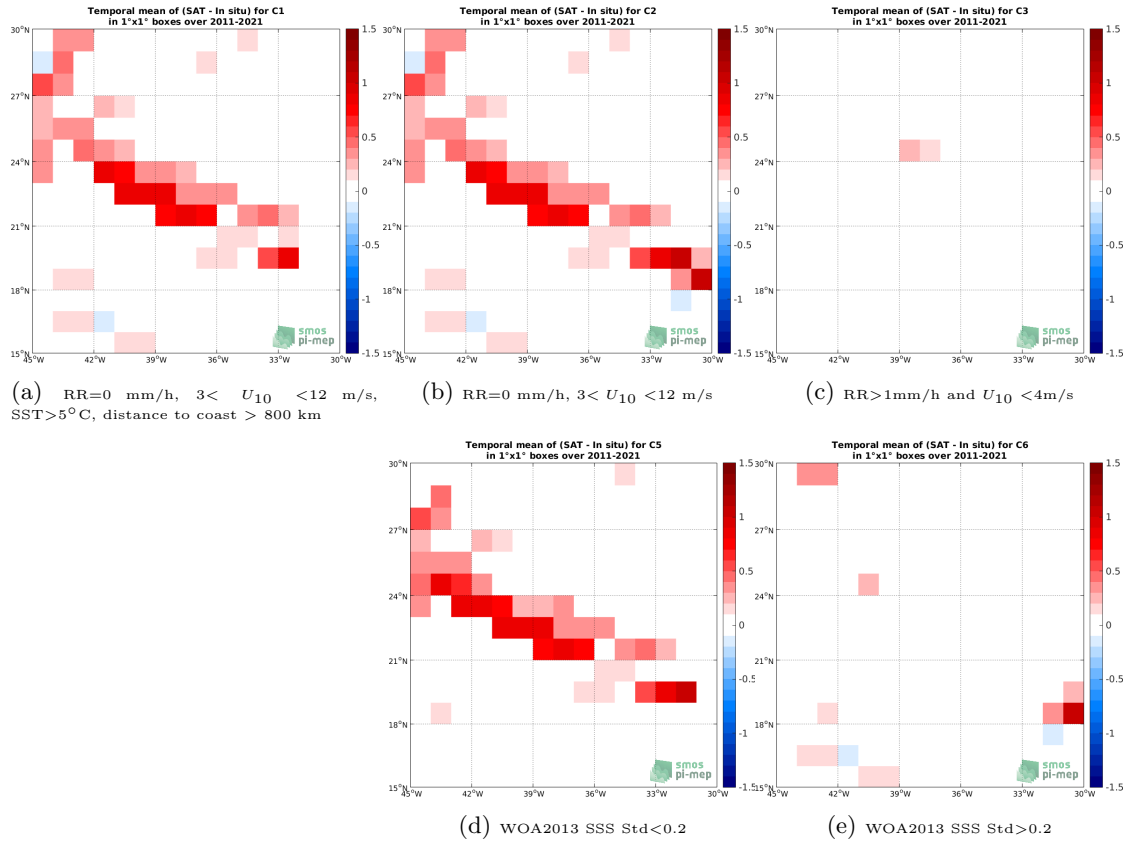
Figure 12: Temporal mean gridded over spatial boxes of size 1^\circ \times 1^\circ of \Delta SSS (SMAP SSS L4 OI v1 - 7day (IPRC) - TSG (SAMOS)) for 5 different subdatasets corresponding to: RR=0 mm/h, 3 < U_{10} < 12 m/s, SST > 5^\circ C , distance to coast > 800 km (a), RR=0 mm/h, 3 < U_{10} < 12 m/s (b), RR > 1 mm/h and U_{10} < 4 m/s (c), WOA2013 SSS Std < 0.2 (d), WOA2013 SSS Std > 0.2 (e).
