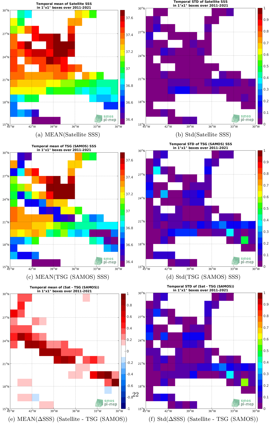
Figure 6: Temporal mean (left) and Std (right) of SSS from SMAP SSS L4 OI v1 - 7day (IPRC) (top), TSG (SAMOS) (middle), and of \Delta SSS (Satellite - TSG (SAMOS)). Only match-up pairs are used to generate these maps.
