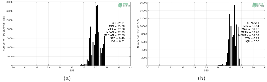
Figure 2: Histograms of SSS from TSG (SAMOS) (a) and SMAP SSS L4 OI v1 - 7day (IPRC) (b) considering all match-up pairs per bins of 0.1 over the SPURS 1 Pi-MEP region and for the full satellite product period.
