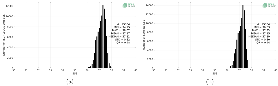
Figure 2: Histograms of SSS from TSG (LEGOS-DM) (a) and SMAP SSS L4 OI v1 - 7 Days (IPRC) (b) considering all match-up pairs per bins of 0.1 over the SPURS 1 Pi-MEP region and for the full satellite product period.
