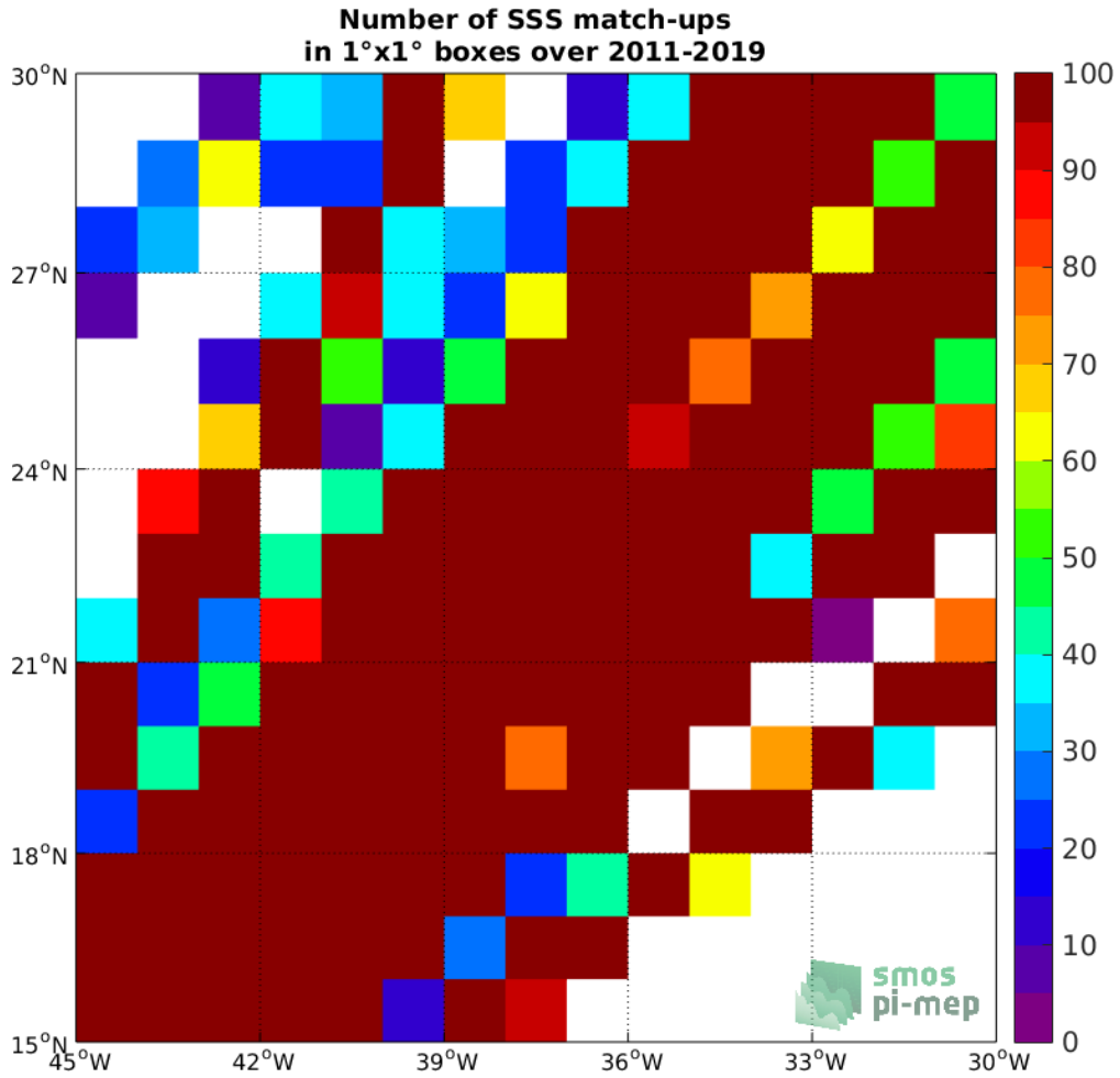
Figure 4: Number of SSS match-ups between TSG (LEGOS-DM) SSS and the SMAP SSS L4 OI v1 - 7 Days (IPRC) SSS product for the SPURS 1 Pi-MEP region over 1^\circ \times 1^\circ boxes and for the full satellite product period.
