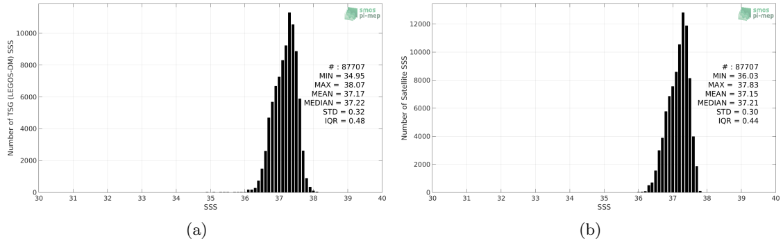
Figure 2: Histograms of SSS from TSG (LEGOS-DM) (a) and SMAP SSS L4 OI v1 - 7 Days (IPRC) (b) considering all match-up pairs per bins of 0.1 over the SPURS 1 Pi-MEP region and for the full satellite product period.
