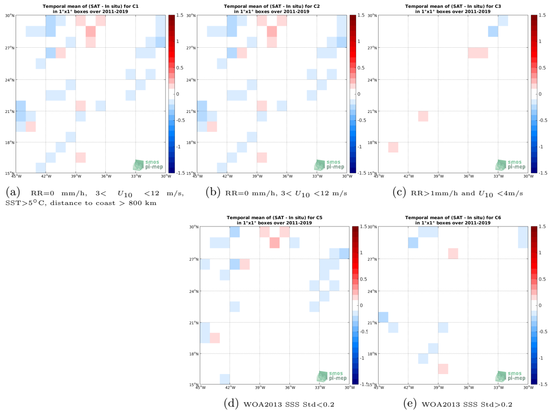
Figure 12: Temporal mean gridded over spatial boxes of size 1^\circ \times 1^\circ of \Delta SSS (SMAP SSS L4 OI v1 - 7 Days (IPRC) - TSG (LEGOS-DM)) for 5 different subdatasets corresponding to:RR=0 mm/h, 3 < U_{10} < 12 m/s, SST >5^\circ C, distance to coast > 800 km (a), RR=0 mm/h, 3 < U_{10} < 12 m/s (b), RR >1 mm/h and U_{10} < 4 m/s (c), WOA2013 SSS Std <0.2 (d), WOA2013 SSS Std >0.2 (e).
