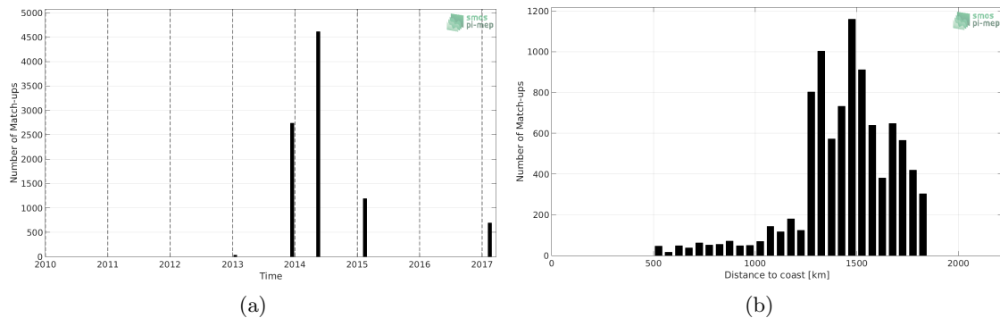
Figure 1: Number of match-ups between TSG (GOSUD-Sailing-ship) and SMAP SSS L4 OI v1 - 7 Days (IPRC) SSS as a function of time (a) and as function of the distance to coast (b) over the SPURS 1 Pi-MEP region and for the full satellite product period.
