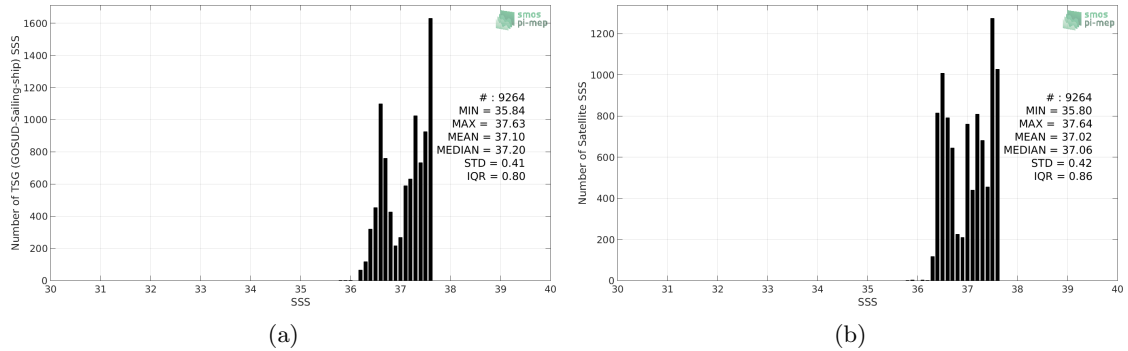
Figure 2: Histograms of SSS from TSG (GOSUD-Sailing-ship) (a) and SMAP SSS L4 OI v1 - 7 Days (IPRC) (b) considering all match-up pairs per bins of 0.1 over the SPURS 1 Pi-MEP region and for the full satellite product period.
