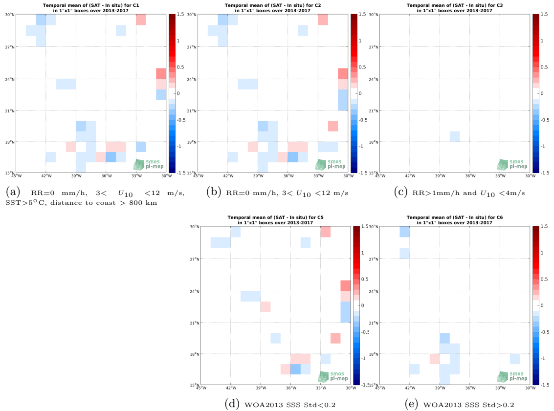
Figure 12: Temporal mean gridded over spatial boxes of size 1^\circ \times 1^\circ of \Delta\text{SSS} (SMAP SSS L4 OI v1 - 7 Days (IPRC) - TSG (GOSUD-Sailing-ship)) for 5 different subdatasets corresponding to:RR=0 mm/h, 3 < U_{10} < 12 m/s, SST>5°C, distance to coast > 800 km (a), RR=0 mm/h, 3 < U_{10} < 12 m/s (b), RR>1mm/h and U_{10} < 4 m/s (c), WOA2013 SSS Std<0.2 (d), WOA2013 SSS Std>0.2 (e).
