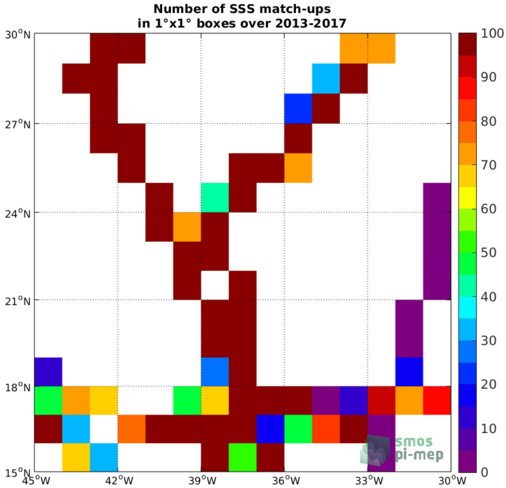
Figure 4: Number of SSS match-ups between TSG (GOSUD-Sailing-ship) SSS and the SMAP SSS L4 OI v1 - 7 Days (IPRC) SSS product for the SPURS 1 Pi-MEP region over 1°x1° boxes and for the full satellite product period.
