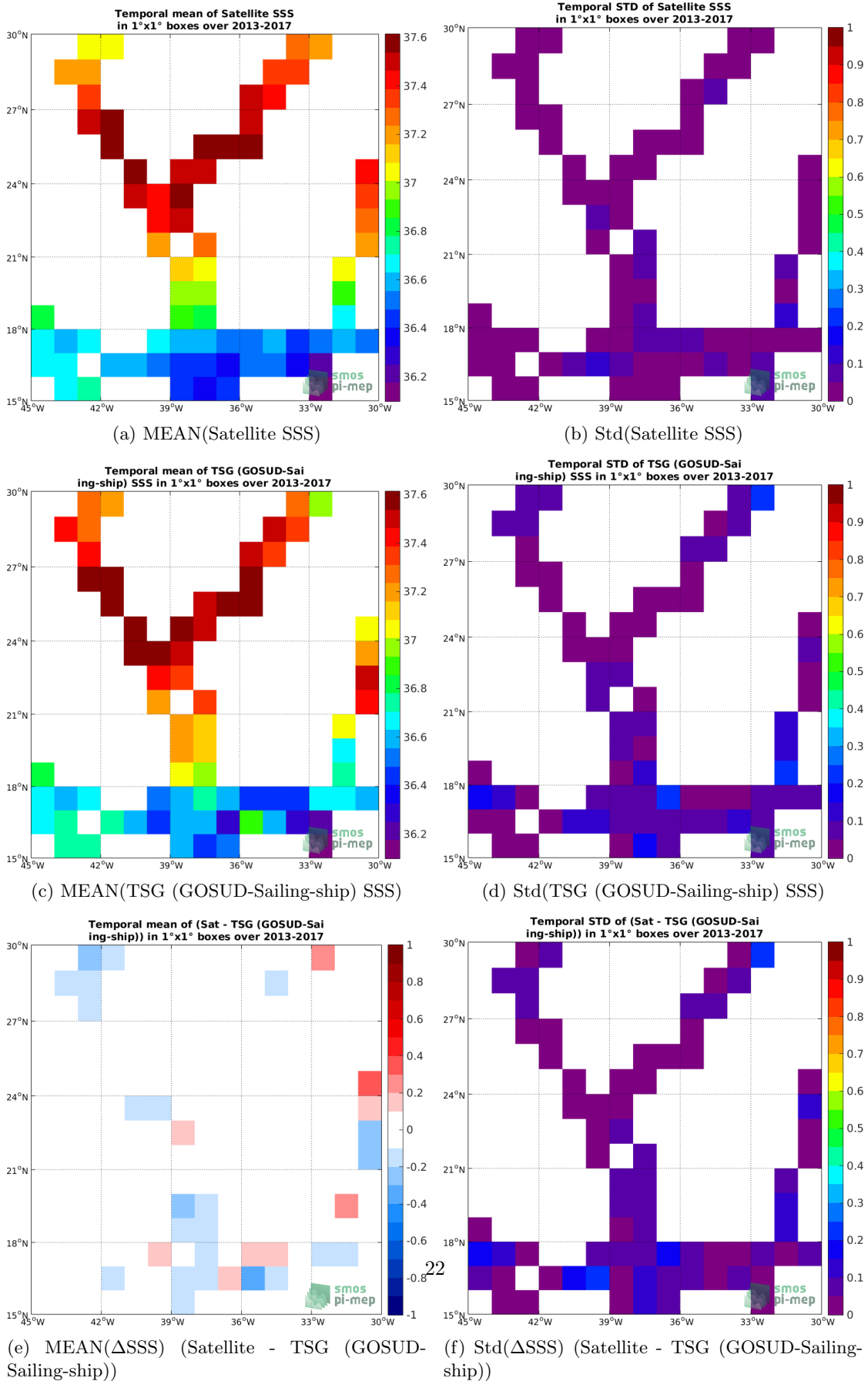
Figure 6: Temporal mean (left) and Std (right) of SSS from SMAP SSS L4 OI v1 - 7day (IPRC) (top), TSG (GOSUD-Sailing-ship) (middle), and of \Delta SSS (Satellite - TSG (GOSUD-Sailing-ship)). Only match-up pairs are used to generate these maps.
