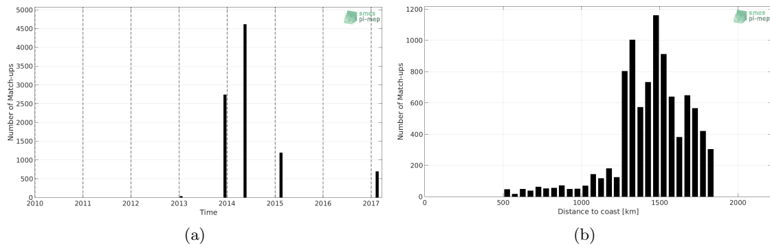
Figure 1: Number of match-ups between TSG (GOSUD-Sailing-ship) and SMAP SSS L4 OI v1 - 7day (IPRC) SSS as a function of time (a) and as function of the distance to coast (b) over the SPURS 1 Pi-MEP region and for the full satellite product period.
