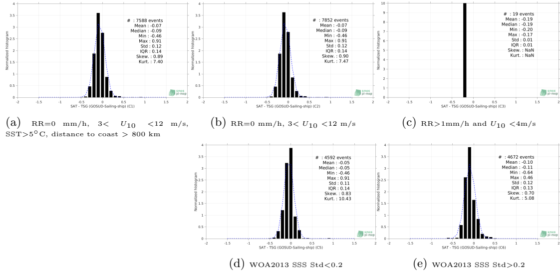
Figure 13: Normalized histogram of \Delta SSS (SMAP SSS L4 OI v1 - 7day (IPRC) - TSG (GOSUD-Sailing-ship)) for 5 different subdatasets corresponding to: RR=0 mm/h, 3 < U_{10} < 12 m/s, SST > 5°C, distance to coast > 800 km (a), RR=0 mm/h, 3 < U_{10} < 12 m/s (b), RR > 1mm/h and U_{10} < 4 m/s (c), WOA2013 SSS Std < 0.2 (d), WOA2013 SSS Std > 0.2 (e).
