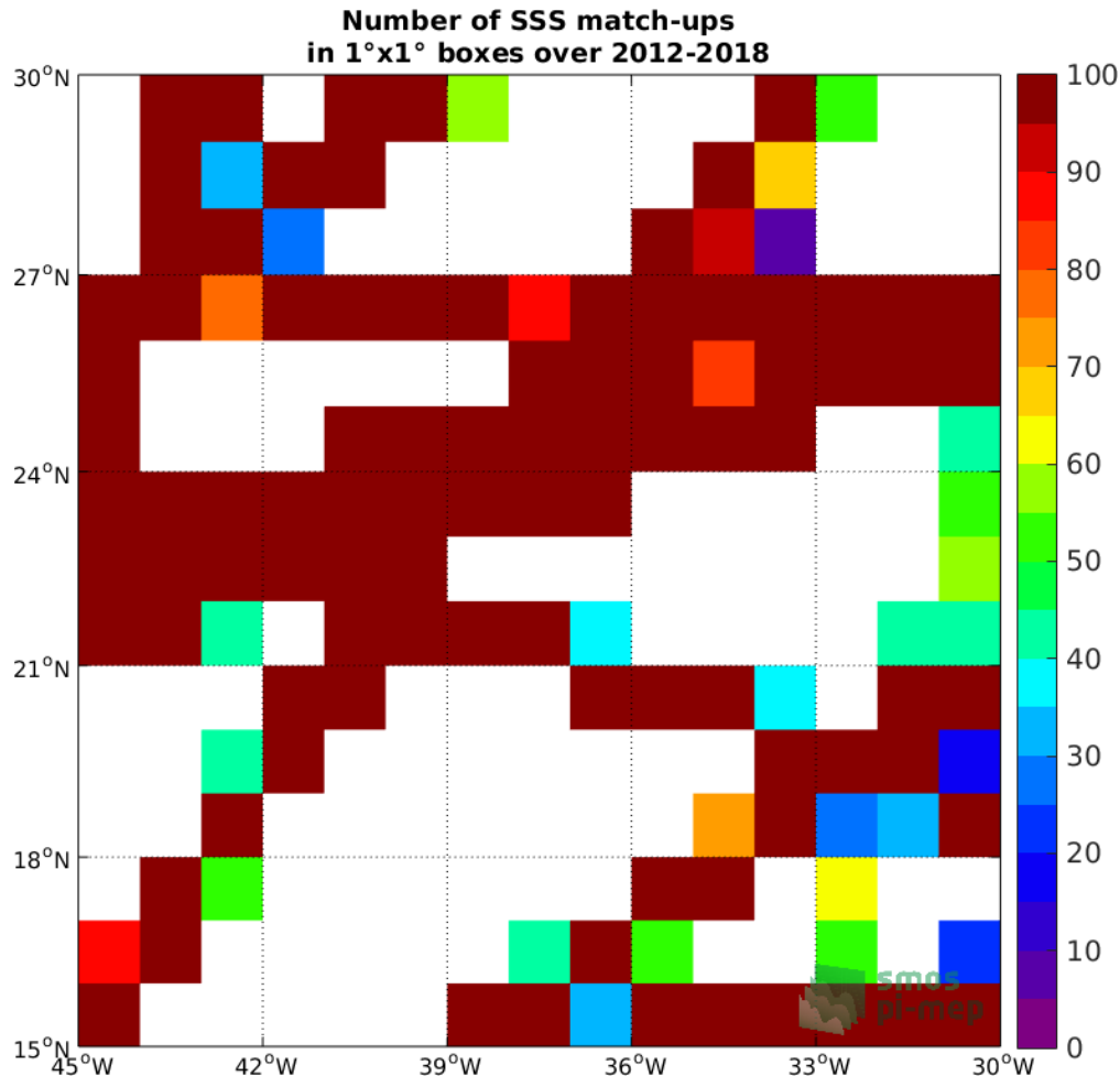
Figure 4: Number of SSS match-ups between TSG (GOSUD-Research-vessel) SSS and the SMAP SSS L4 OI v1 - 7 Days (IPRC) SSS product for the SPURS 1 Pi-MEP region over 1^\circ \times 1^\circ boxes and for the full satellite product period.
