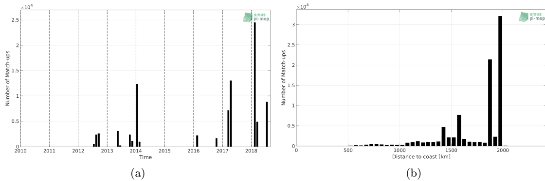
Figure 1: Number of match-ups between TSG (GOSUD-Research-vessel) and SMAP SSS L4 OI v1 - 7 Days (IPRC) SSS as a function of time (a) and as function of the distance to coast (b) over the SPURS 1 Pi-MEP region and for the full satellite product period.
