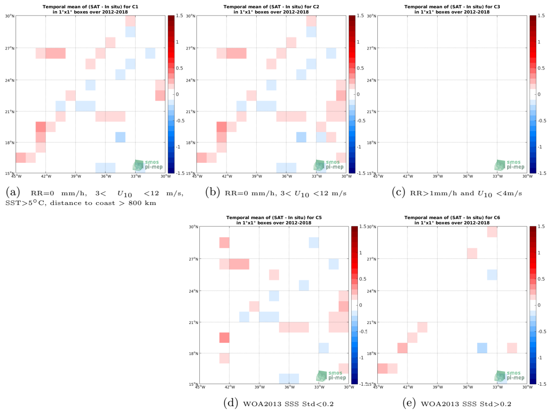
Figure 12: Temporal mean gridded over spatial boxes of size 1^\circ \times 1^\circ of \Delta\text{SSS} (SMAP SSS L4 OI v1 - 7 Days (IPRC) - TSG (GOSUD-Research-vessel)) for 5 different subdatasets corresponding to:RR=0 mm/h, 3 < U_{10} < 12 m/s, SST>5°C, distance to coast > 800 km (a), RR=0 mm/h, 3 < U_{10} < 12 m/s (b), RR>1mm/h and U_{10} < 4 m/s (c), WOA2013 SSS Std<0.2 (d), WOA2013 SSS Std>0.2 (e).
