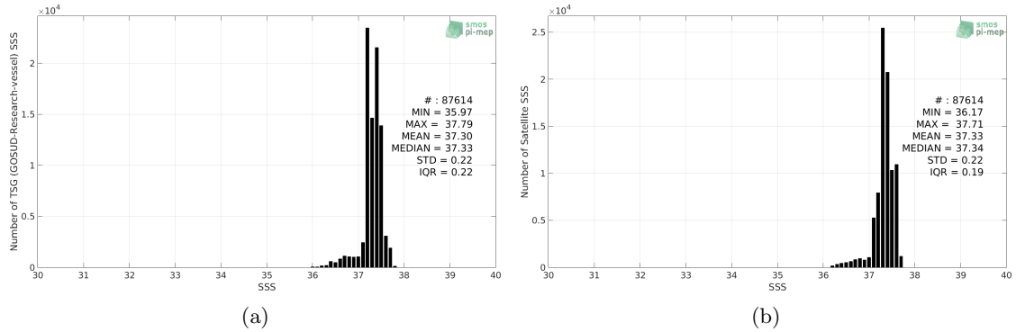
Figure 2: Histograms of SSS from TSG (GOSUD-Research-vessel) (a) and SMAP SSS L4 OI v1 - 7 Days (IPRC) (b) considering all match-up pairs per bins of 0.1 over the SPURS 1 Pi-MEP region and for the full satellite product period.
