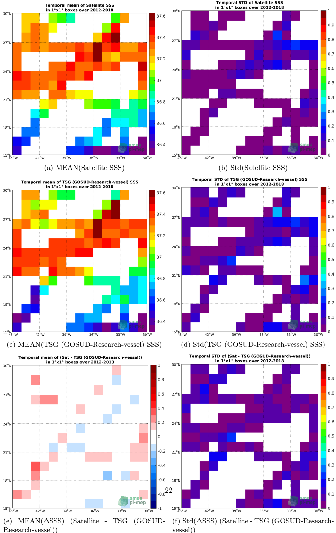
Figure 6: Temporal mean (left) and Std (right) of SSS from SMAP SSS L4 OI v1 - 7 Days (IPRC) (top), TSG (GOSUD-Research-vessel) (middle), and of \Delta SSS (Satellite - TSG (GOSUD-Research-vessel)). Only match-up pairs are used to generate these maps.
