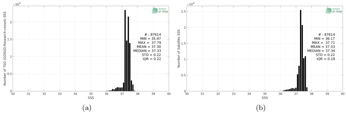
Figure 2: Histograms of SSS from TSG (GOSUD-Research-vessel) (a) and SMAP SSS L4 OI v1 - 7day (IPRC) (b) considering all match-up pairs per bins of 0.1 over the SPURS 1 Pi-MEP region and for the full satellite product period.
