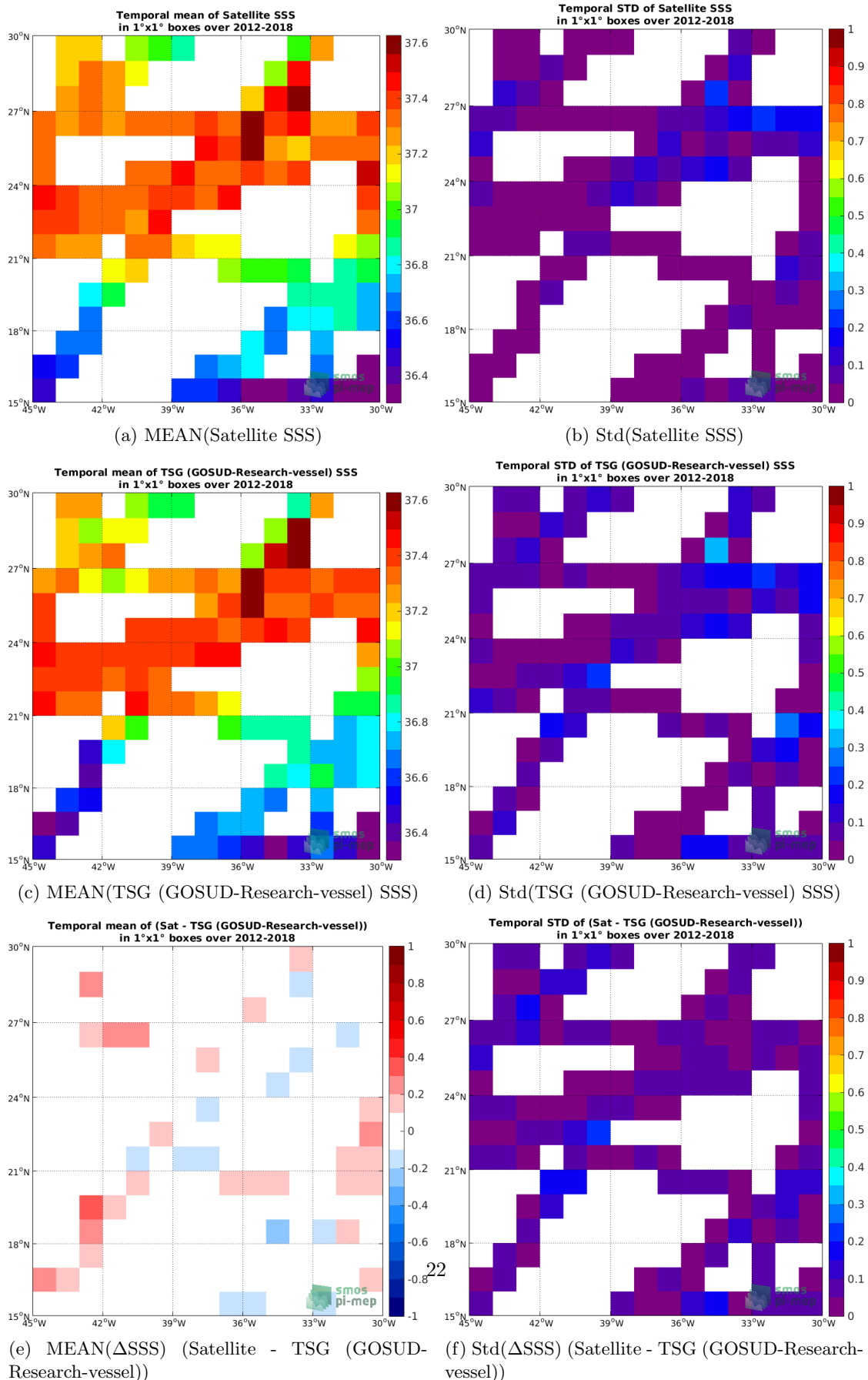
Figure 6: Temporal mean (left) and Std (right) of SSS from SMAP SSS L4 OI v1 - 7day (IPRC) (top), TSG (GOSUD-Research-vessel) (middle), and of \Delta SSS (Satellite - TSG (GOSUD-Research-vessel)). Only match-up pairs are used to generate these maps.
