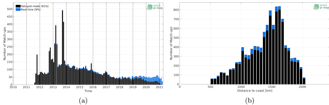
Figure 1: Number of match-ups between Argo and SMAP SSS L4 OI v1 - 7 Days (IPRC) SSS as a function of time (a) and as function of the distance to coast (b) over the SPURS 1 Pi-MEP region and for the full satellite product period.
