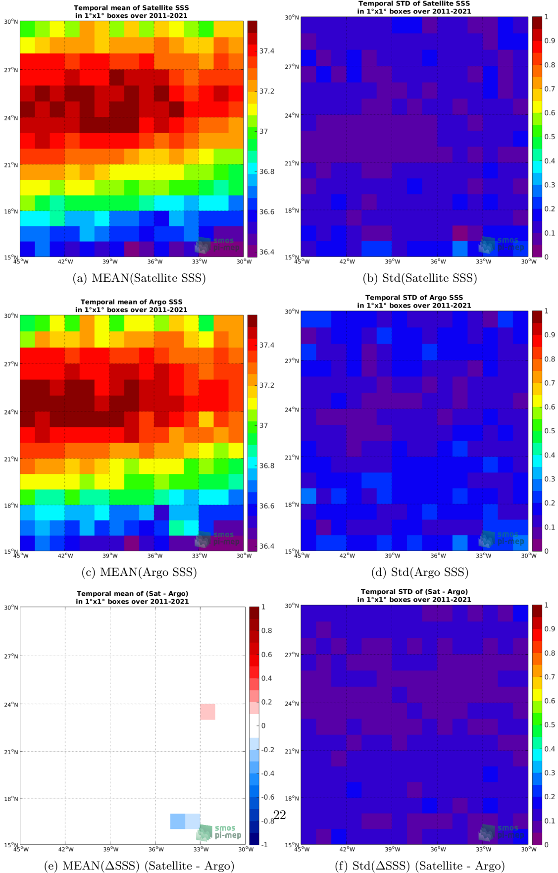
Figure 6: Temporal mean (left) and Std (right) of SSS from SMAP SSS L4 OI v1 - 7 Days (IPRC) (top), Argo (middle), and of \Delta SSS (Satellite - Argo). Only match-up pairs are used to generate these maps.
