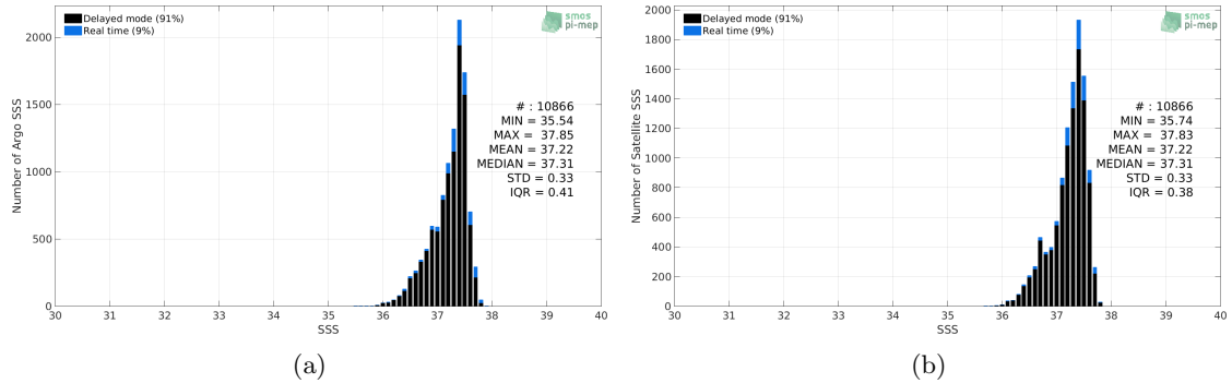
Figure 2: Histograms of SSS from Argo (a) and SMAP SSS L4 OI v1 - 7 Days (IPRC) (b) considering all match-up pairs per bins of 0.1 over the SPURS 1 Pi-MEP region and for the full satellite product period.
