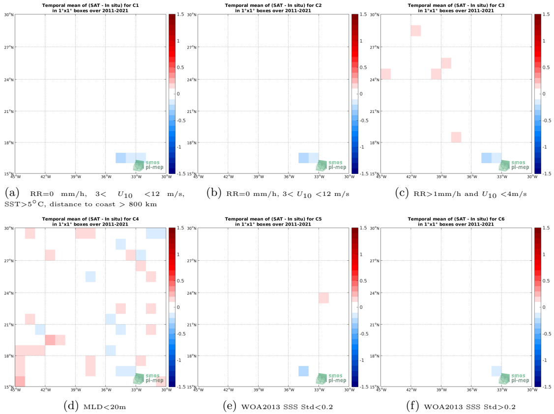
Figure 12: Temporal mean gridded over spatial boxes of size 1^\circ \times 1^\circ of \Delta SSS (SMAP SSS L4 OI v1 - 7 Days (IPRC) - Argo) for 6 different subdatasets corresponding to:RR=0 mm/h, 3 < U_{10} < 12 m/s, SST>5°C, distance to coast > 800 km (a), RR=0 mm/h, 3 < U_{10} < 12 m/s (b), RR>1mm/h and U_{10} < 4 m/s (c),MLD<20m (d),WOA2013 SSS Std<0.2 (e),WOA2013 SSS Std>0.2 (f).
