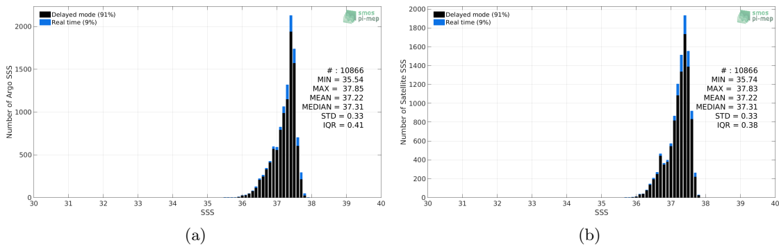
Figure 2: Histograms of SSS from Argo (a) and SMAP SSS L4 OI v1 - 7day (IPRC) (b) considering all match-up pairs per bins of 0.1 over the SPURS 1 Pi-MEP region and for the full satellite product period.
