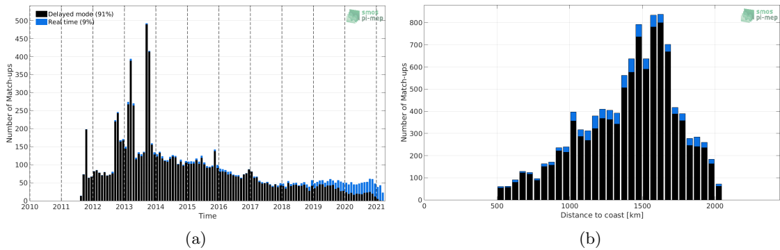
Figure 1: Number of match-ups between Argo and SMAP SSS L4 OI v1 - 7day (IPRC) SSS as a function of time (a) and as function of the distance to coast (b) over the SPURS 1 Pi-MEP region and for the full satellite product period.
