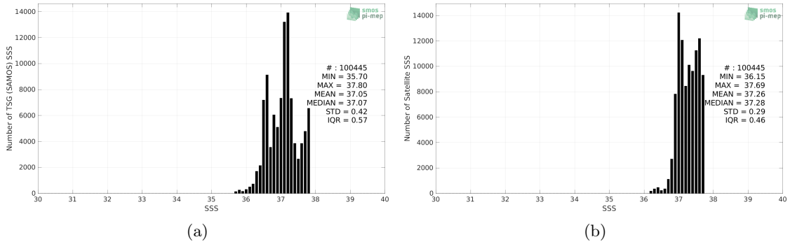
Figure 2: Histograms of SSS from TSG (SAMOS) (a) and SMAP SSS L4 OI v1 - Monthly (IPRC) (b) considering all match-up pairs per bins of 0.1 over the SPURS 1 Pi-MEP region and for the full satellite product period.
