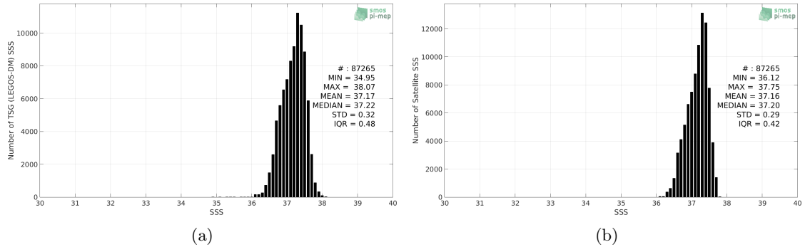
Figure 2: Histograms of SSS from TSG (LEGOS-DM) (a) and SMAP SSS L4 OI v1 - Monthly (IPRC) (b) considering all match-up pairs per bins of 0.1 over the SPURS 1 Pi-MEP region and for the full satellite product period.
