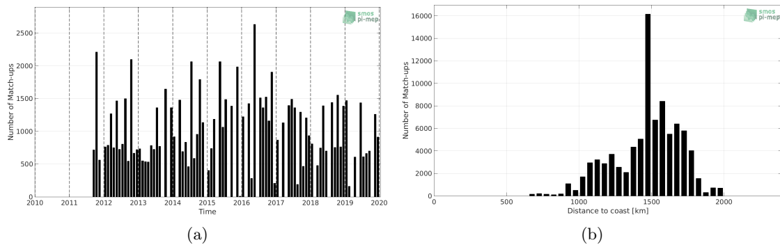
Figure 1: Number of match-ups between TSG (LEGOS-DM) and SMAP SSS L4 OI v1 - Monthly (IPRC) SSS as a function of time (a) and as function of the distance to coast (b) over the SPURS 1 Pi-MEP region and for the full satellite product period.
