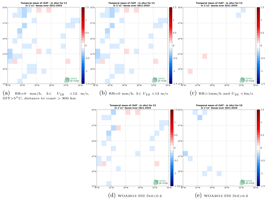
Figure 12: Temporal mean gridded over spatial boxes of size 1^\circ \times 1^\circ of \Delta SSS (SMAP SSS L4 OI v1 - Monthly (IPRC) - TSG (LEGOS-DM)) for 5 different subdatasets corresponding to:RR=0 mm/h, 3 < U_{10} < 12 m/s, SST >5^\circ C, distance to coast > 800 km (a), RR=0 mm/h, 3 < U_{10} < 12 m/s (b), RR >1 mm/h and U_{10} < 4 m/s (c), WOA2013 SSS Std <0.2 (d), WOA2013 SSS Std >0.2 (e).
