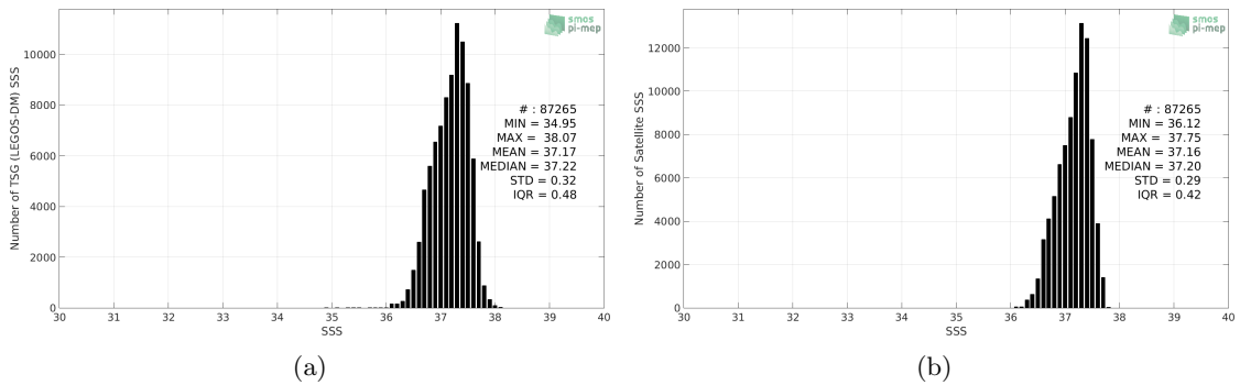
Figure 2: Histograms of SSS from TSG (LEGOS-DM) (a) and SMAP SSS L4 OI v1 - Monthly (IPRC) (b) considering all match-up pairs per bins of 0.1 over the SPURS 1 Pi-MEP region and for the full satellite product period.
