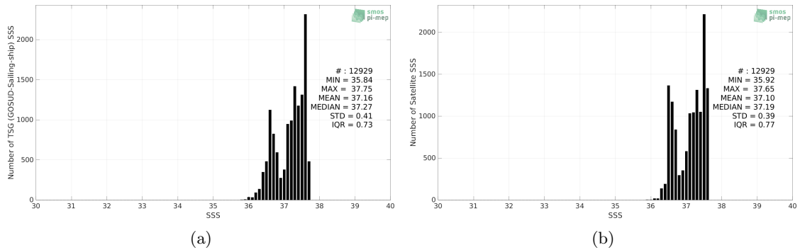
Figure 2: Histograms of SSS from TSG (GOSUD-Sailing-ship) (a) and SMAP SSS L4 OI v1 - Monthly (IPRC) (b) considering all match-up pairs per bins of 0.1 over the SPURS 1 Pi-MEP region and for the full satellite product period.
